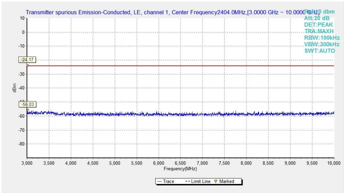
Fig.6. Transmitter Spurious Emission -Conducted: GFSK, 2404 MHz,3GHz - 10GHz
