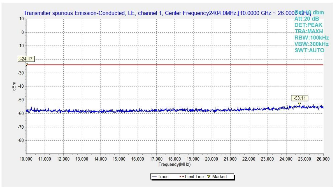
Fig.7. Transmitter Spurious Emission -Conducted: GFSK, 2404MHz,10GHz - 26GHz
