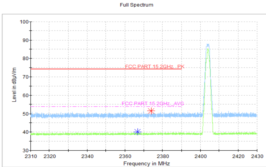
Fig.18. Frequency Band Edges: GFSK, 2404 MHz, Hopping Off, 2.31 GHz – 2.43GHz
