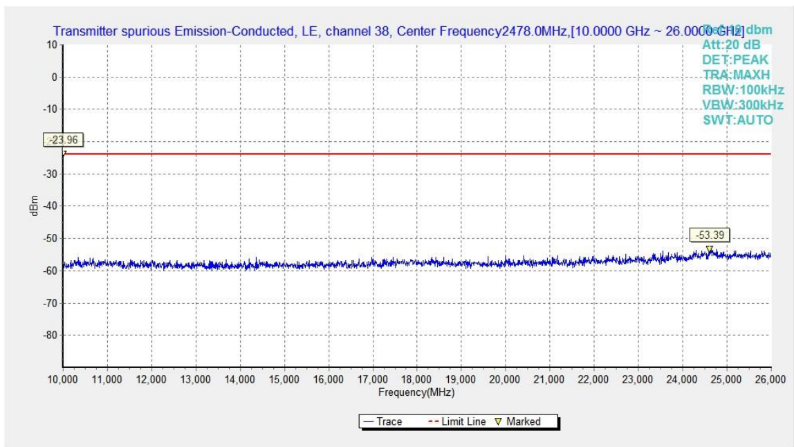
Fig.17. Transmitter Spurious Emission -Conducted: GFSK, 2478 MHz, 10GHz - 26GHz
