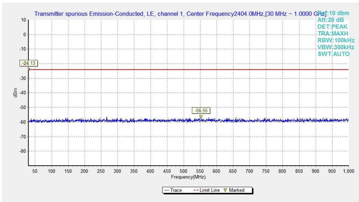
Fig.4. Transmitter Spurious Emission -Conducted: GFSK, 2404 MHz, 30MHz - 1GHz
