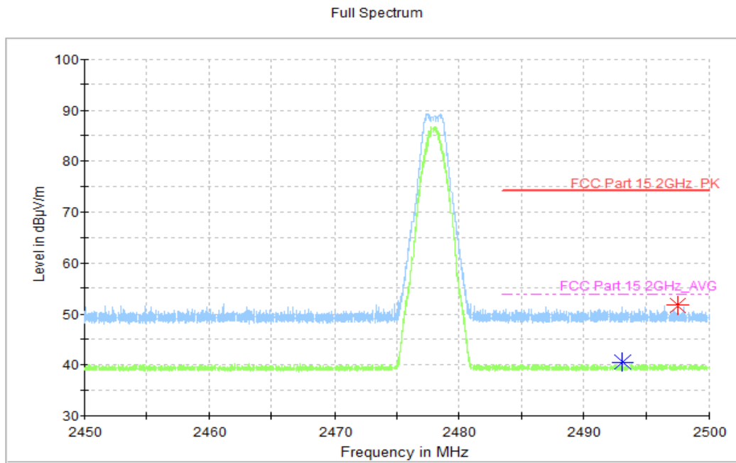
Fig.19. Frequency Band Edges: GFSK, 2478 MHz, Hopping Off, 2.45 GHz - 2.50GHz
