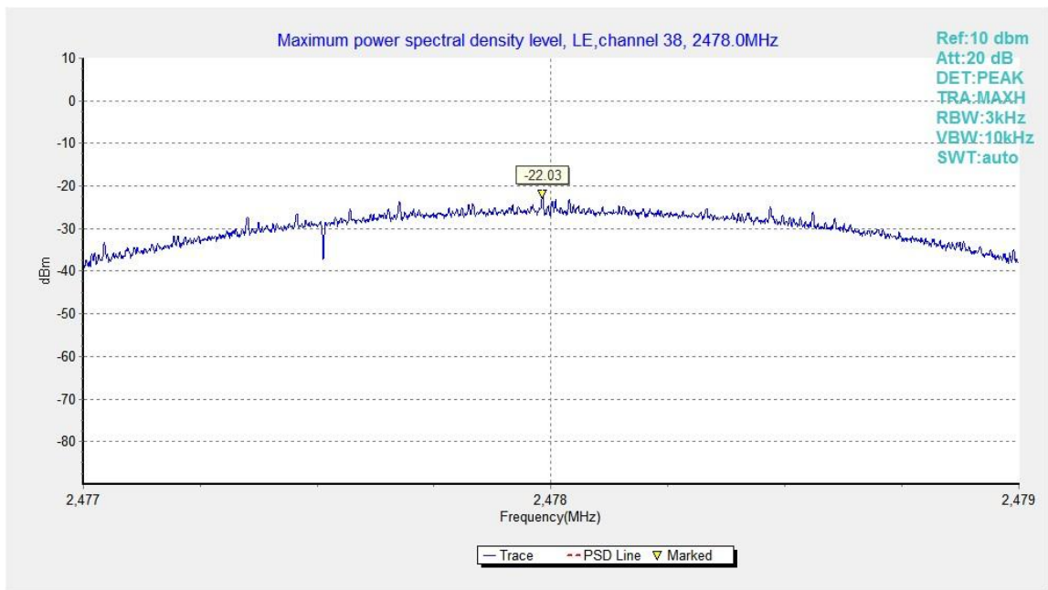
Fig.25. Maximum Power Spectral Density Level Function: GFSK, 2478 MHz
