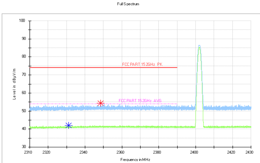
Fig.18. Frequency Band Edges: GFSK, 2402 MHz, Hopping Off, 2.31 GHz – 2.43GHz
