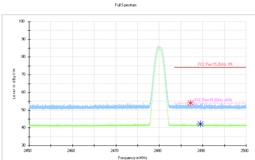
Fig.19. Frequency Band Edges: GFSK, 2480 MHz, Hopping Off, 2.45 GHz - 2.50GHz
