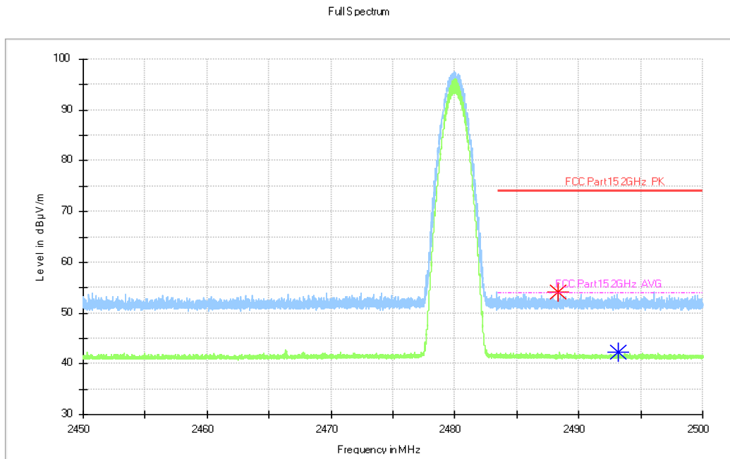
Fig.63. Frequency Band Edges: 8DPSK, Channel 78, 2.45 GHz - 2.50GHz
