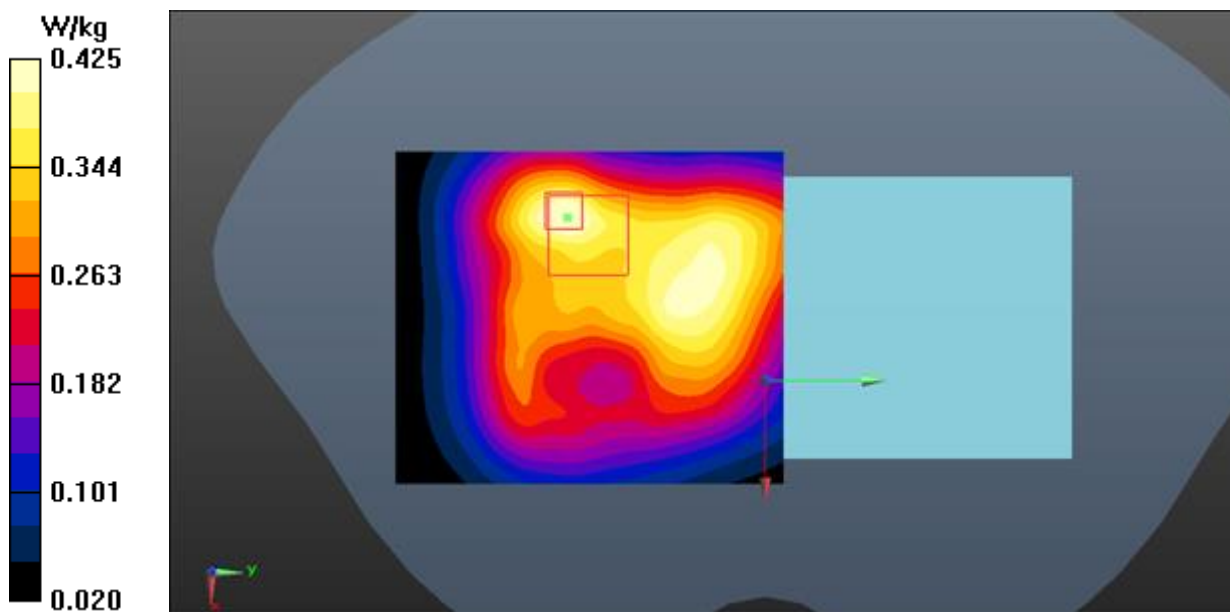
Fig.4 GSM 1900 Body
