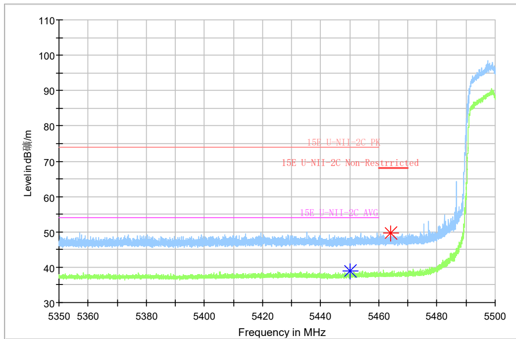
Fig.48 Band Edges (802.11ac-HT20 Ch100, 5500MHz)
