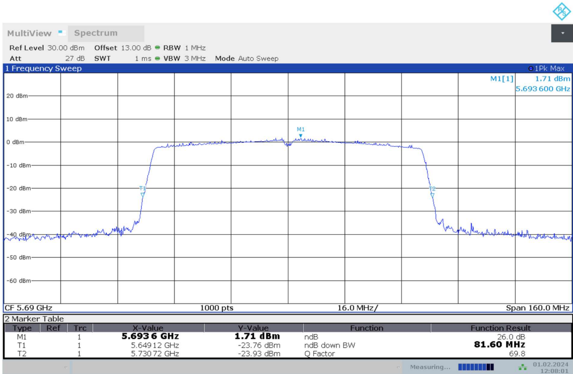
Fig.33 26dB Emission Bandwidth (802. 11ac-VHT80, 5690MHz)
