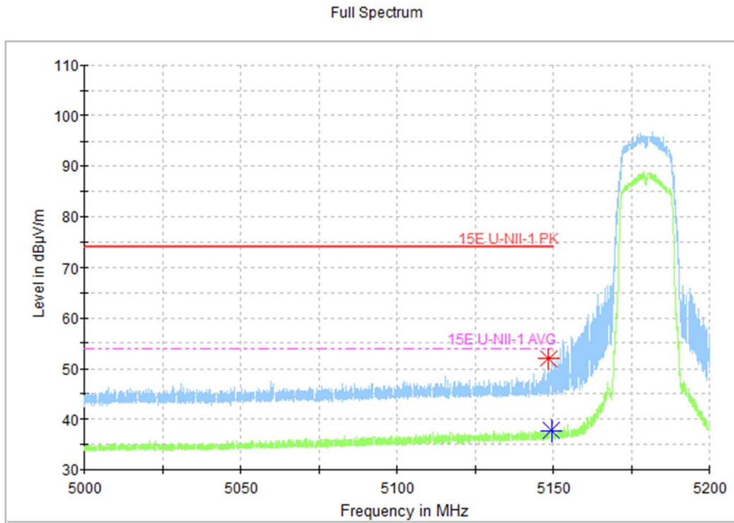
Fig.34 Band Edges (802.11a Ch36, 5180MHz)
