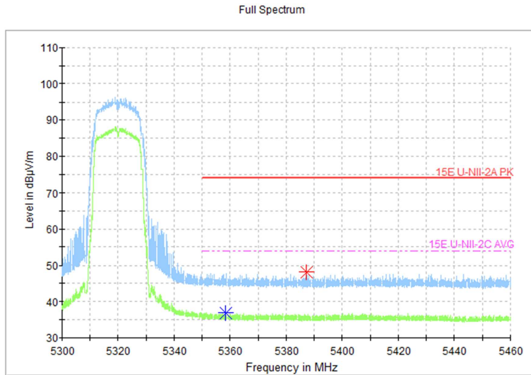
Fig.35 Band Edges (802.11a Ch64, 5320MHz)
