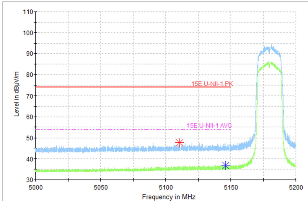
Fig.38 Band Edges (802.11n-HT20 Ch36, 5180MHz)
