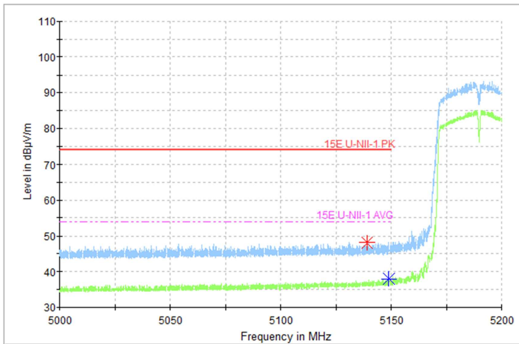
Fig.50 Band Edges (802.11ac-HT40 Ch38, 5190MHz)
