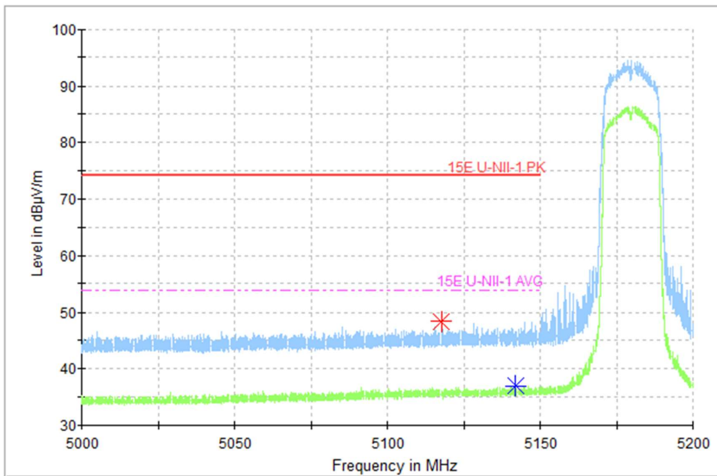
Fig.46 Band Edges (802.11ac-HT20 Ch36, 5180MHz)
