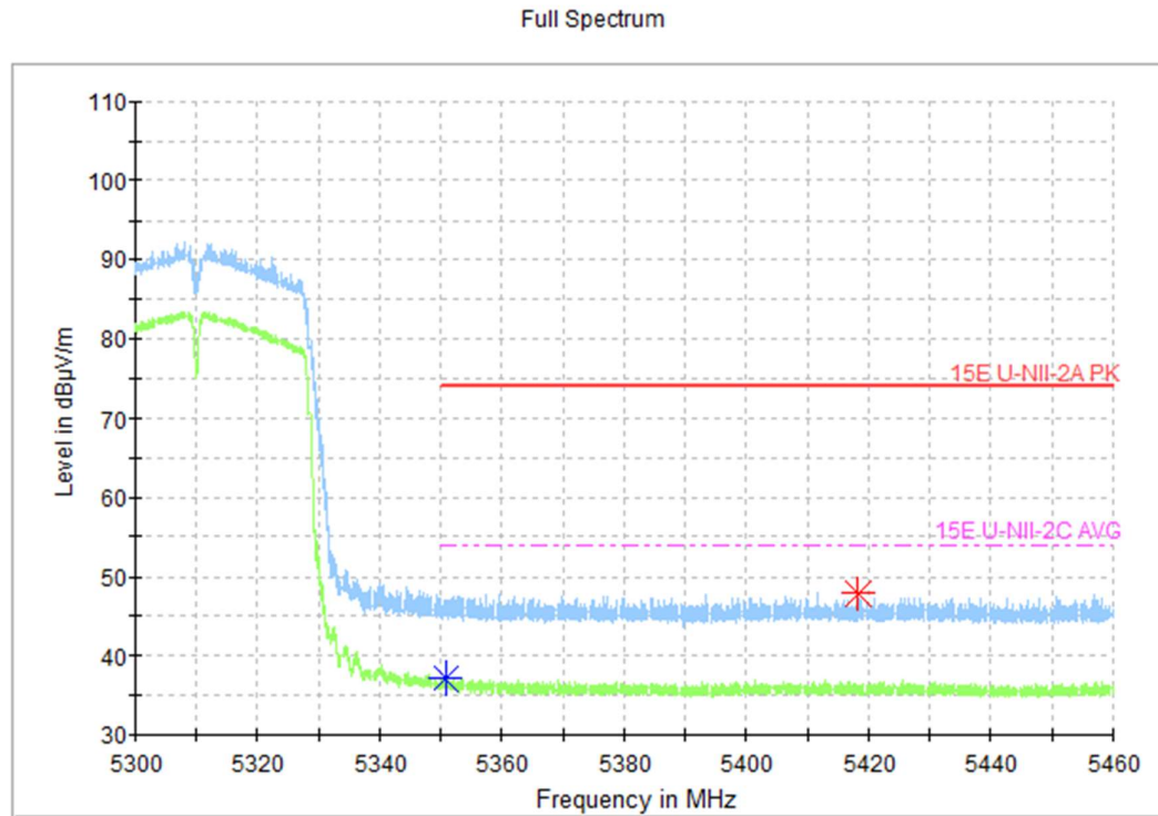
Fig.43 Band Edges (802.11n-HT40 Ch62, 5310MHz)
