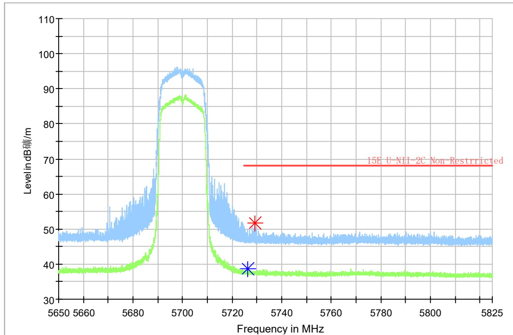
Fig.49 Band Edges (802.11ac-HT20 Ch140, 5700MHz)
