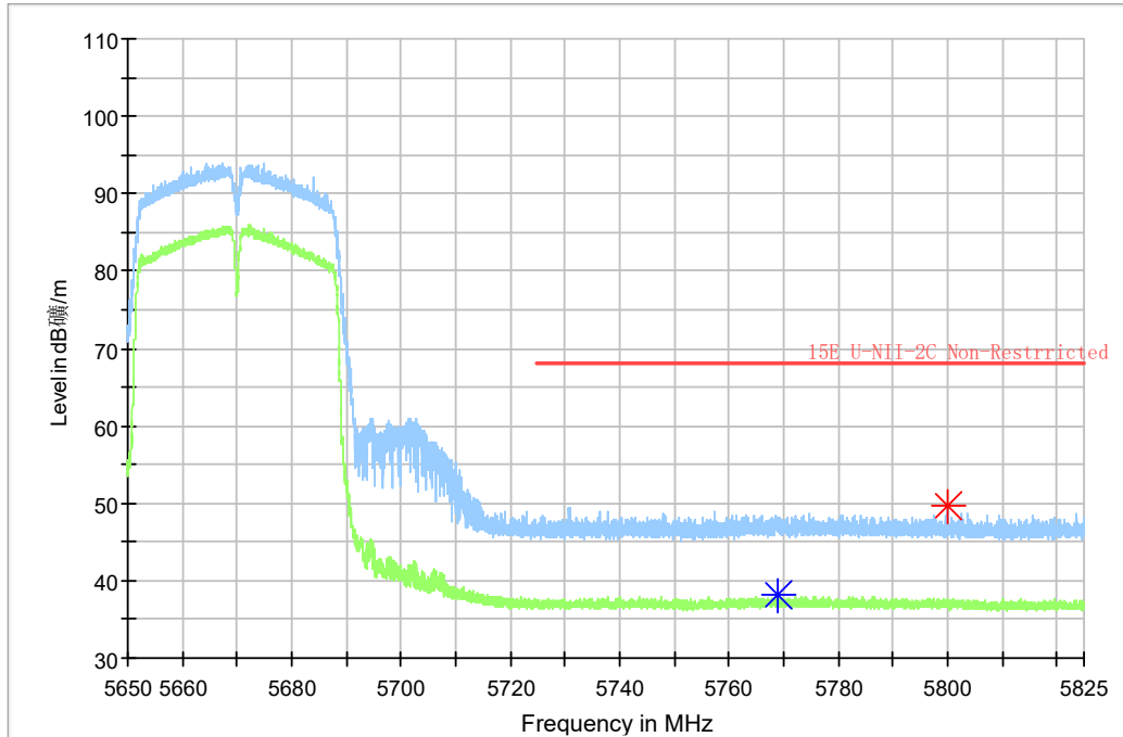
Fig.45 Band Edges (802.11n-HT40 Ch134, 5670MHz)
