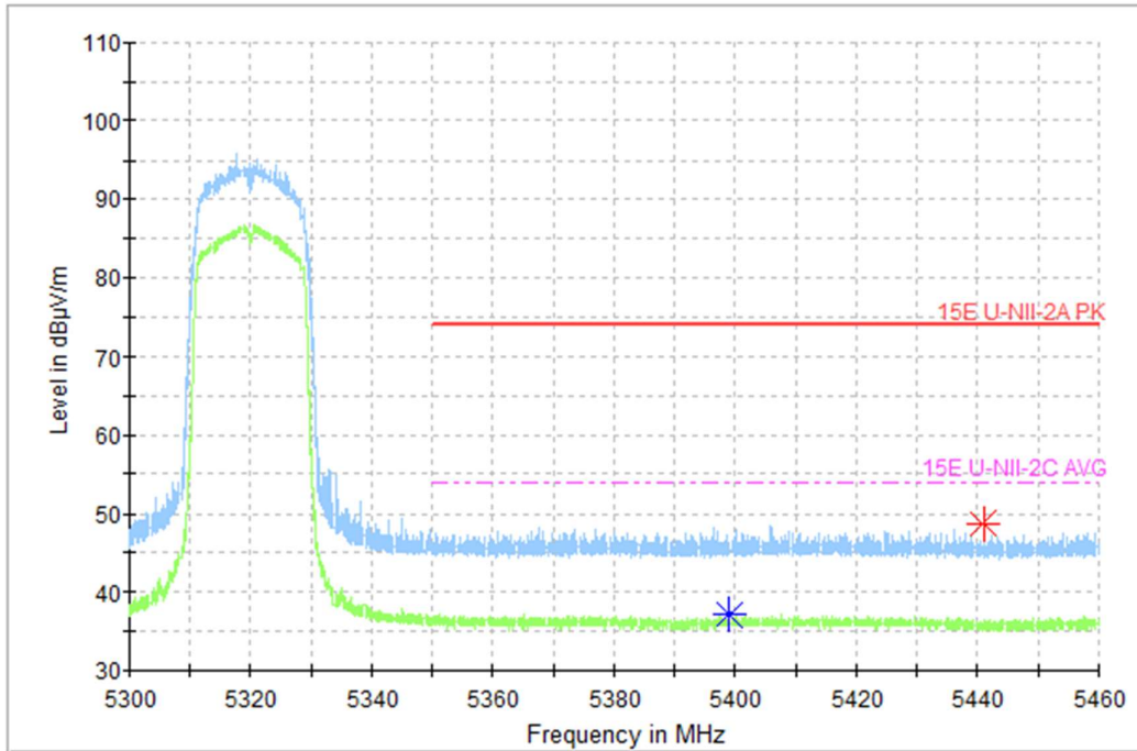
Fig.47 Band Edges (802.11ac-HT20 Ch64, 5320MHz)
