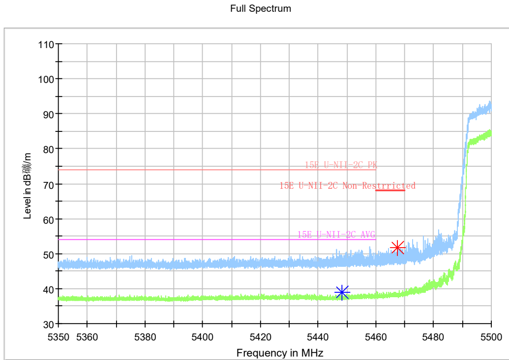
Fig.44 Band Edges (802.11n-HT40 Ch102, 5510MHz)
