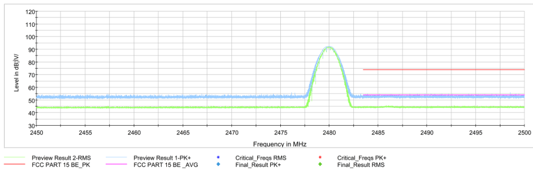
Fig.61. Frequency Band Edges: \pi/4 DQPSK, Channel 78, Hopping Off, 2.45 GHz - 2.50GHz
