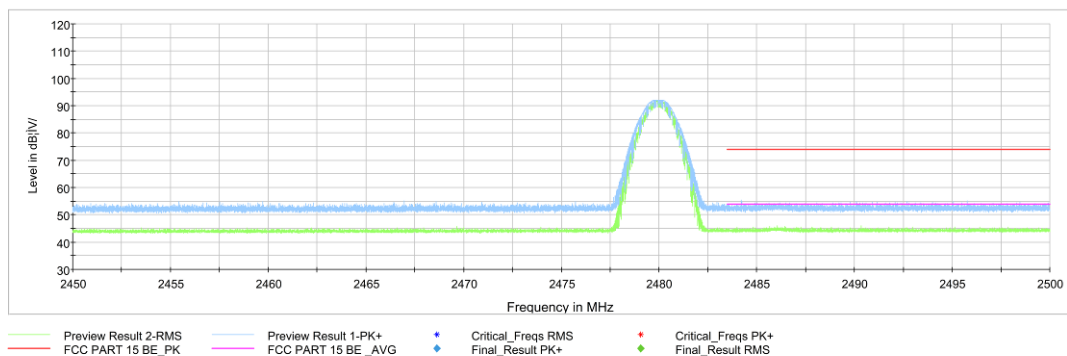
Fig.63. Frequency Band Edges: 8DPSK, Channel 78, 2.45 GHz - 2.50GHz
