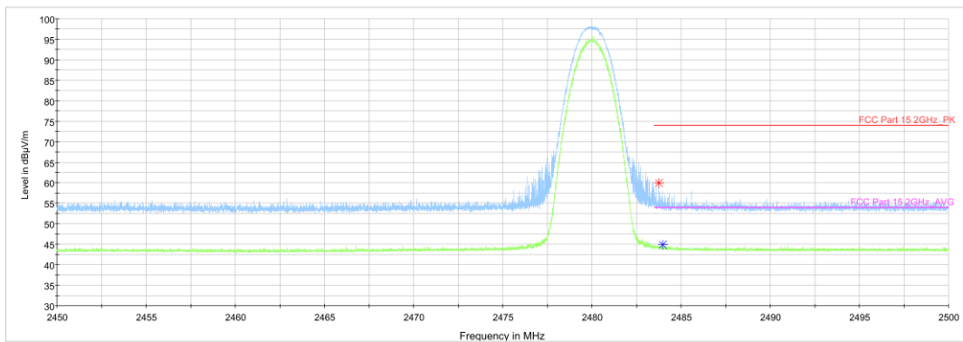
Fig.61. Frequency Band Edges: \pi/4 DQPSK, Channel 78, Hopping Off, 2.45 GHz - 2.50GHz
