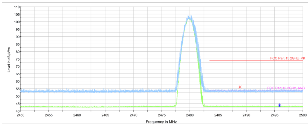
Fig.70. Frequency Band Edges: \pi/4 DQPSK, Channel 78, Hopping Off, 2.45 GHz - 2.50GHz
