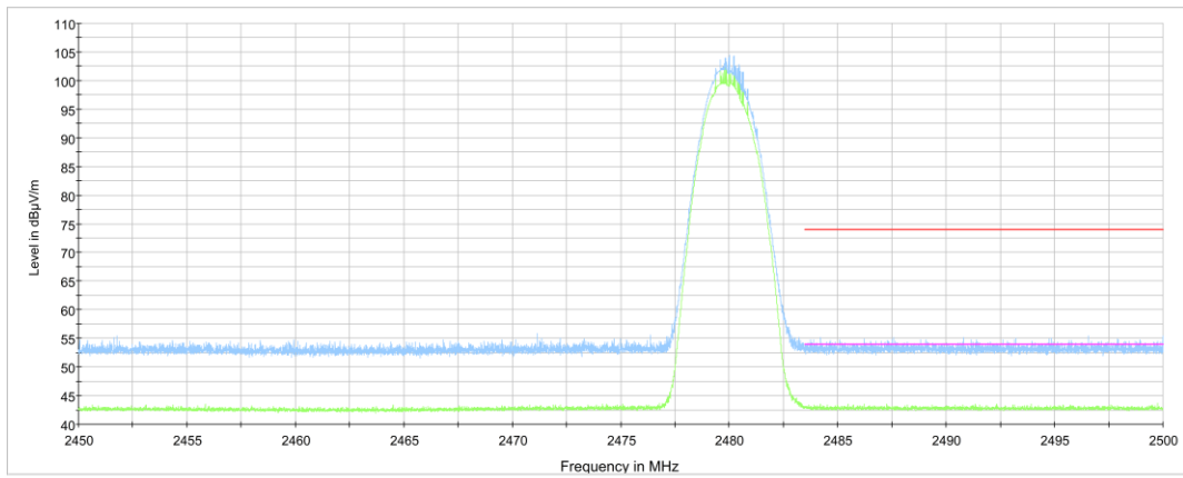
Fig.72. Frequency Band Edges: 8DPSK, Channel 78, 2.45 GHz - 2.50GHz
