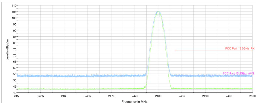
Fig.68. Frequency Band Edges: GFSK, Channel 78, Hopping Off, ch11, 2.45 GHz - 2.50GHz
