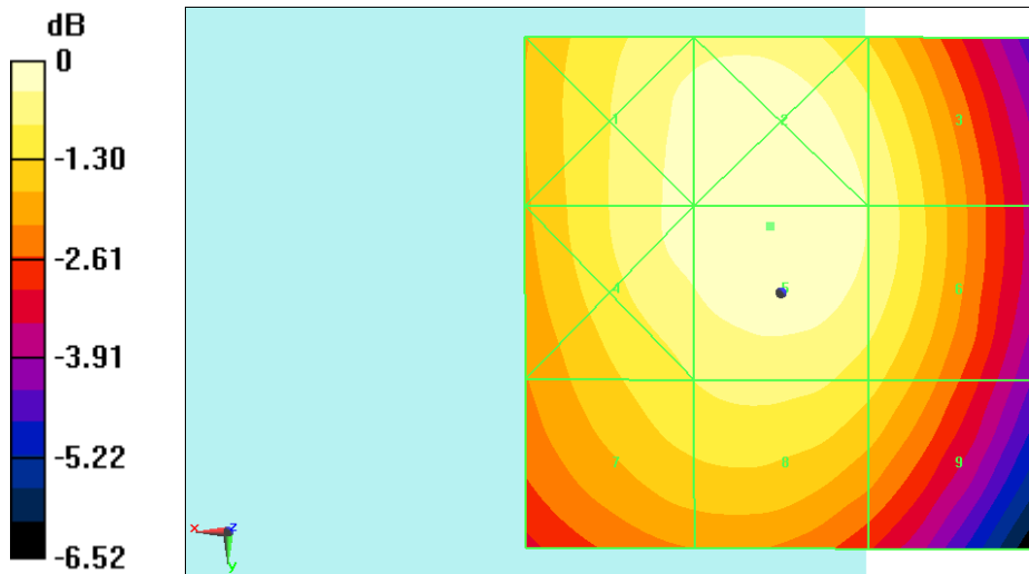
Fig B.1 HAC RF E-Field GSM 850
