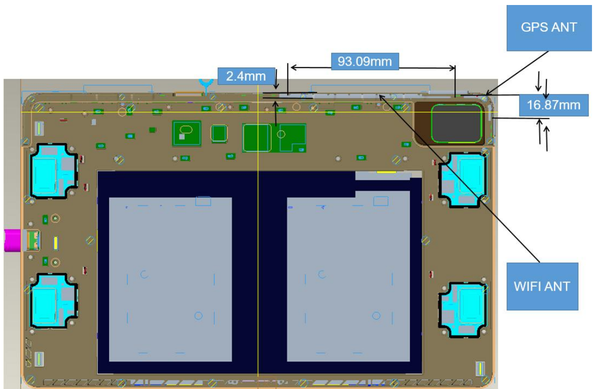
Picture 23 Antenna Locations
