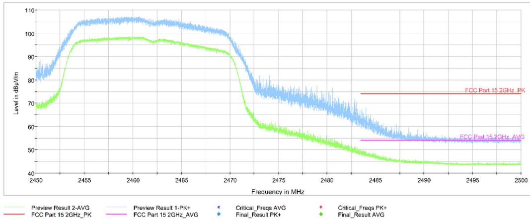
Fig.A.6.1.4 Transmitter Spurious Emission - Radiated (Power): 802.11g, ch11, 2.45 GHz - 2.50GHz
