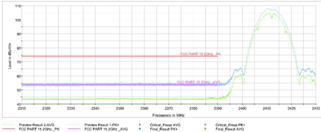
Fig.A.6.1.1 Transmitter Spurious Emission - Radiated (Power): 802.11b, ch1, 2.31 GHz – 2.43GHz
