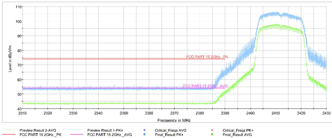
Fig.A.6.1.5 Transmitter Spurious Emission - Radiated (Power): 802.11n-HT20, ch1, 2.31 GHz - 2.43GHz
