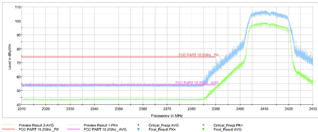
Fig.A.6.1.3 Transmitter Spurious Emission - Radiated (Power): 802.11g, ch1, 2.31 GHz - 2.43GHz
