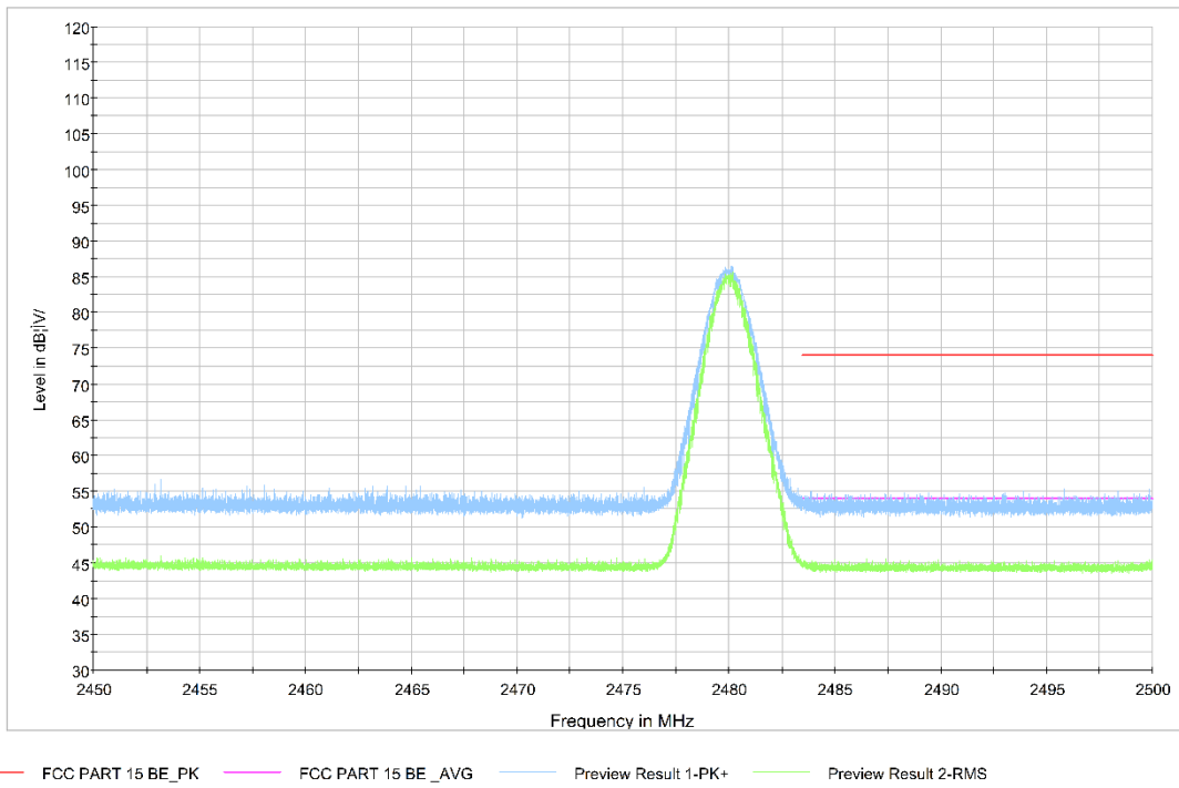
Fig.18. Frequency Band Edges: 8DPSK, Channel 78, 2.45 GHz - 2.50GHz
