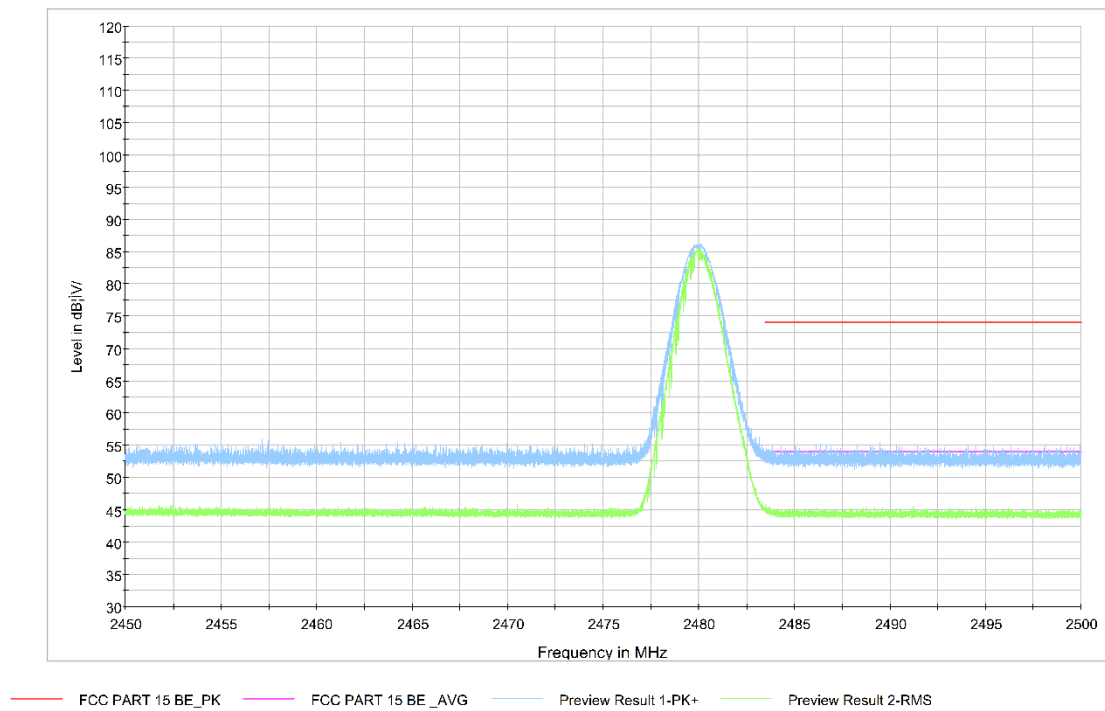
Fig.16. Frequency Band Edges: \pi/4 DQPSK, Channel 78, Hopping Off, 2.45 GHz - 2.50GHz
