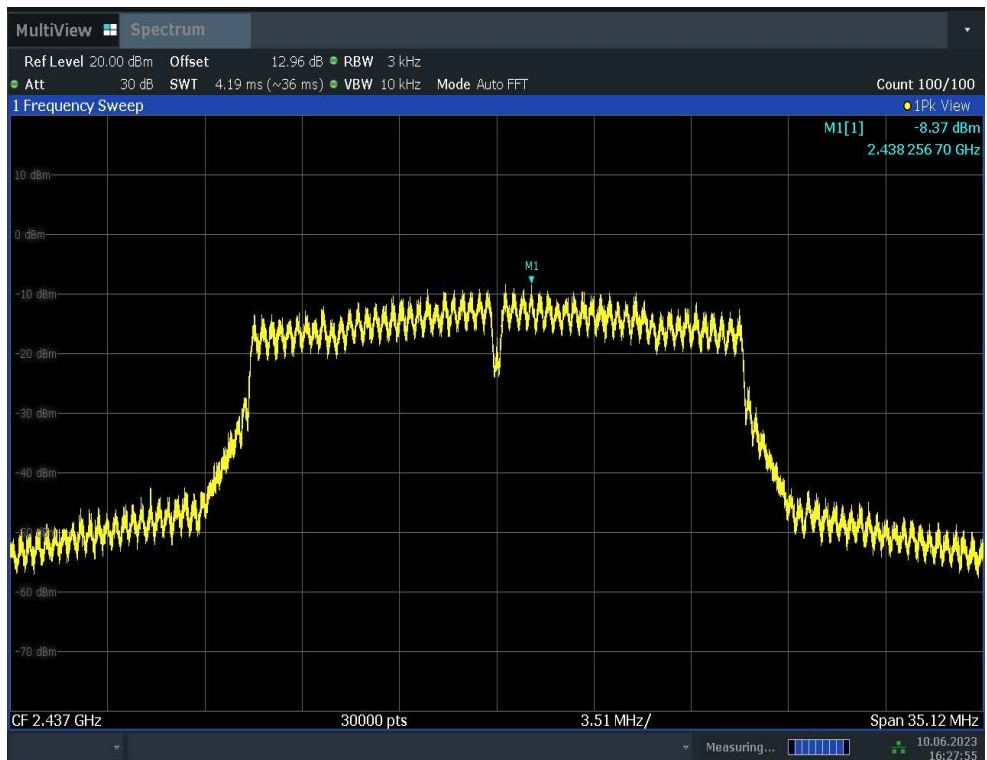
Fig.A.3.8 Power Spectral Density (802.11n-HT20, Ch 6)
