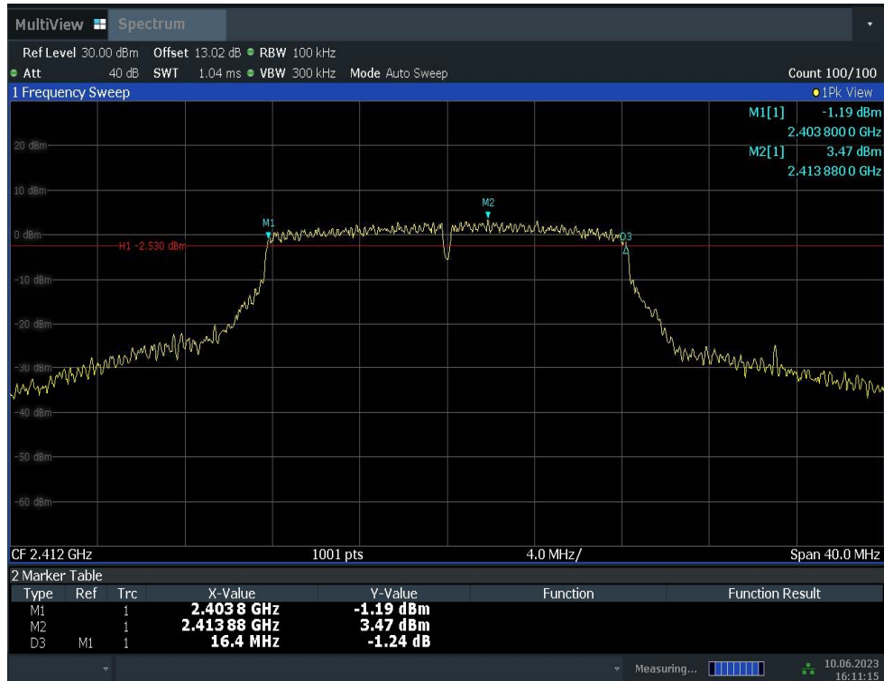
Fig.A.4.4 Occupied 6dB Bandwidth (802.11g, Ch 1)
