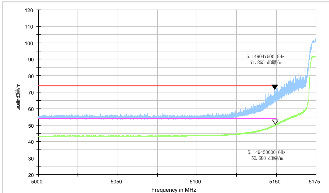
Fig.27 Band Edges (802.11n-HT40 Ch38, 5190MHz)
