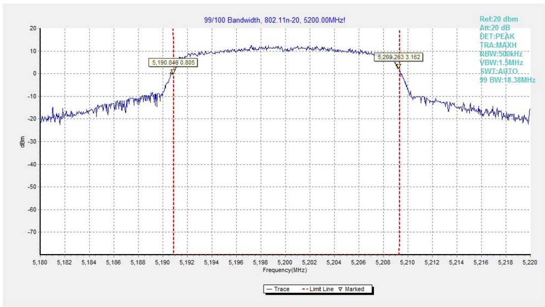
Fig.47 99% Occupied bandwidth (802.11n-HT20, 5200MHz)
