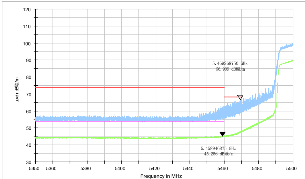
Fig.37 Band Edges (802.11ac-HT40 Ch102, 5510MHz)
