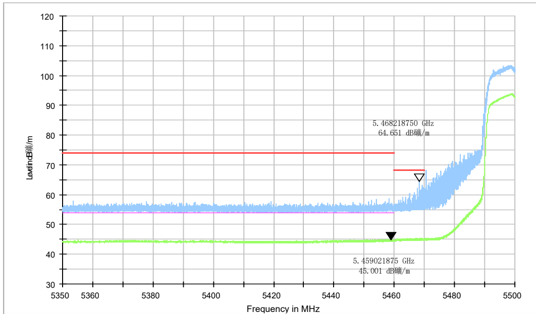
Fig.33 Band Edges (802.11ac-HT20 Ch100, 5500MHz)
