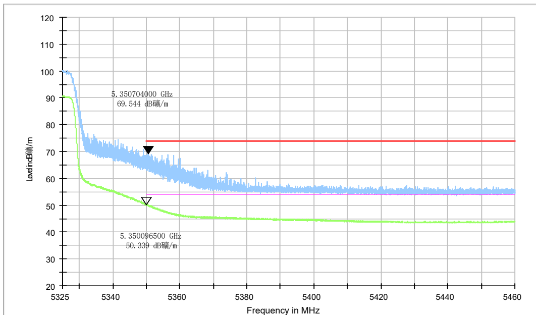
Fig.28 Band Edges (802.11n-HT40 Ch62, 5310MHz)
