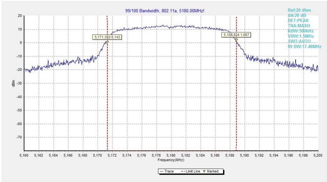
Fig.43 99% Occupied bandwidth (802.11a, 5180MHz)
