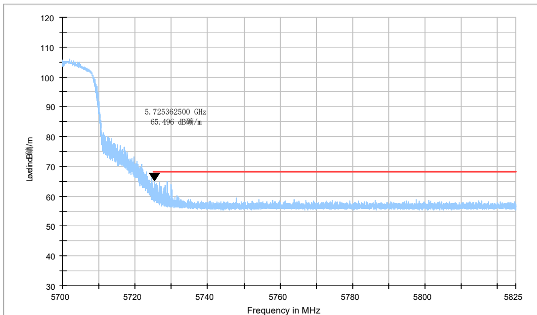
Fig.34 Band Edges (802.11ac-HT20 Ch140, 5700MHz)
