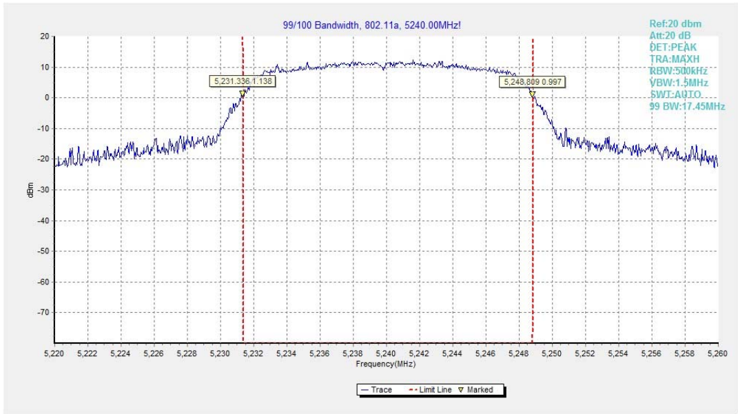
Fig.45 99% Occupied bandwidth (802.11a, 5240MHz)
