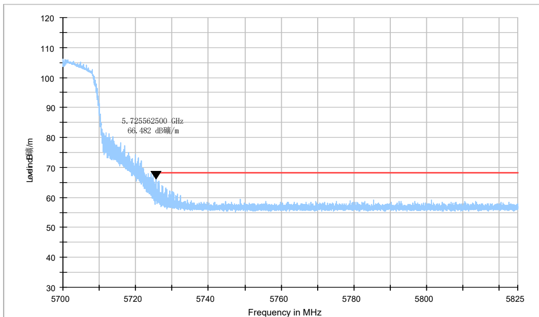
Fig.26 Band Edges (802.11n-HT20 Ch140, 5700MHz)
