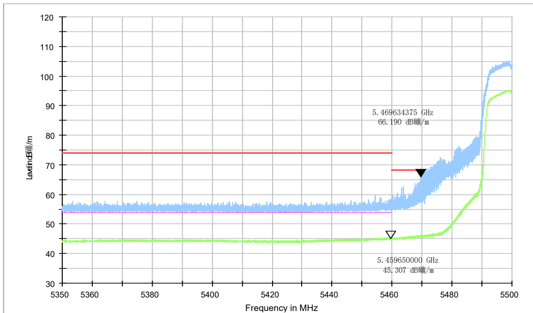
Fig.21 Band Edges (802.11a Ch100, 5500MHz)
