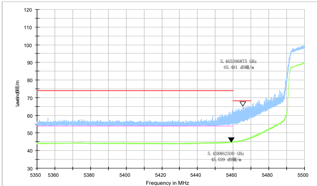
Fig.29 Band Edges (802.11n-HT40 Ch102, 5510MHz)
