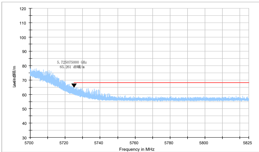
Fig.38 Band Edges (802.11ac-HT40 Ch134, 5670MHz)
