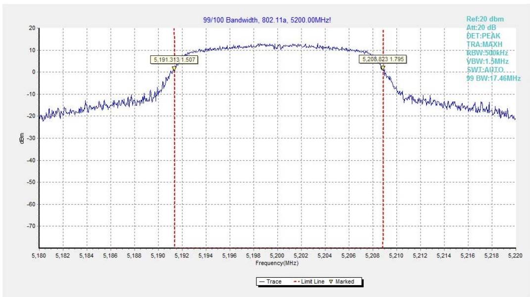
Fig.44 99% Occupied bandwidth (802.11a, 5200MHz)
