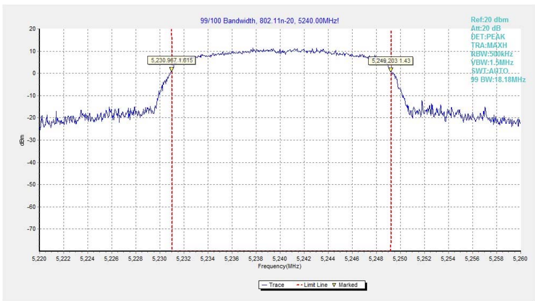
Fig.48 99% Occupied bandwidth (802.11n-HT20, 5240MHz)
