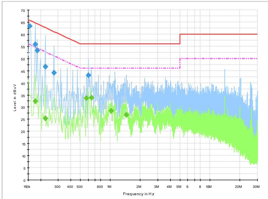
Fig.B.9.1 AC Powerline Conducted Emission- bluetooth
