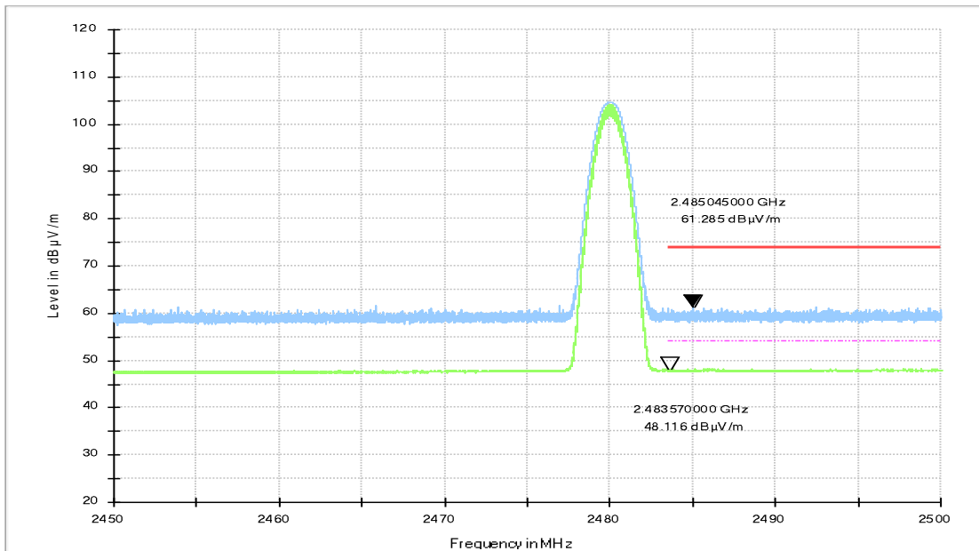
Fig.14. Frequency Band Edges: GFSK, Channel 78, 2.45 GHz - 2.50GHz
