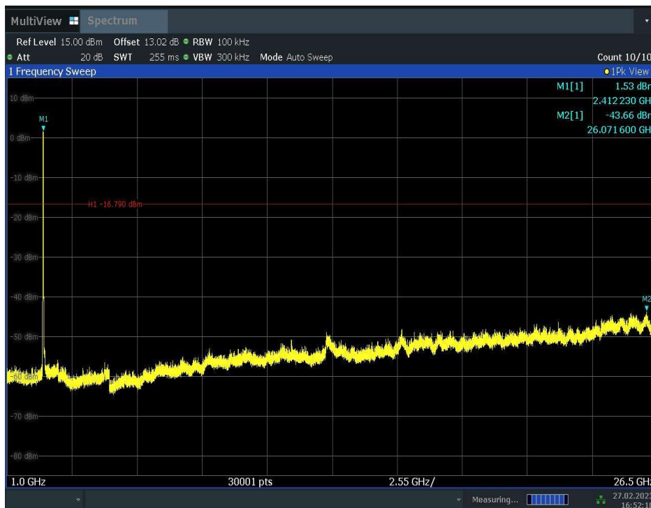
Fig.A.6.1.12 Transmitter Spurious Emission - Conducted (802.11g, Ch1, 1 GHz-26.5 GHz)
