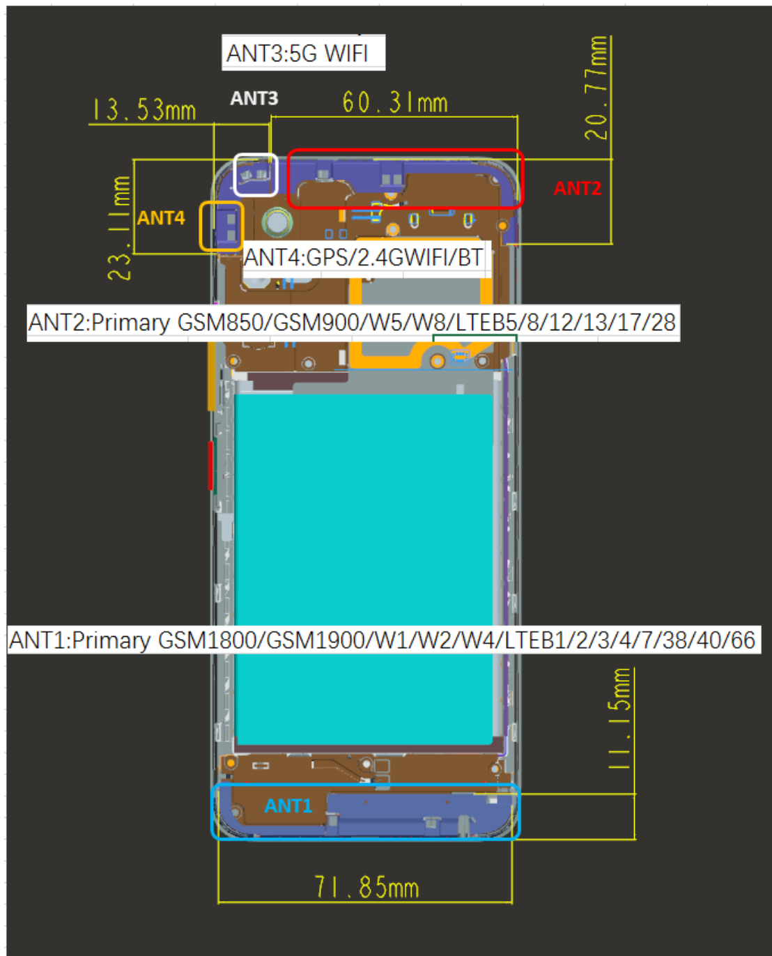
Picture 12 Antenna Locations
