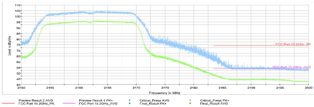
Fig.A.6.2.10 Transmitter Spurious Emission - Radiated (Power): 802.11g, ch11, 2.45 GHz - 2.50GHz
