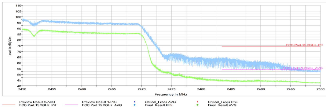
Fig.A.6.2.11 Transmitter Spurious Emission - Radiated (Power): 802.11n-HT40, ch9, 2.45 GHz - 2.50GHz
