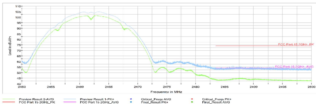
Fig.A.6.2.9 Transmitter Spurious Emission - Radiated (Power): 802.11b, ch11, 2.45 GHz - 2.50GHz
