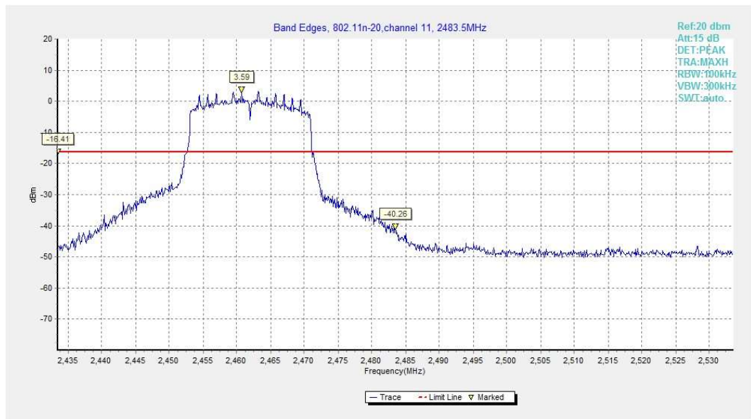
Fig.A.5.6 Band Edges (802.11n-HT20, Ch 11)
