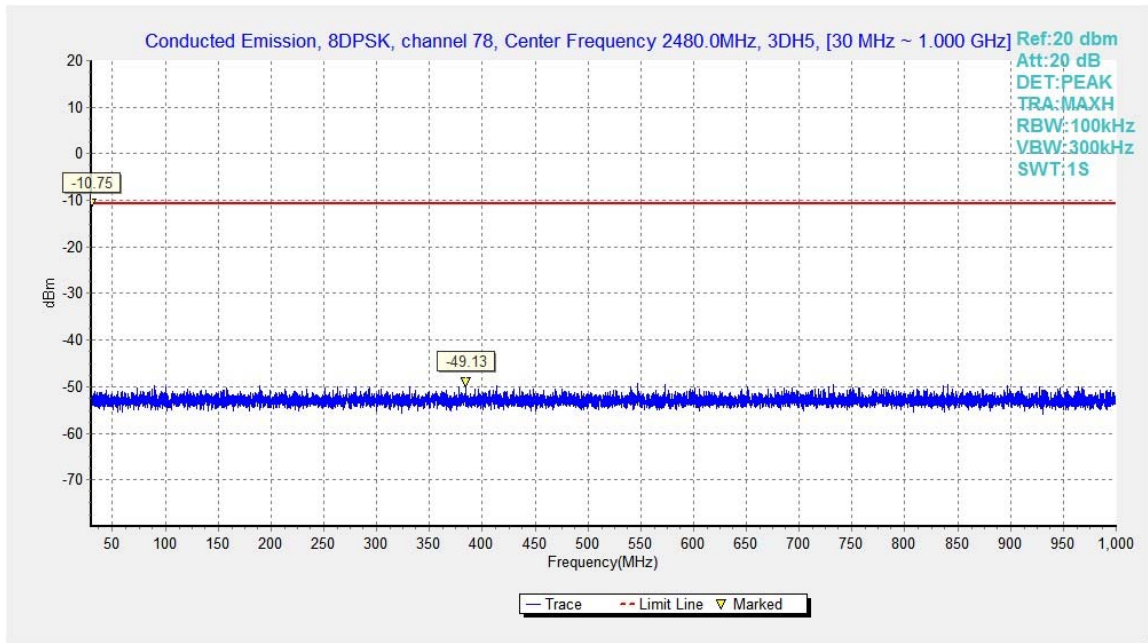
Fig.61. Conducted spurious emission: 8DPSK, Channel 78, 30MHz - 1GHz
