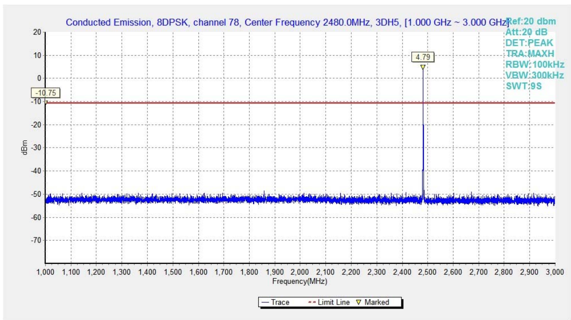
Fig.62. Conducted spurious emission: 8DPSK, Channel 78, 1GHz - 3GHz
