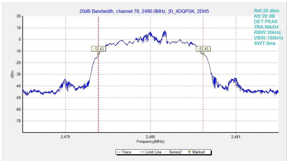
Fig.88. 20dB Bandwidth: \pi/4 DQPSK, Channel 78
