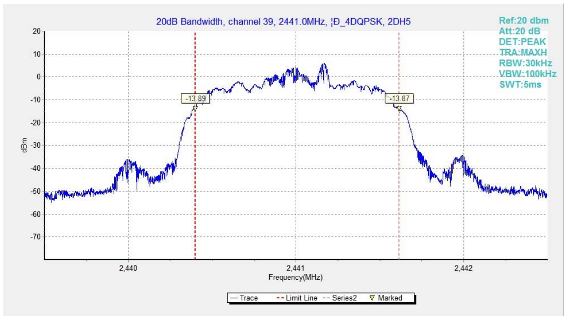
Fig.87. 20dB Bandwidth: \pi/4 DQPSK, Channel 39
