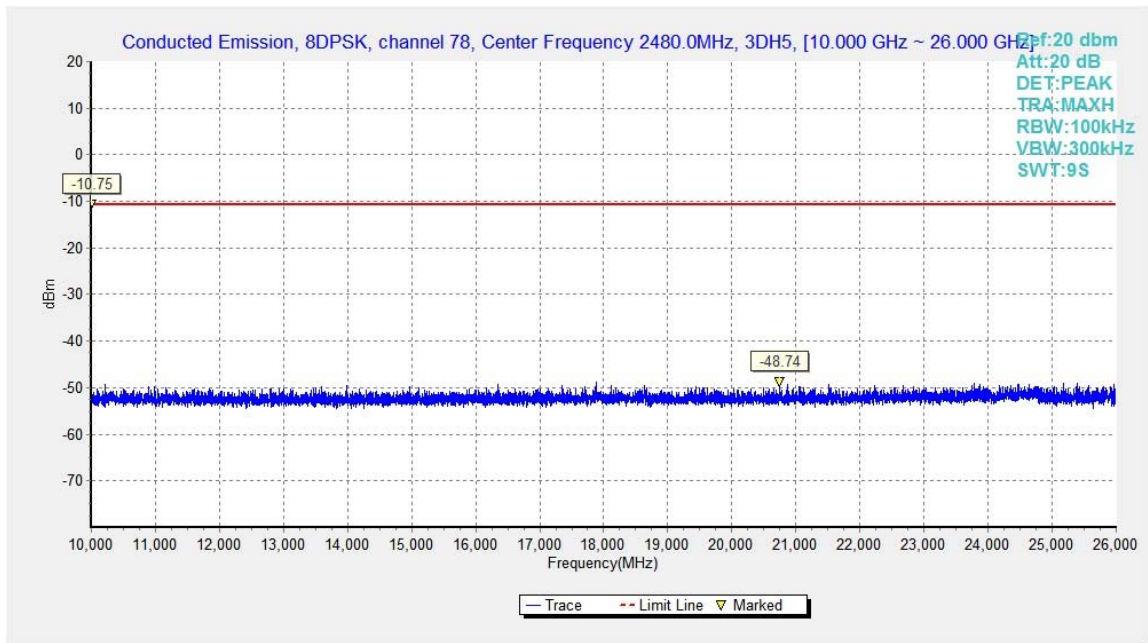
Fig.64. Conducted spurious emission: 8DPSK, Channel 78, 10GHz - 26GHz
