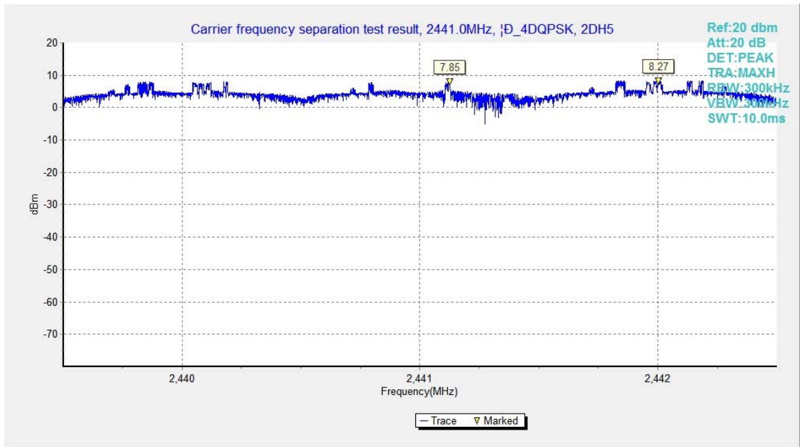
Fig.93. Carrier frequency separation measurement: \pi/4 DQPSK, Channel 39
