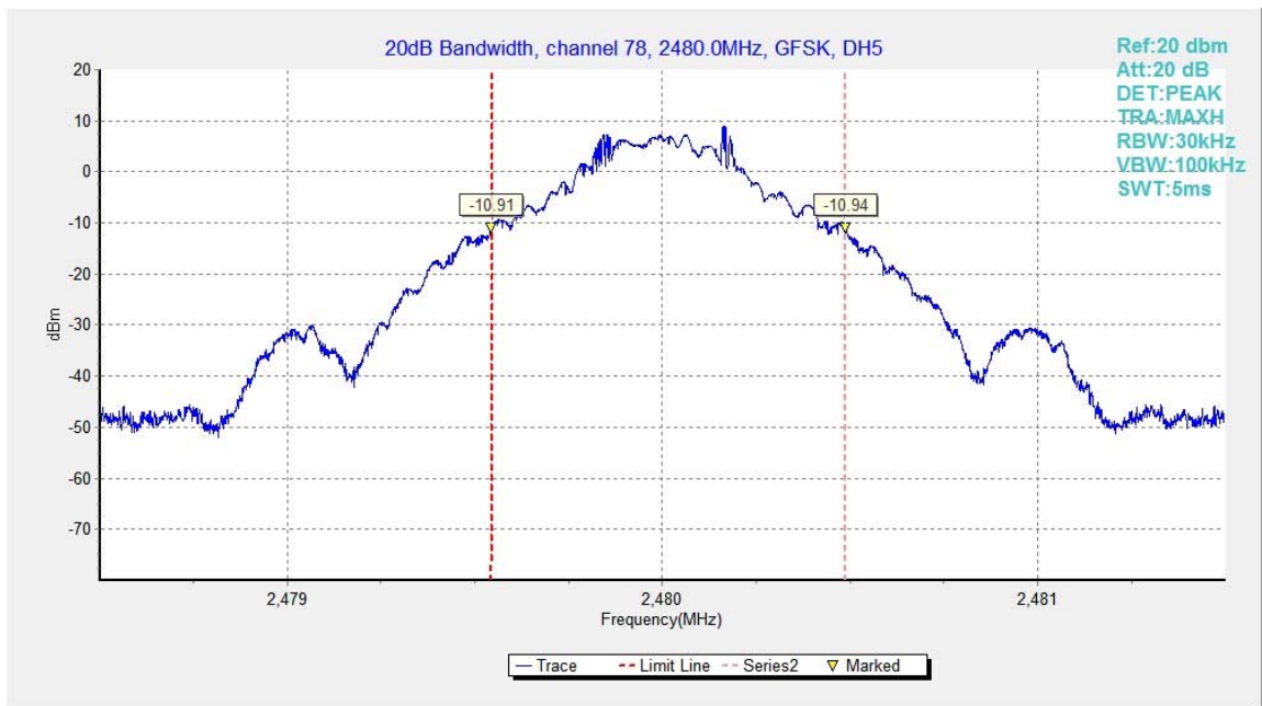
Fig.85. 20dB Bandwidth: GFSK, Channel 78
