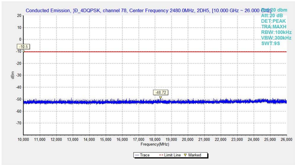
Fig.49. Conducted spurious emission: \pi/4 DQPSK, Channel 78, 10GHz - 26GHz
