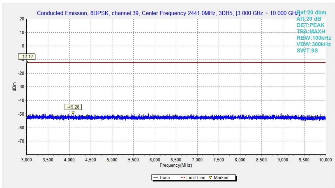
Fig.58. Conducted spurious emission: 8DPSK, Channel 39, 3GHz - 10GHz
