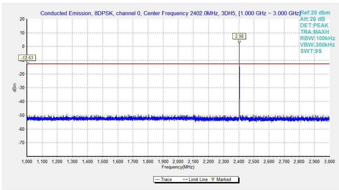
Fig.52. Conducted spurious emission: 8DPSK, Channel 0, 1GHz - 3GHz
