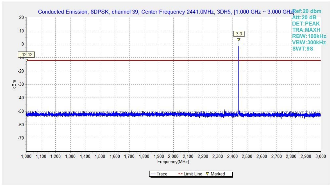
Fig.57. Conducted spurious emission: 8DPSK, Channel 39, 1GHz - 3GHz
