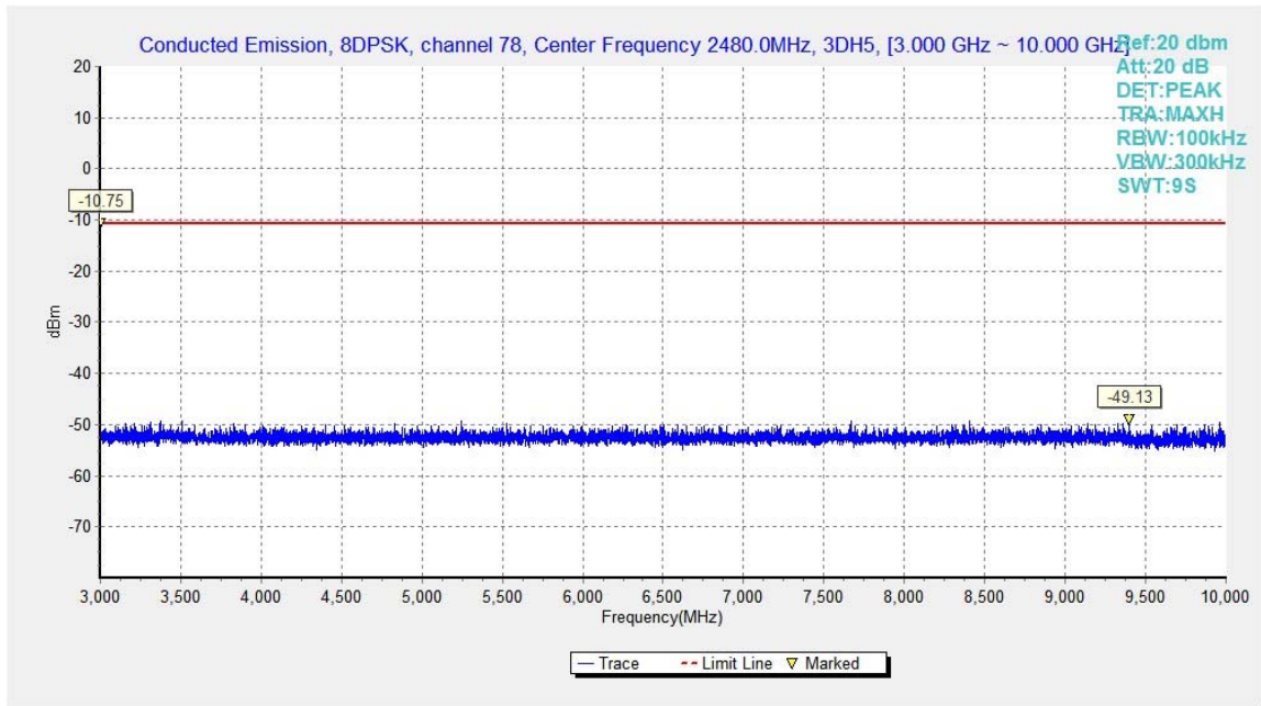
Fig.63. Conducted spurious emission: 8DPSK, Channel 78, 3GHz - 10GHz
