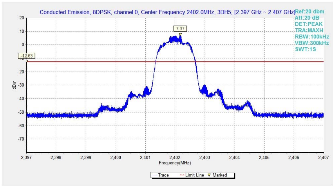
Fig.50. Conducted spurious emission: 8DPSK, Channel 0, 2402MHz
