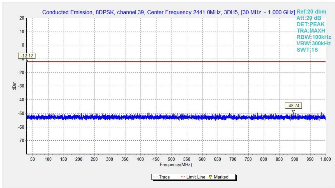
Fig.56. Conducted spurious emission: 8DPSK, Channel 39, 30MHz - 1GHz
