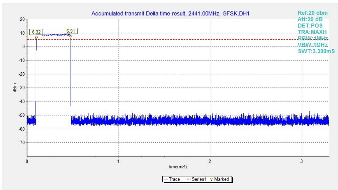
Fig.65. Time of occupancy (Dwell Time): Channel 39, Packet DH1
