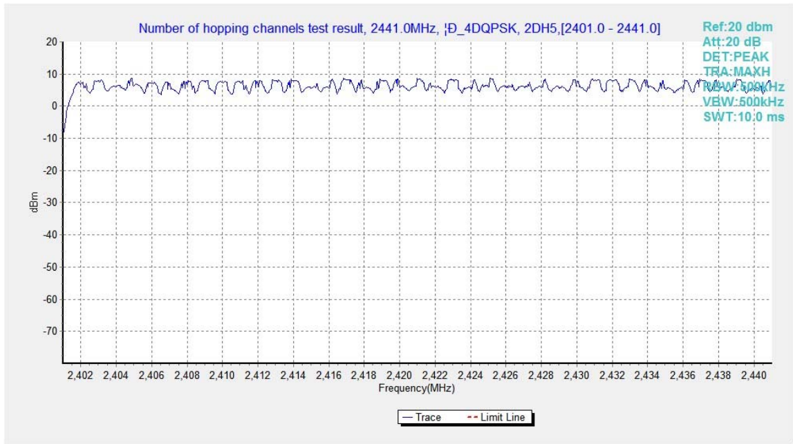
Fig.97. Number of hopping frequencies: \pi/4 DQPSK, Channel 0 - 39
