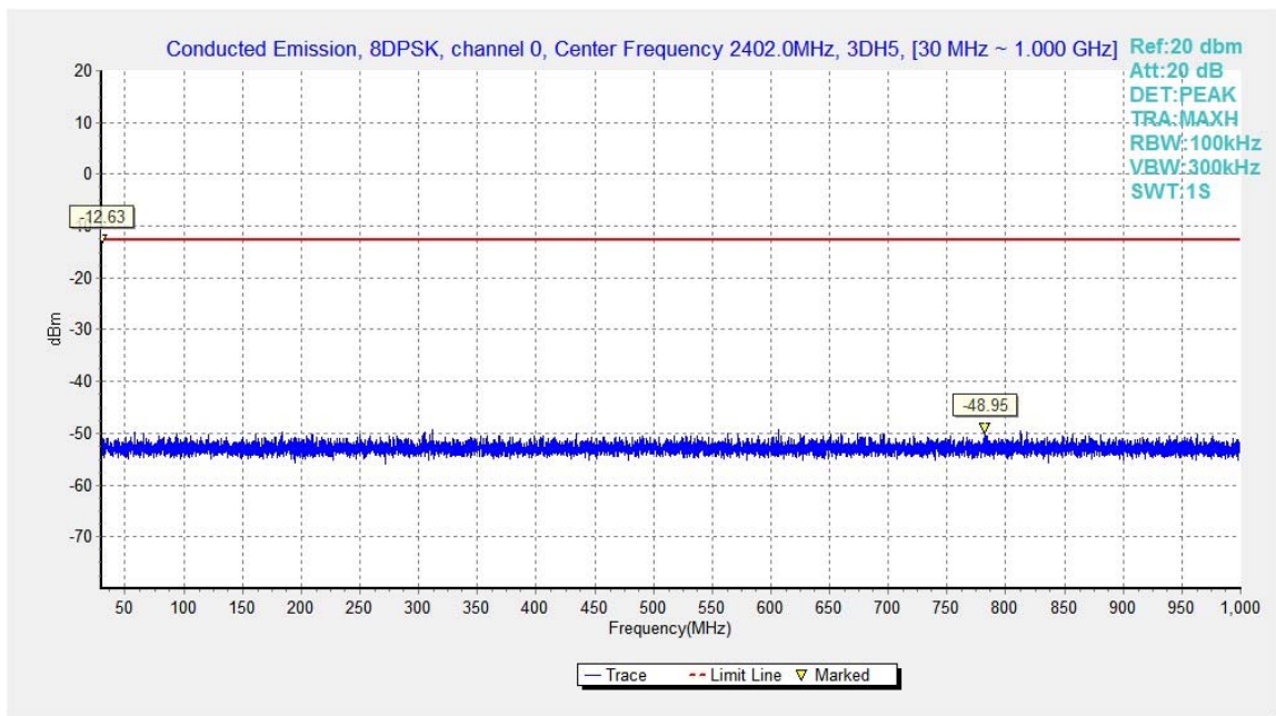
Fig.51. Conducted spurious emission: 8DPSK, Channel 0, 30MHz - 1GHz
