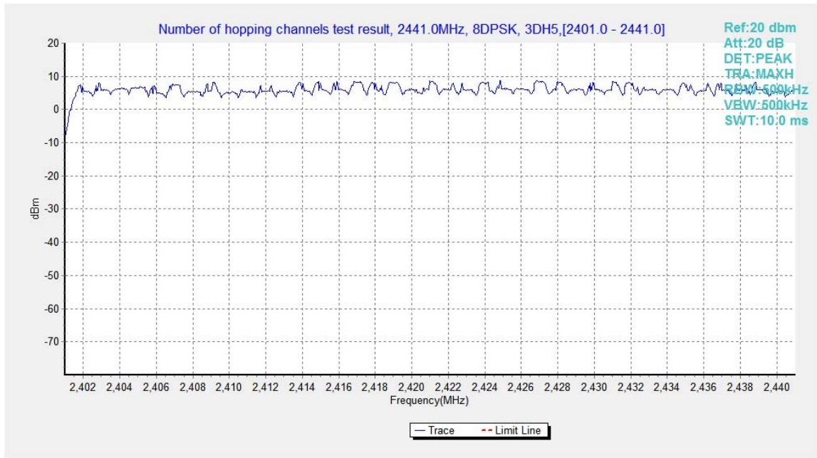
Fig.99. Number of hopping frequencies: 8DPSK, Channel 0 - 39
