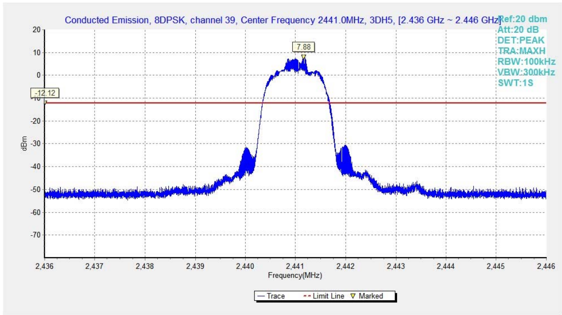
Fig.55. Conducted spurious emission: 8DPSK, Channel 39, 2441MHz
