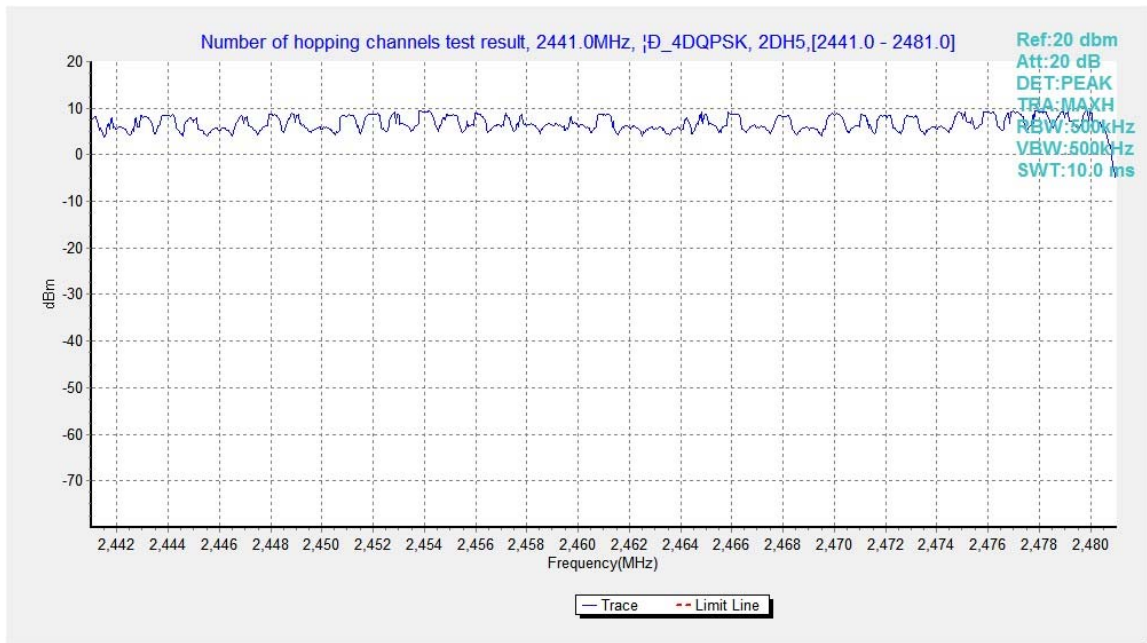
Fig.98. Number of hopping frequencies: \pi/4 DQPSK, Channel 40 - 78
