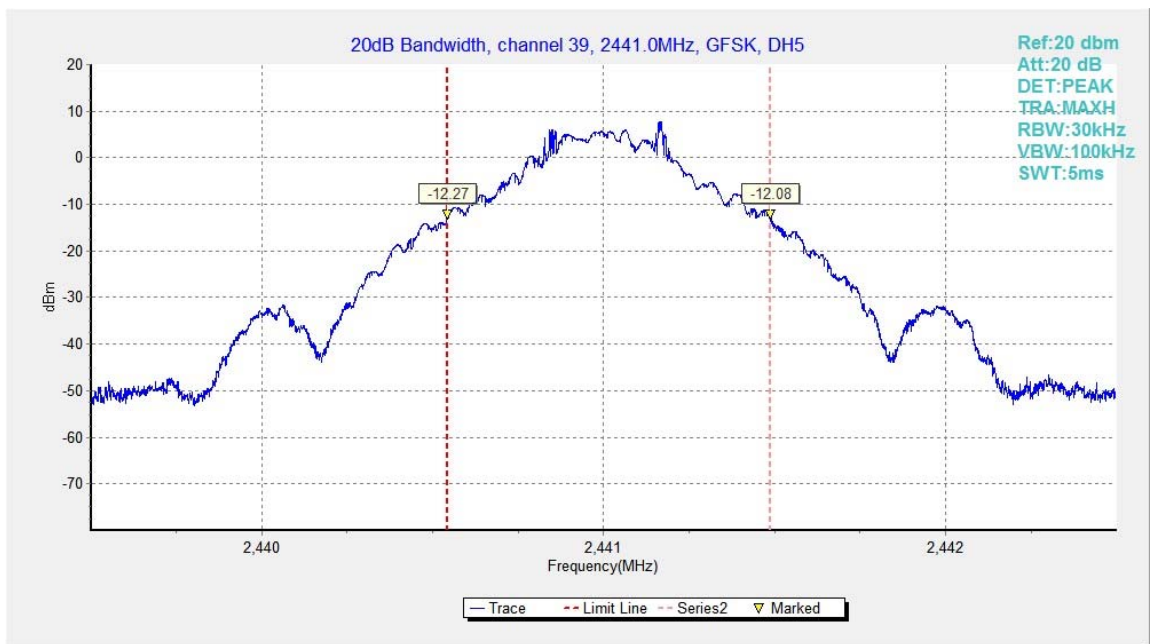
Fig.84. 20dB Bandwidth: GFSK, Channel 39
