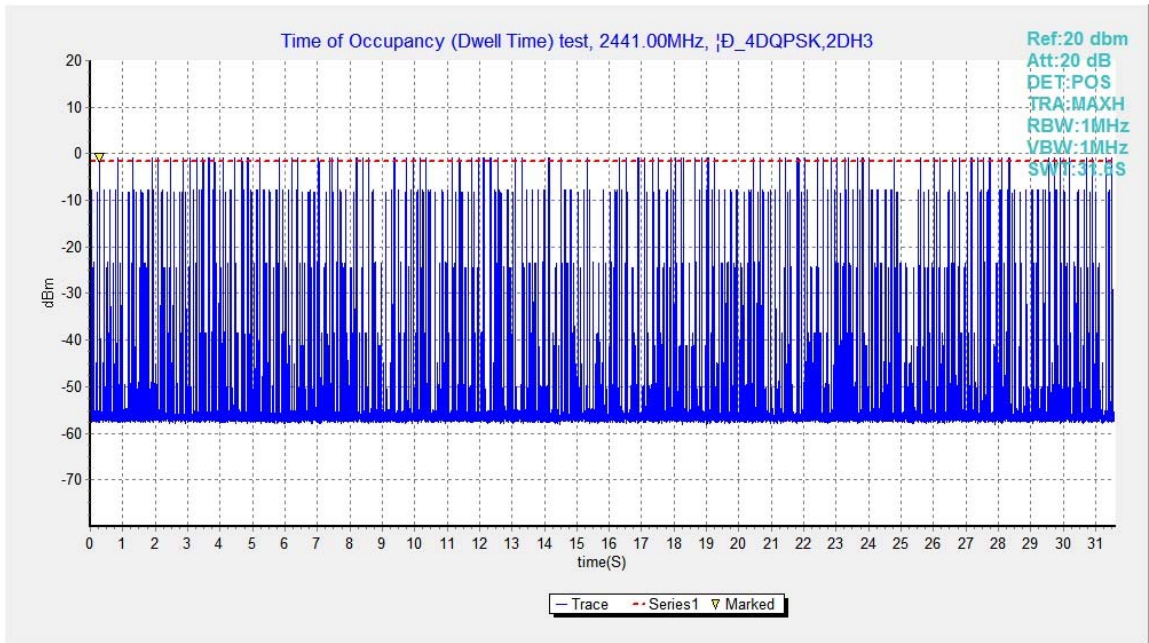
Fig.74. Number of Transmissions Measurement: Channel 39,Packet 2-DH3
