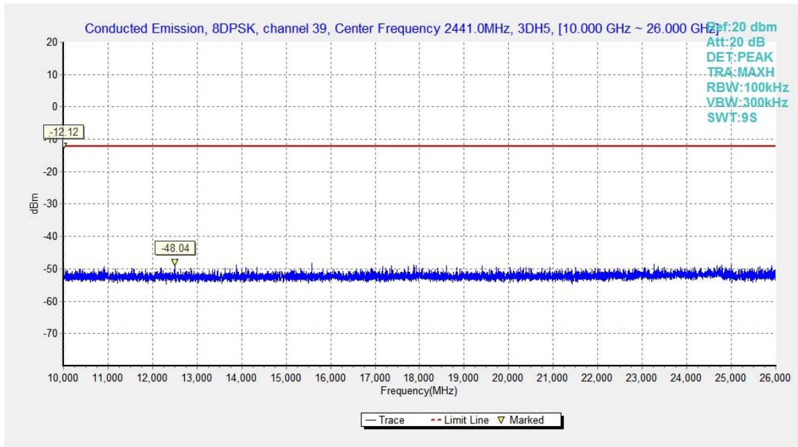
Fig.59. Conducted spurious emission: 8DPSK, Channel 39, 10GHz – 26GHz
