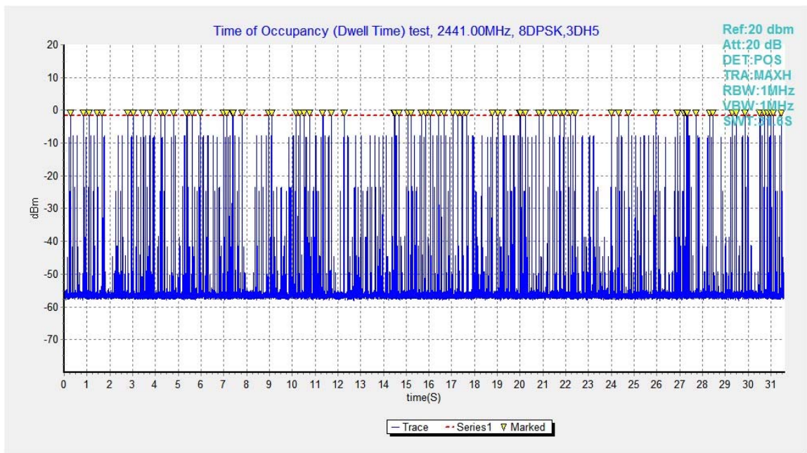
Fig.82. Number of Transmissions Measurement: Channel 39,Packet 3-DH5
