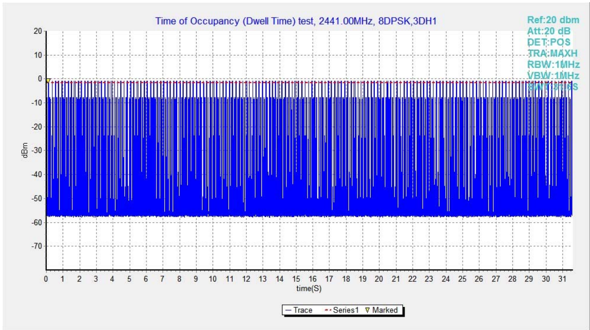
Fig.78. Number of Transmissions Measurement: Channel 39,Packet 3-DH1
