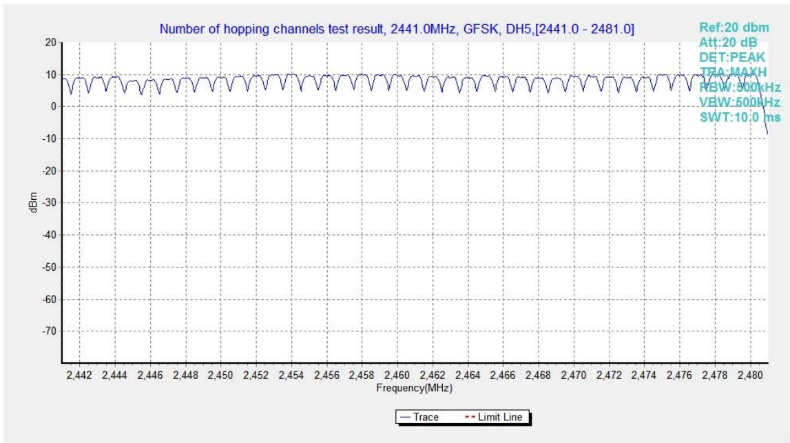
Fig.96. Number of hopping frequencies: GFSK, Channel 40 - 78
