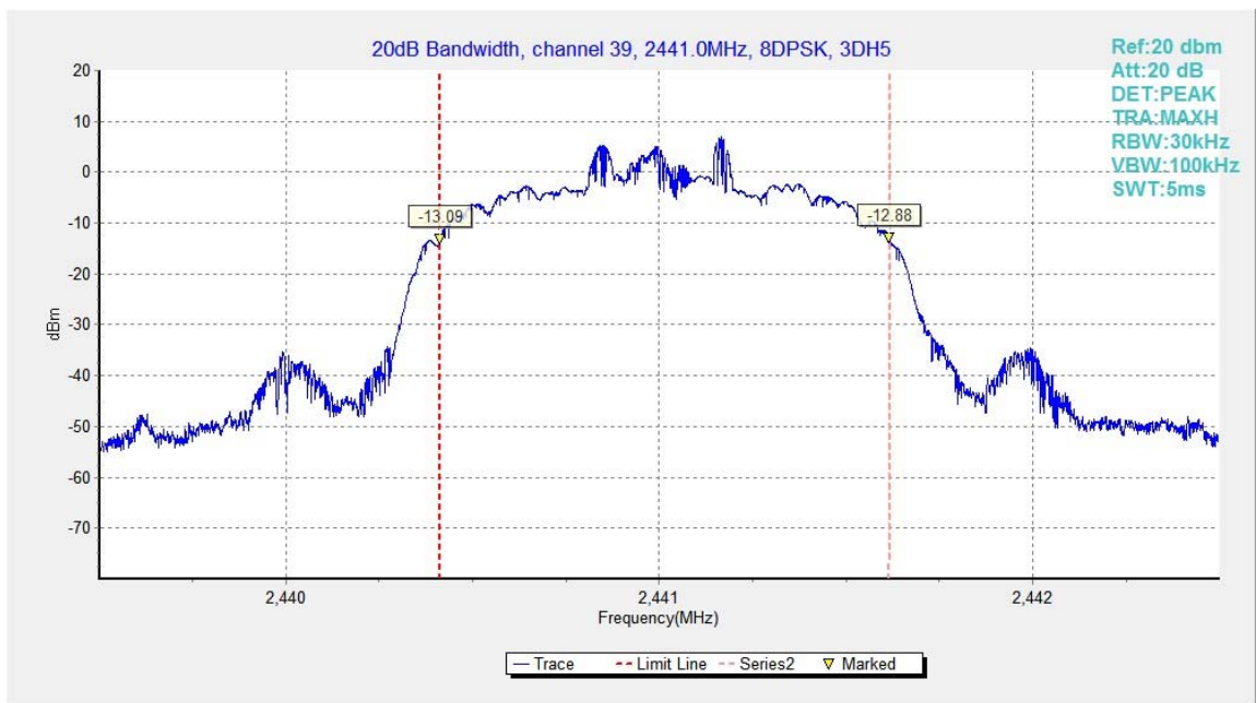
Fig.90. 20dB Bandwidth: 8DPSK, Channel 39
