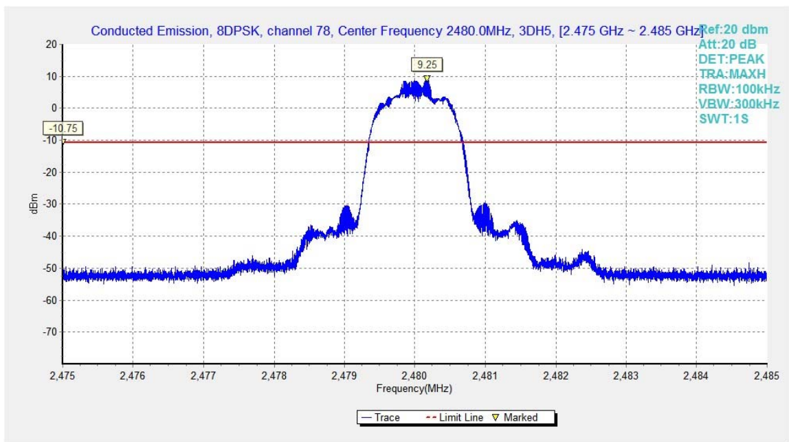
Fig.60. Conducted spurious emission: 8DPSK, Channel 78, 2480MHz
