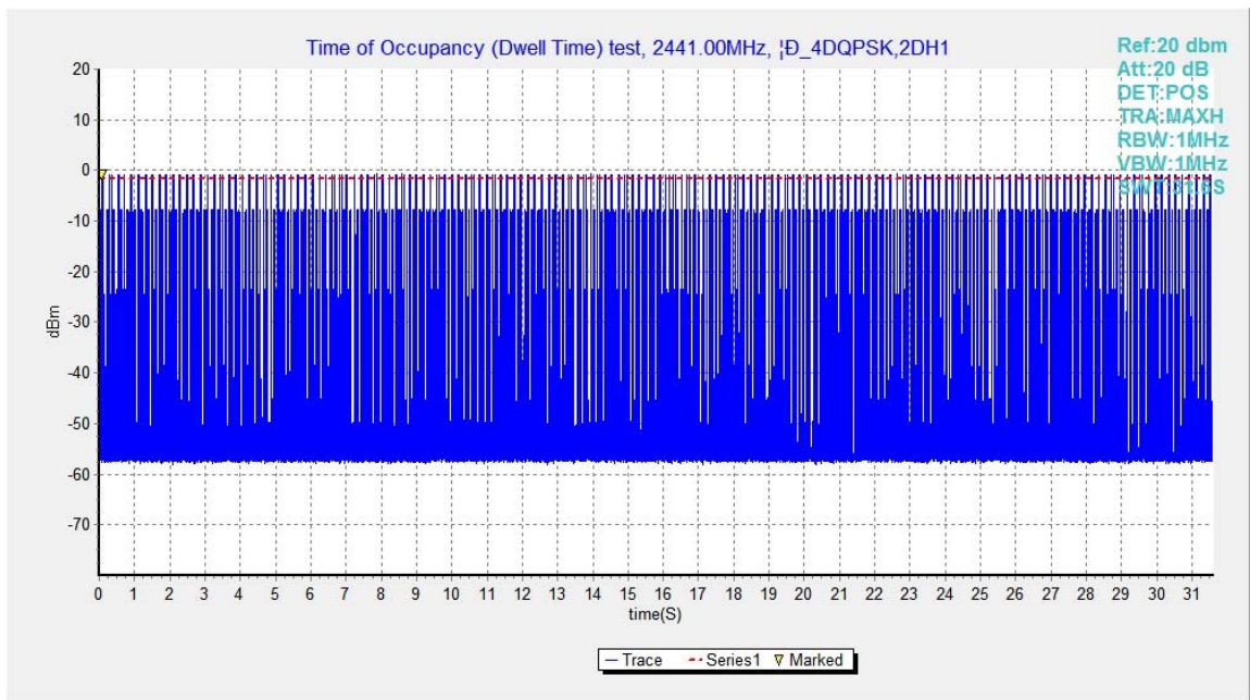
Fig.72. Number of Transmissions Measurement: Channel 39,Packet 2-DH1
