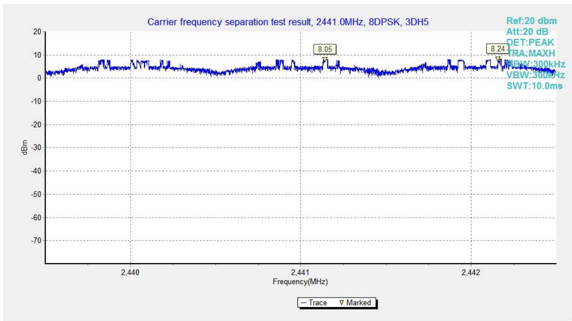
Fig.94. Carrier frequency separation measurement: 8DPSK, Channel 39
