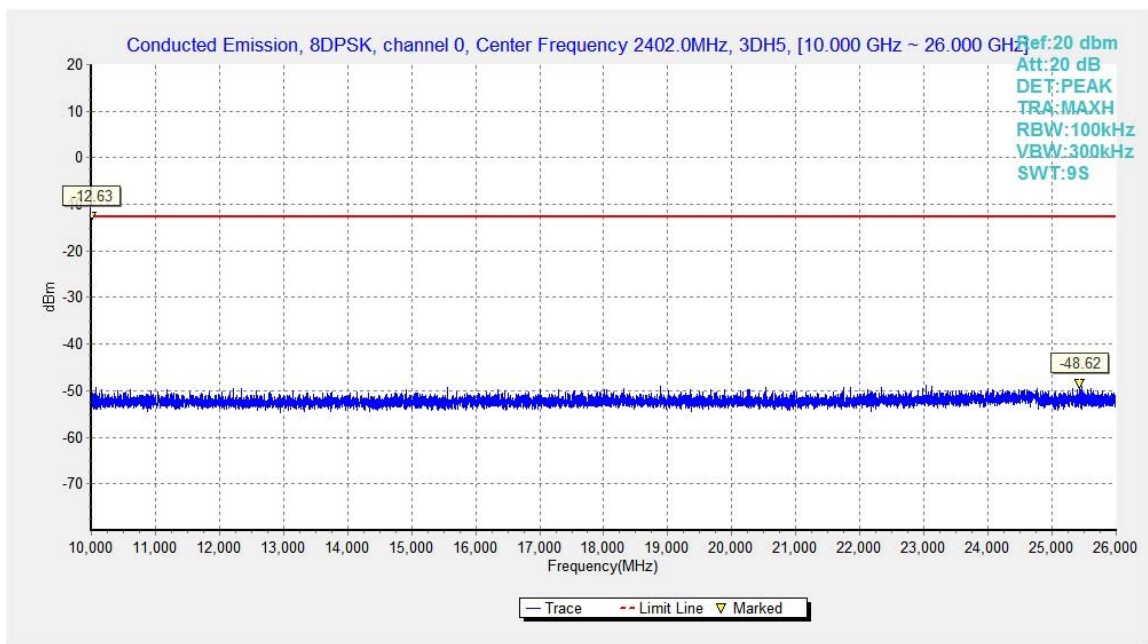
Fig.54. Conducted spurious emission: 8DPSK, Channel 0, 10GHz - 26GHz
