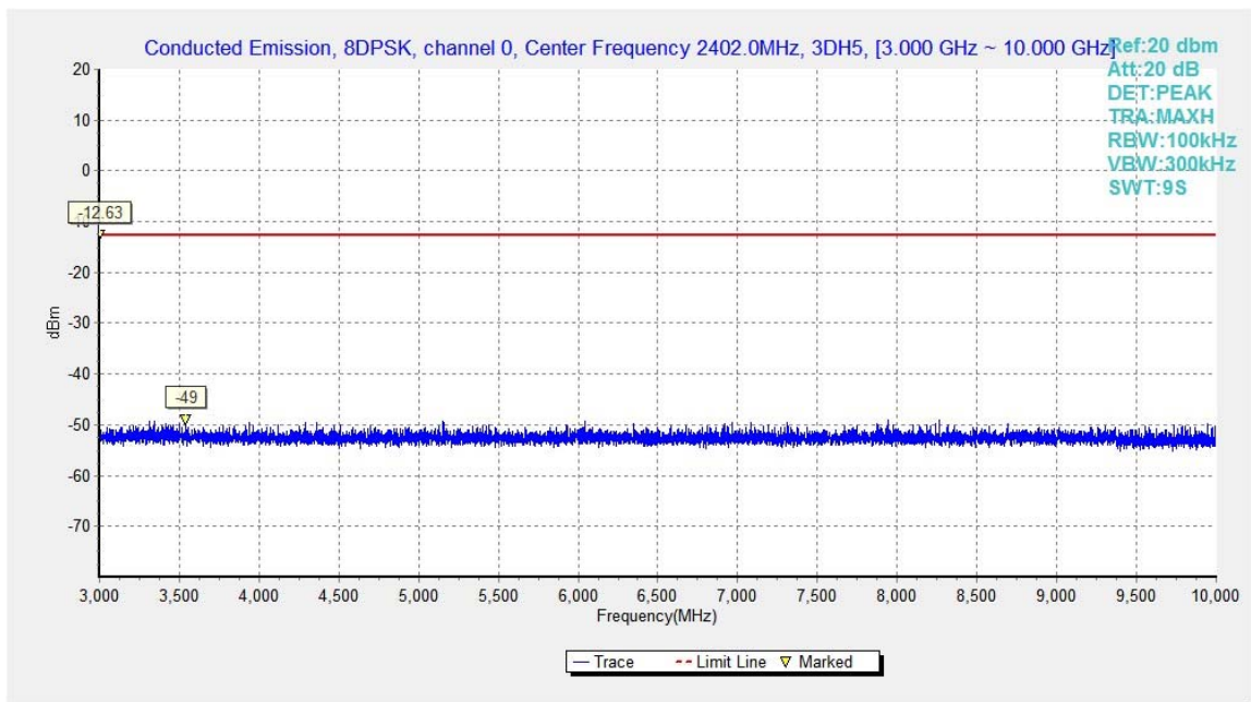
Fig.53. Conducted spurious emission: 8DPSK, Channel 0, 3GHz - 10GHz
