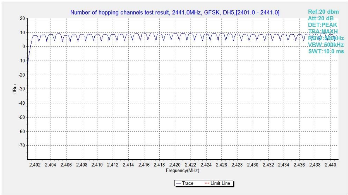
Fig.95. Number of hopping frequencies: GFSK, Channel 0 - 39
