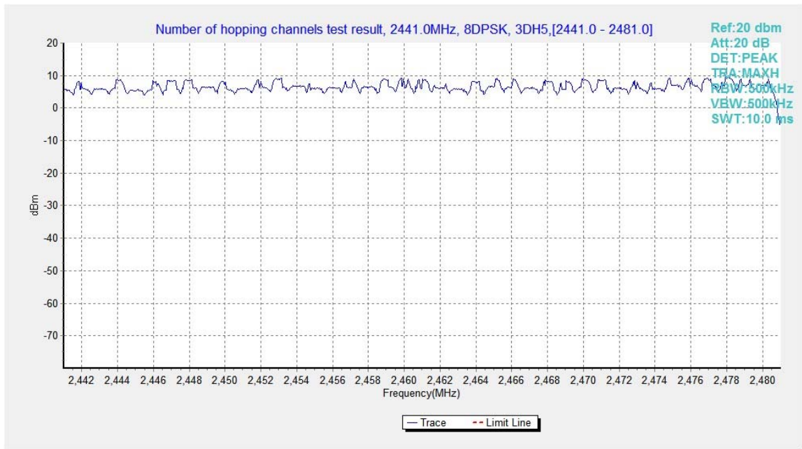
Fig.100. Number of hopping frequencies: 8DPSK, Channel 40 - 78
