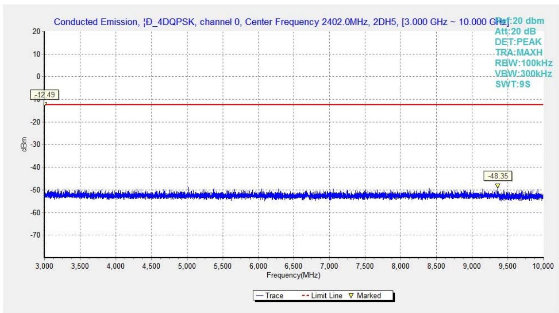
Fig.38. Conducted spurious emission: \pi/4 DQPSK, Channel 0, 3GHz - 10GHz
