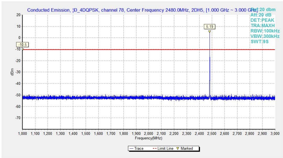
Fig.47. Conducted spurious emission: \pi/4 DQPSK, Channel 78, 1GHz - 3GHz
