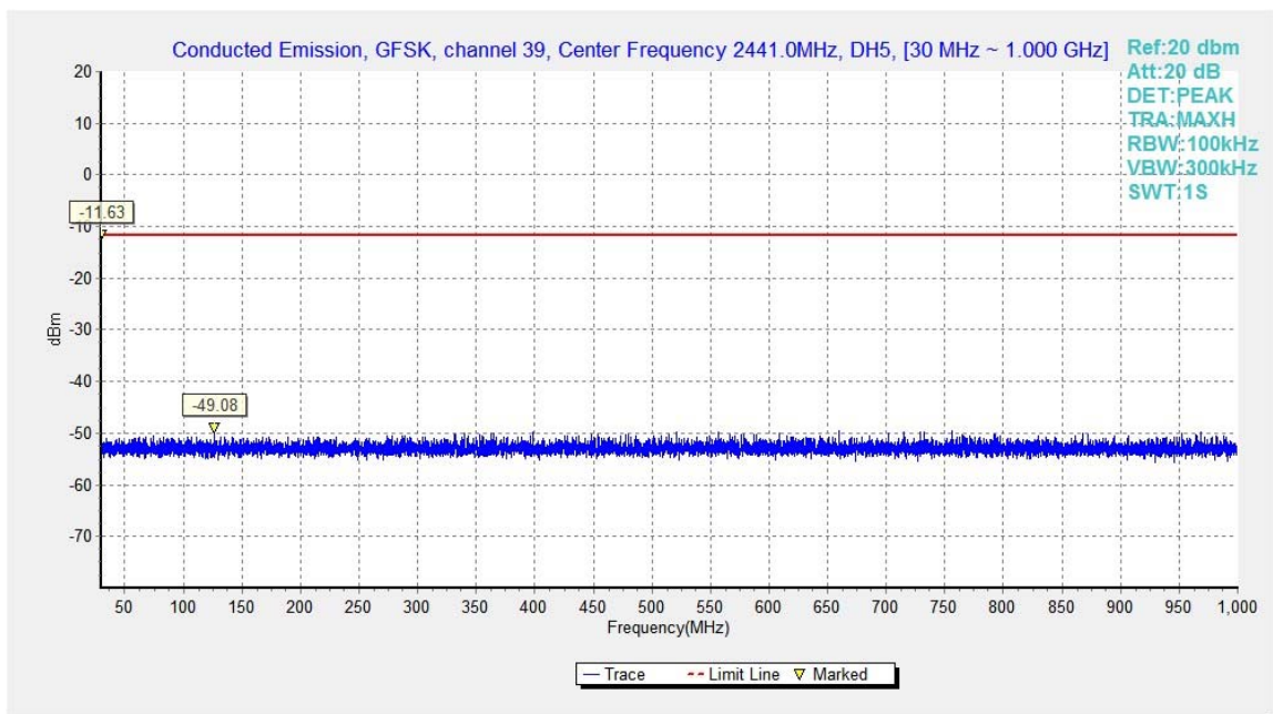
Fig.26. Conducted spurious emission: GFSK, Channel 39, 30MHz - 1GHz
