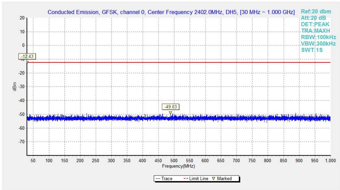
Fig.21. Conducted spurious emission: GFSK, Channel 0, 30MHz - 1GHz
