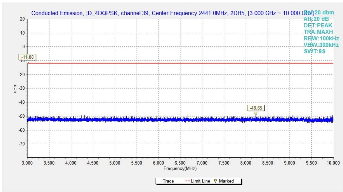
Fig.43. Conducted spurious emission: \pi/4 DQPSK, Channel 39, 3GHz - 10GHz
