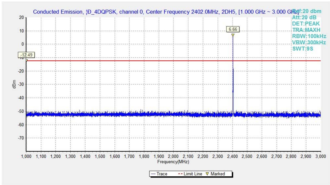
Fig.37. Conducted spurious emission: \pi/4 DQPSK, Channel 0, 1GHz - 3GHz
