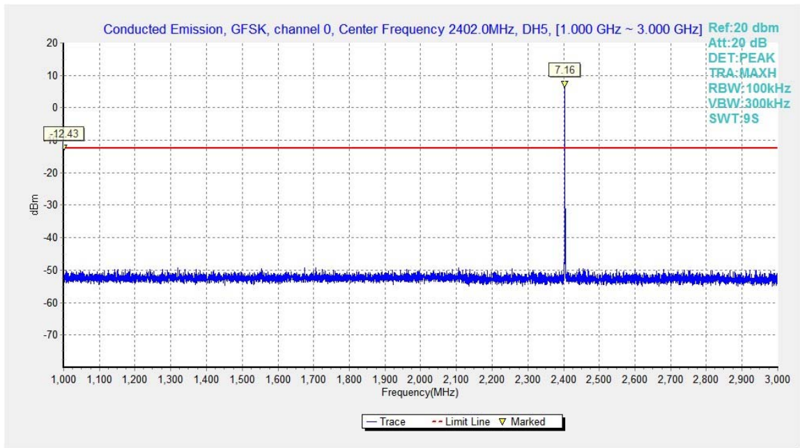
Fig.22. Conducted spurious emission: GFSK, Channel 0, 1GHz - 3GHz
