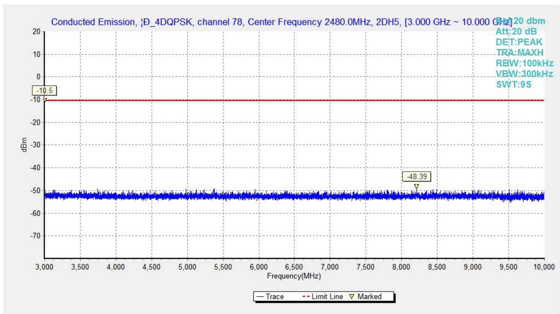
Fig.48. Conducted spurious emission: \pi/4 DQPSK, Channel 78, 3GHz - 10GHz
