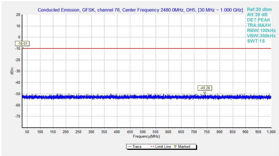
Fig.31. Conducted spurious emission: GFSK, Channel 78, 30MHz - 1GHz
