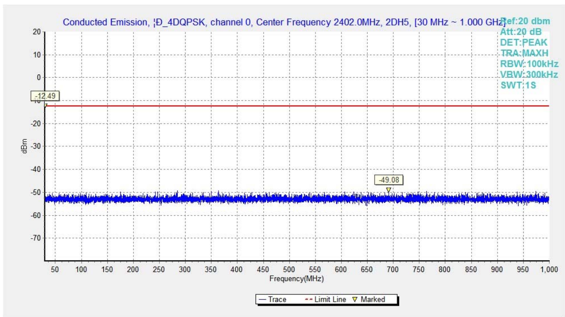
Fig.36. Conducted spurious emission: \pi/4 DQPSK, Channel 0, 30MHz - 1GHz
