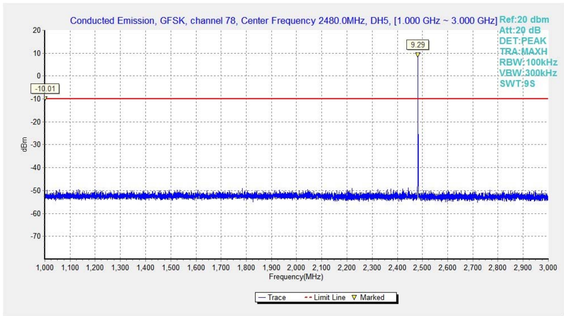
Fig.32. Conducted spurious emission: GFSK, Channel 78, 1GHz - 3GHz
