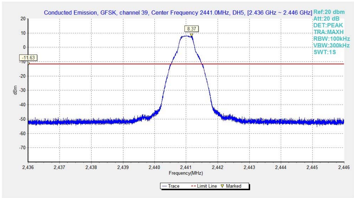
Fig.25. Conducted spurious emission: GFSK, Channel 39, 2441MHz
