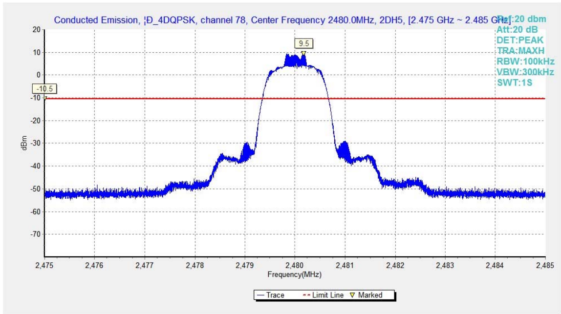
Fig.45. Conducted spurious emission: \pi/4 DQPSK, Channel 78, 2480MHz
