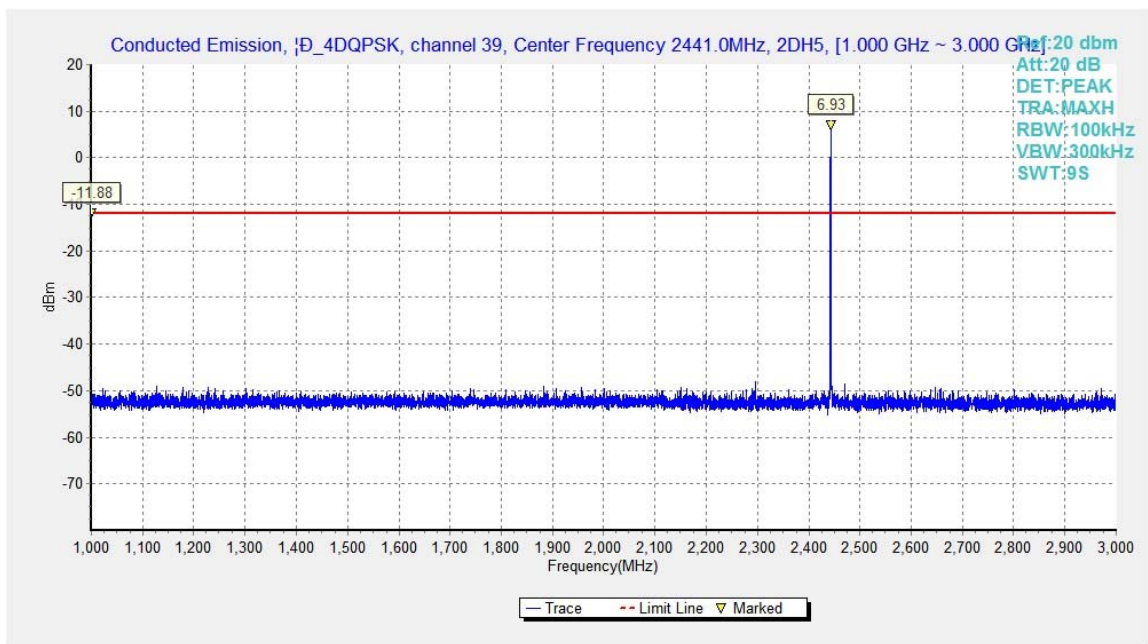
Fig.42. Conducted spurious emission: \pi/4 DQPSK, Channel 39, 1GHz - 3GHz
