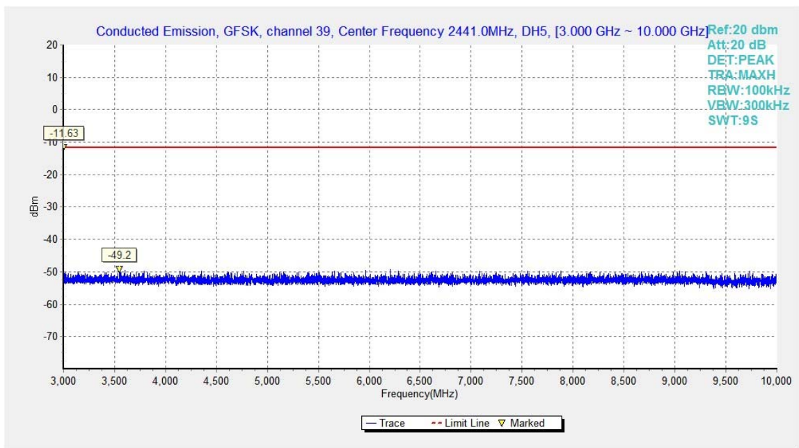
Fig.28. Conducted spurious emission: GFSK, Channel 39, 3GHz – 10GHz
