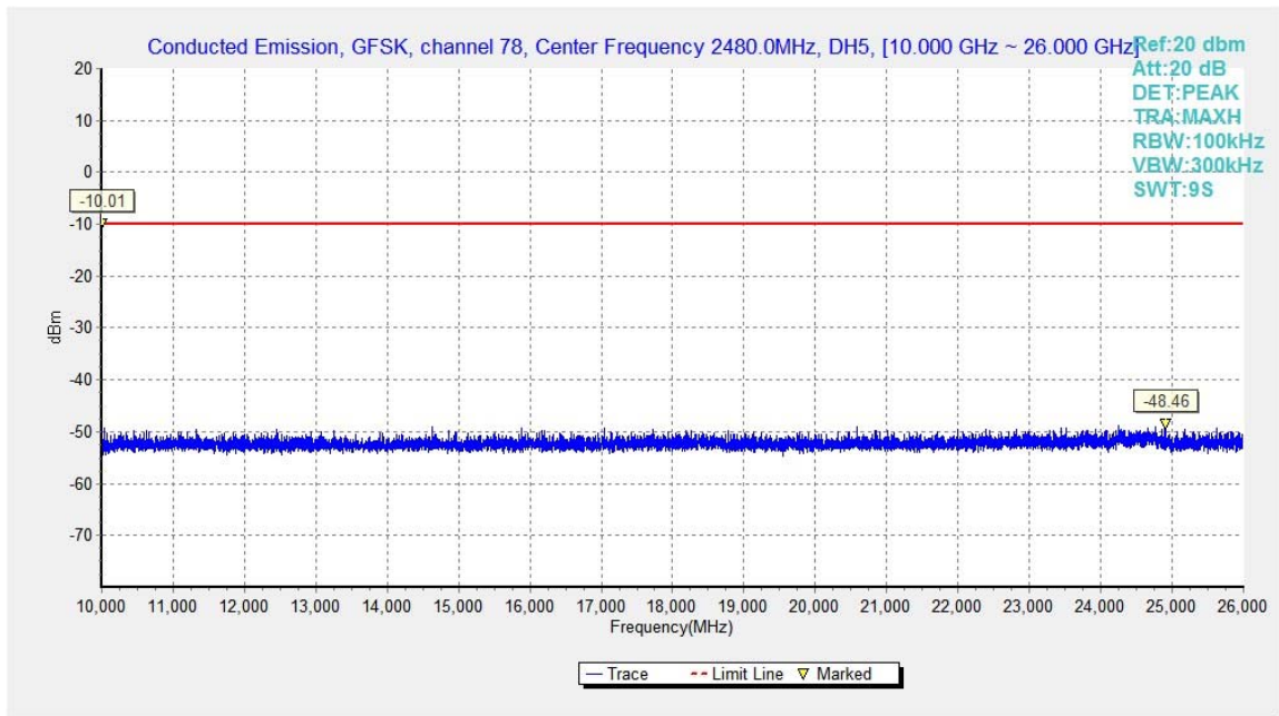
Fig.34. Conducted spurious emission: GFSK, Channel 78, 10GHz - 26GHz
