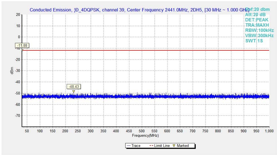
Fig.41. Conducted spurious emission: \pi/4 DQPSK, Channel 39, 30MHz - 1GHz
