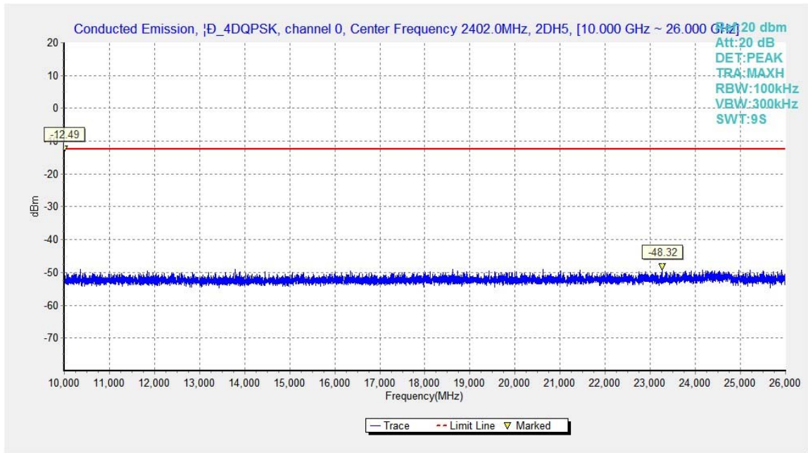
Fig.39. Conducted spurious emission: \pi/4 DQPSK, Channel 0, 10GHz - 26GHz
