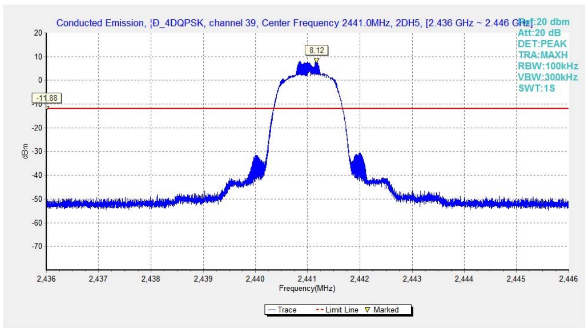
Fig.40. Conducted spurious emission: \pi/4 DQPSK, Channel 39, 2441MHz
