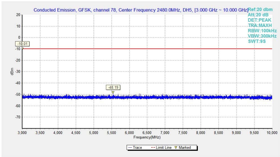
Fig.33. Conducted spurious emission: GFSK, Channel 78, 3GHz - 10GHz
