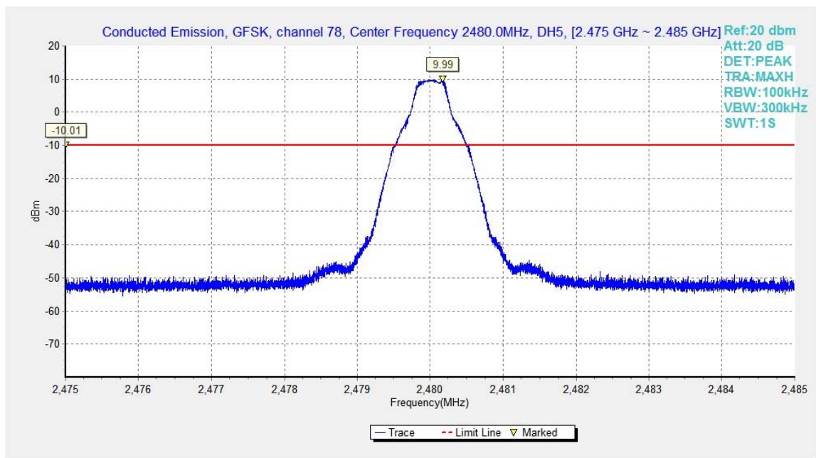
Fig.30. Conducted spurious emission: GFSK, Channel 78, 2480MHz
