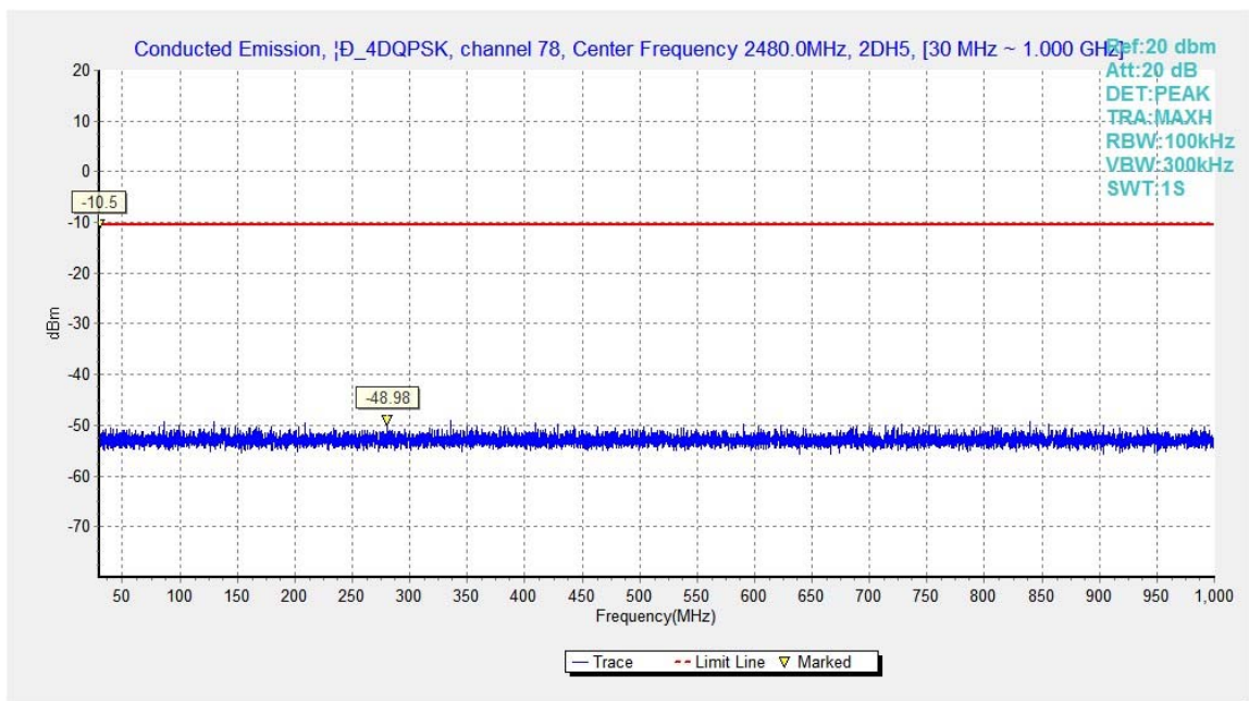
Fig.46. Conducted spurious emission: \pi/4 DQPSK, Channel 78, 30MHz - 1GHz
