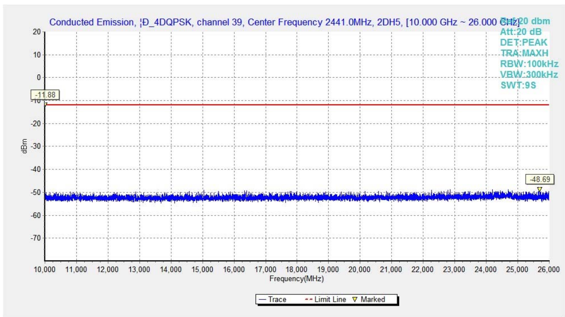
Fig.44. Conducted spurious emission: \pi/4 DQPSK, Channel 39, 10GHz – 26GHz
