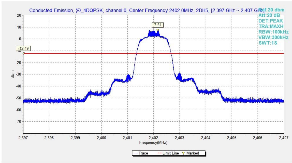
Fig.35. Conducted spurious emission: \pi/4 DQPSK, Channel 0, 2402MHz
