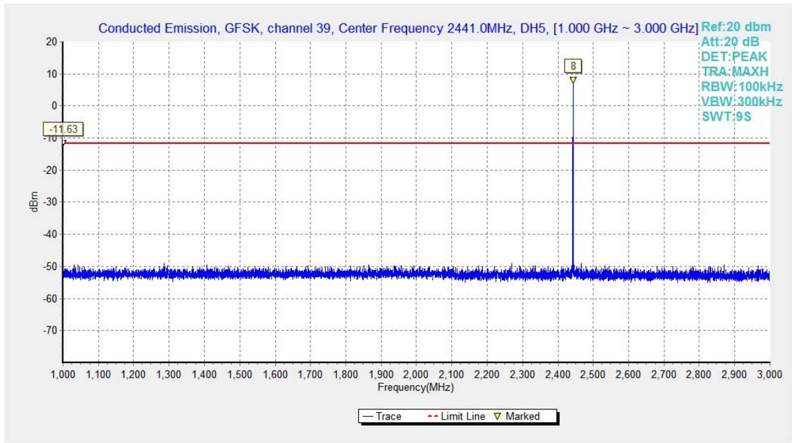
Fig.27. Conducted spurious emission: GFSK, Channel 39, 1GHz – 3GHz
