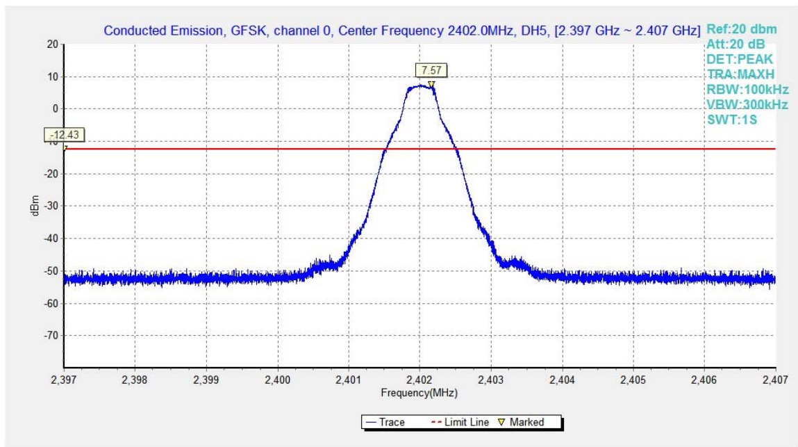
Fig.20. Conducted spurious emission: GFSK, Channel 0, 2402MHz
