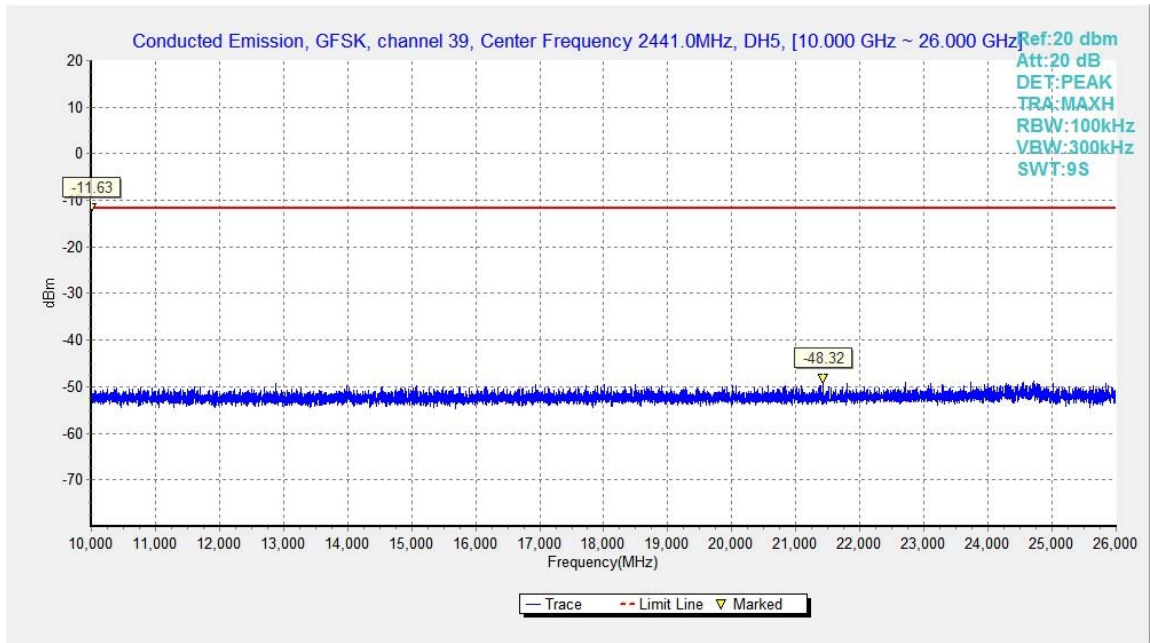
Fig.29. Conducted spurious emission: GFSK, Channel 39, 10GHz – 26GHz
