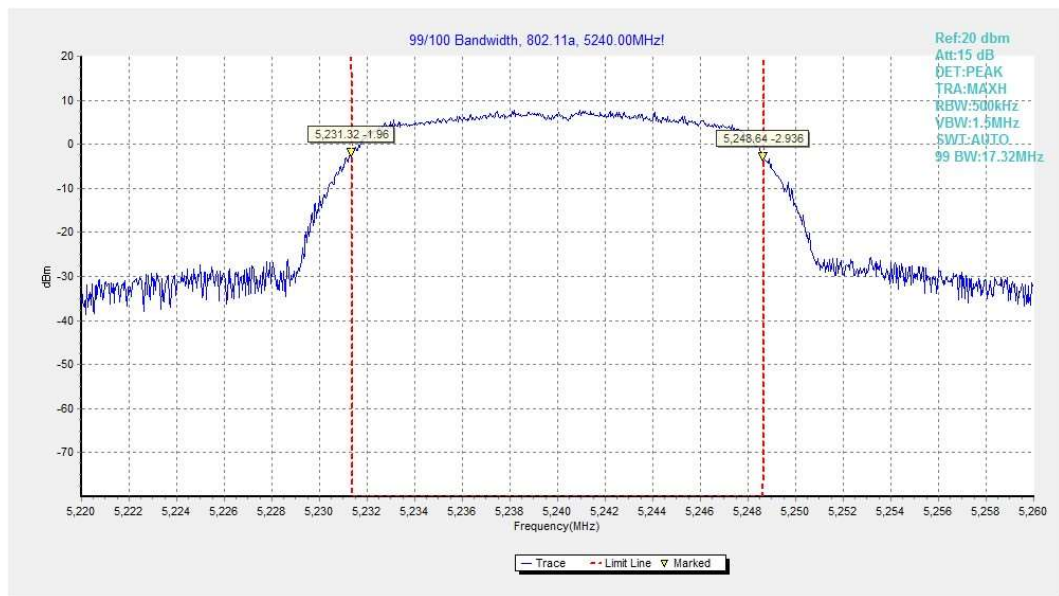
Fig.71 99% Occupied bandwidth (802.11a, 5240MHz)
