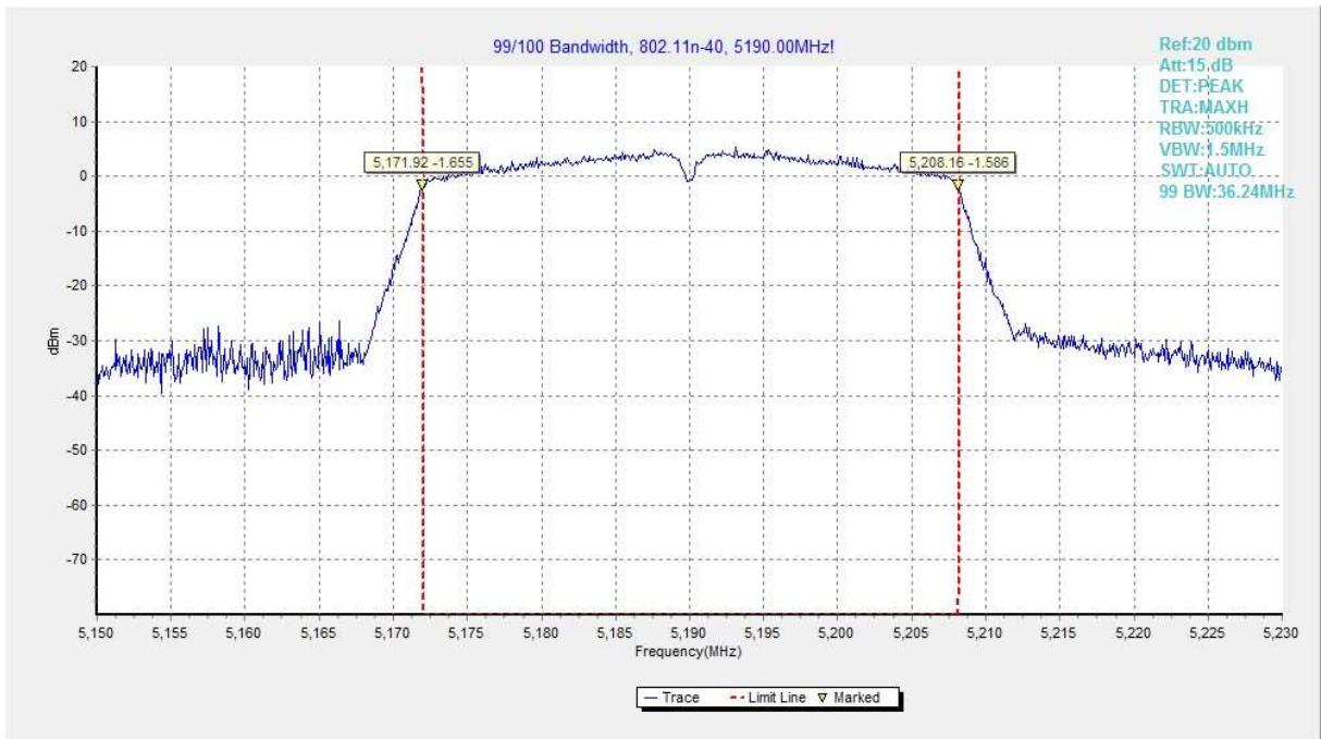
Fig.75 99% Occupied bandwidth (802.11n-HT40, 5190MHz)
