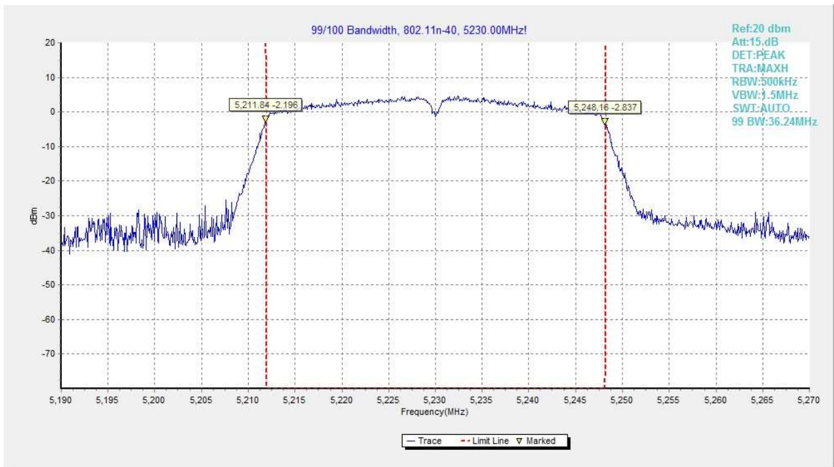
Fig.76 99% Occupied bandwidth (802.11n-HT40, 5230MHz)
