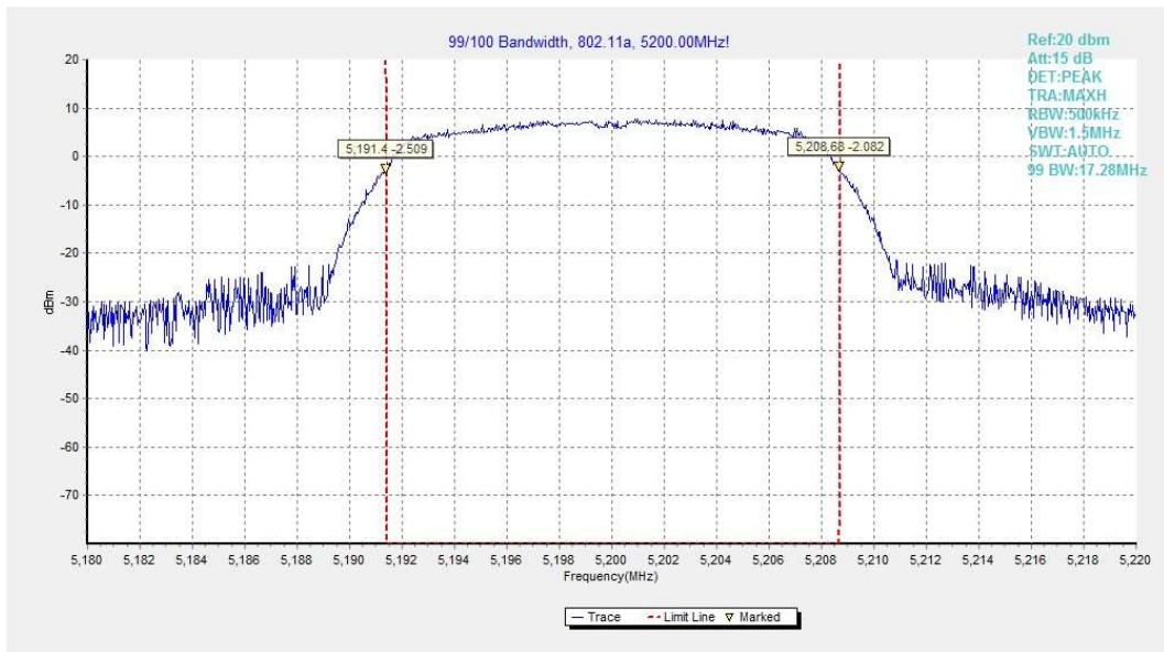
Fig.70 99% Occupied bandwidth (802.11a, 5200MHz)
