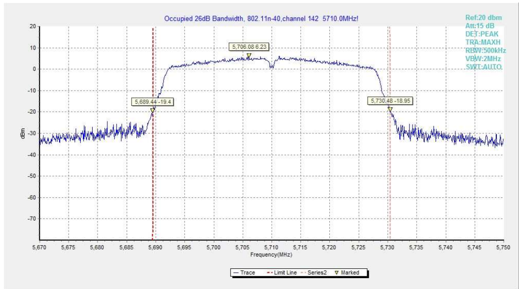
Fig.28 Occupied 26dB Bandwidth (802.11n-HT40, 5710MHz)
