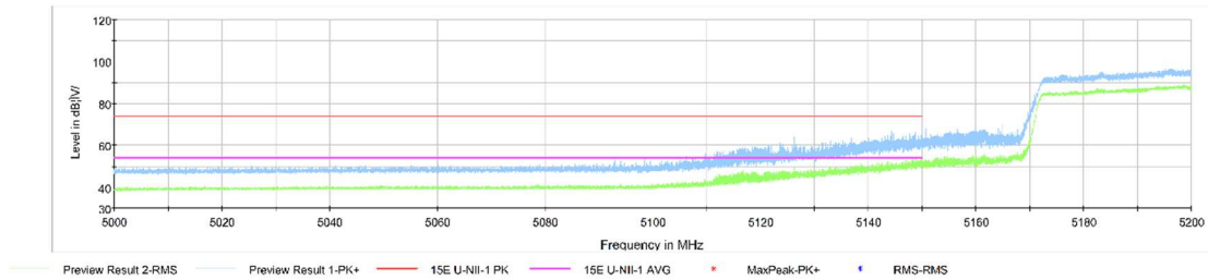
Fig.54 Band Edges (802.11ac-HT80 Ch42 , 5210MHz)
