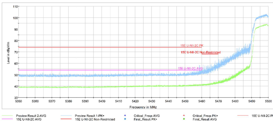
Fig.60 Band Edges (802.11a Ch100, 5500MHz)
