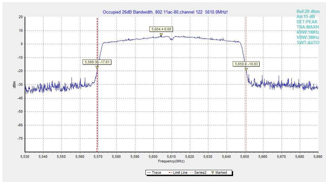
Fig.32 Occupied 26dB Bandwidth (802.11ac-HT80, 5610MHz)
