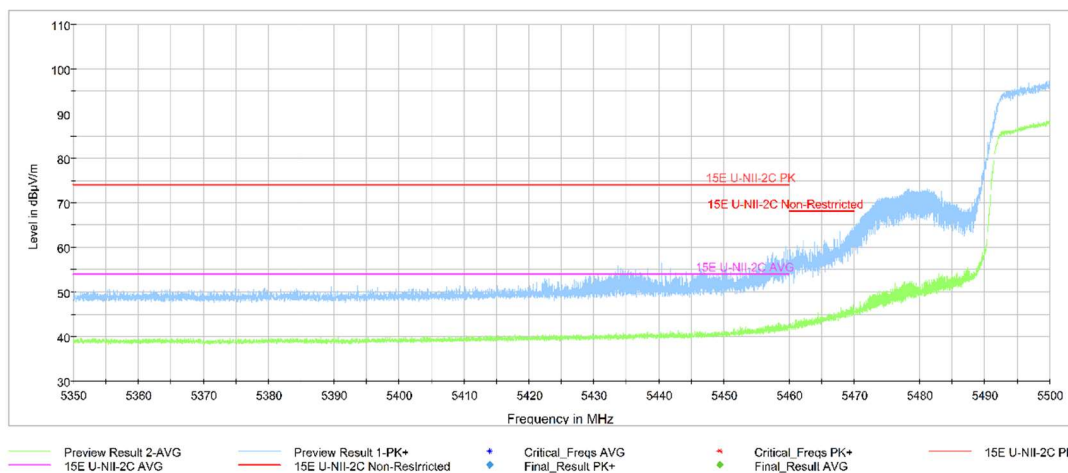
Fig.63 Band Edges (802.11n-HT40 Ch102, 5510MHz)
