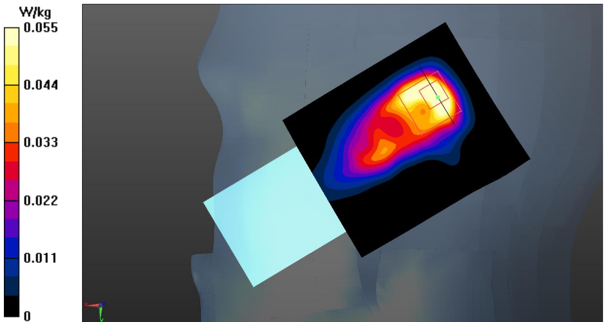
Fig.21 Bluetooth Head
