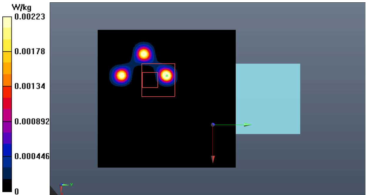
Fig.22 Bluetooth Body
