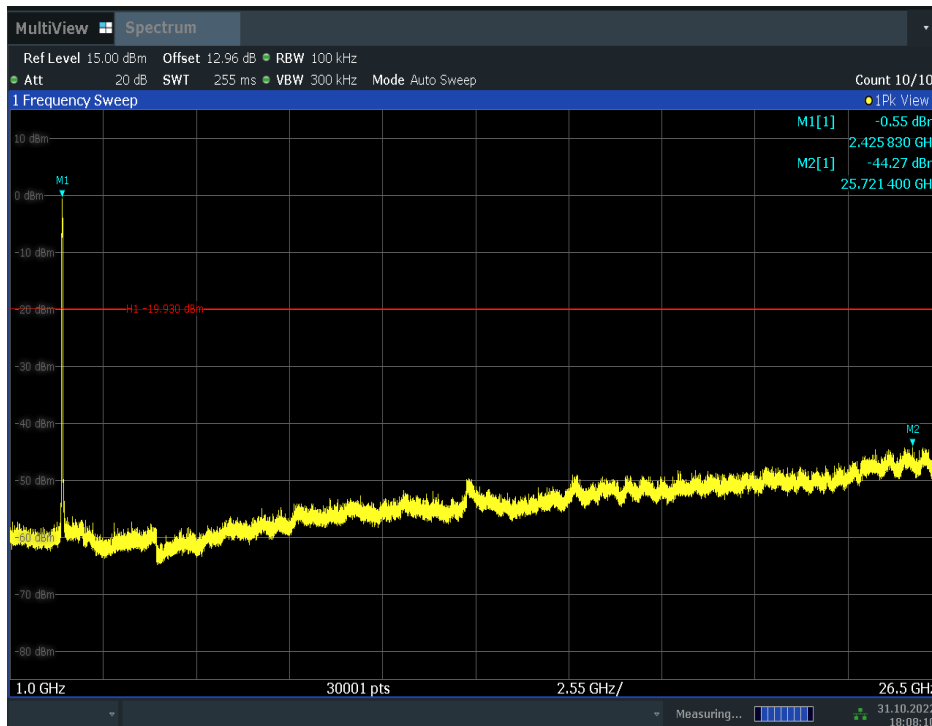
Fig.A.6.1.48 Transmitter Spurious Emission - Conducted (802.11n-HT40, Ch3, 1 GHz-26.5 GHz)
