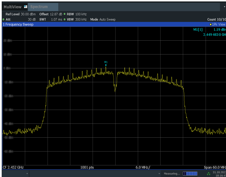
Fig.A.6.1.52 Transmitter Spurious Emission - Conducted (802.11n-HT40, Ch9, Center Frequency)
