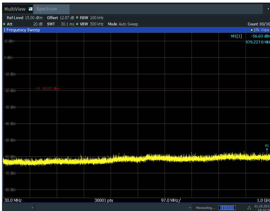
Fig.A.6.1.53 Transmitter Spurious Emission - Conducted (802.11n-HT40, Ch9, 30 MHz-1
