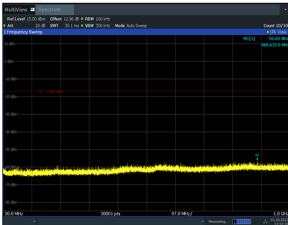
Fig.A.6.1.41 Transmitter Spurious Emission - Conducted (802.11n-HT20, Ch6, 30 MHz-1)
