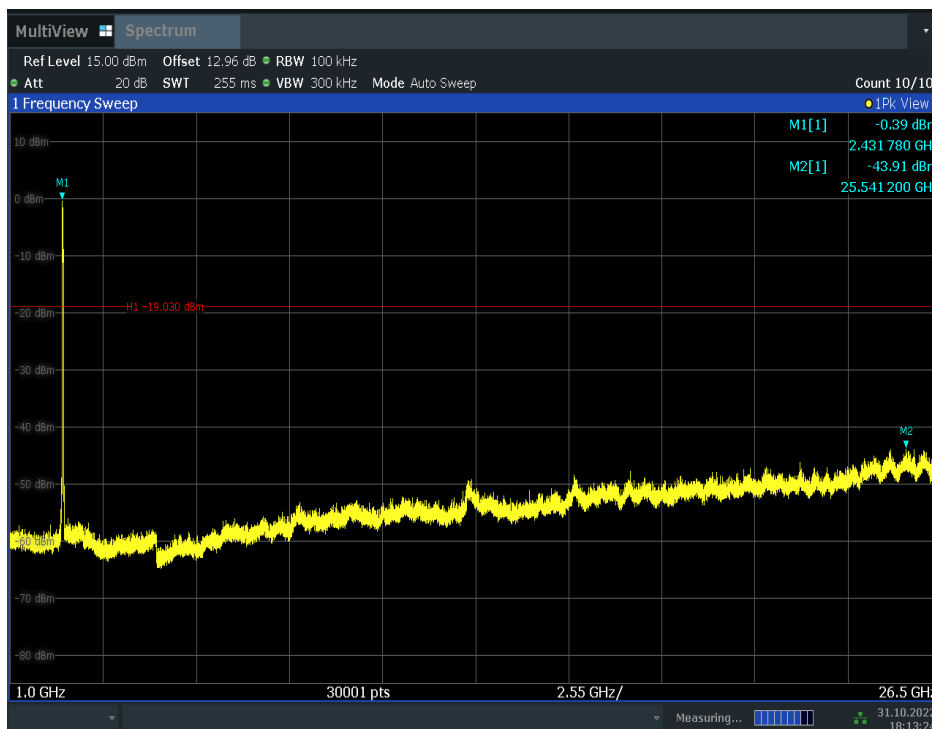
Fig.A.6.1.51 Transmitter Spurious Emission - Conducted (802.11n-HT40, Ch6, 1 GHz-26.5
