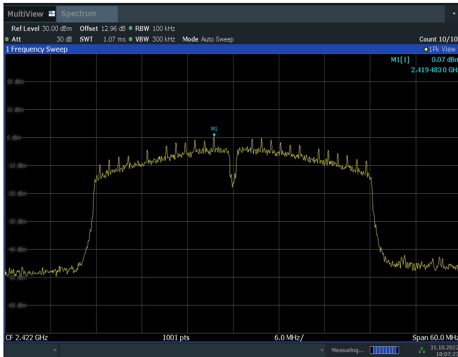
Fig.A.6.1.46 Transmitter Spurious Emission - Conducted (802.11n-HT40, Ch3, Center Frequency)
