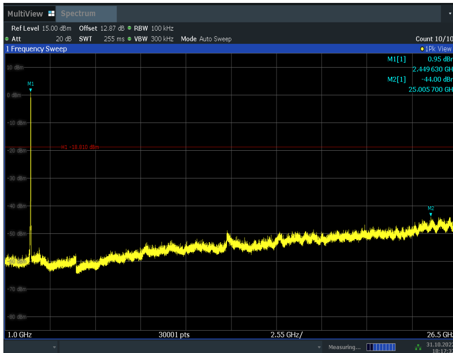
Fig.A.6.1.54 Transmitter Spurious Emission - Conducted (802.11n-HT40, Ch9, 1 GHz-26.5 GHz)
