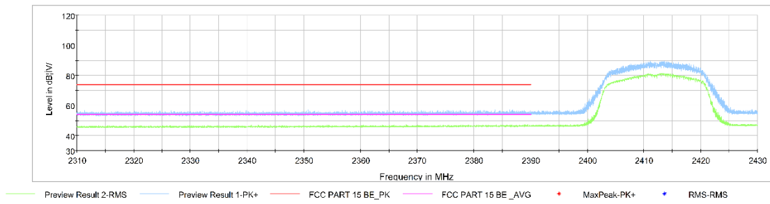
Fig.A.6.2.5 Transmitter Spurious Emission - Radiated (Power): 802.11n-HT20, ch1, 2.31 GHz - 2.43GHz
