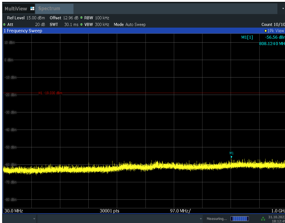
Fig.A.6.1.50 Transmitter Spurious Emission - Conducted (802.11n-HT40, Ch6, 30 MHz-1 GHz)
