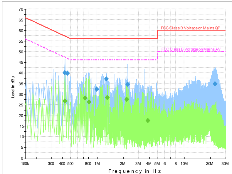
Fig.A.7.2 AC Powerline Conducted Emission-Idle
