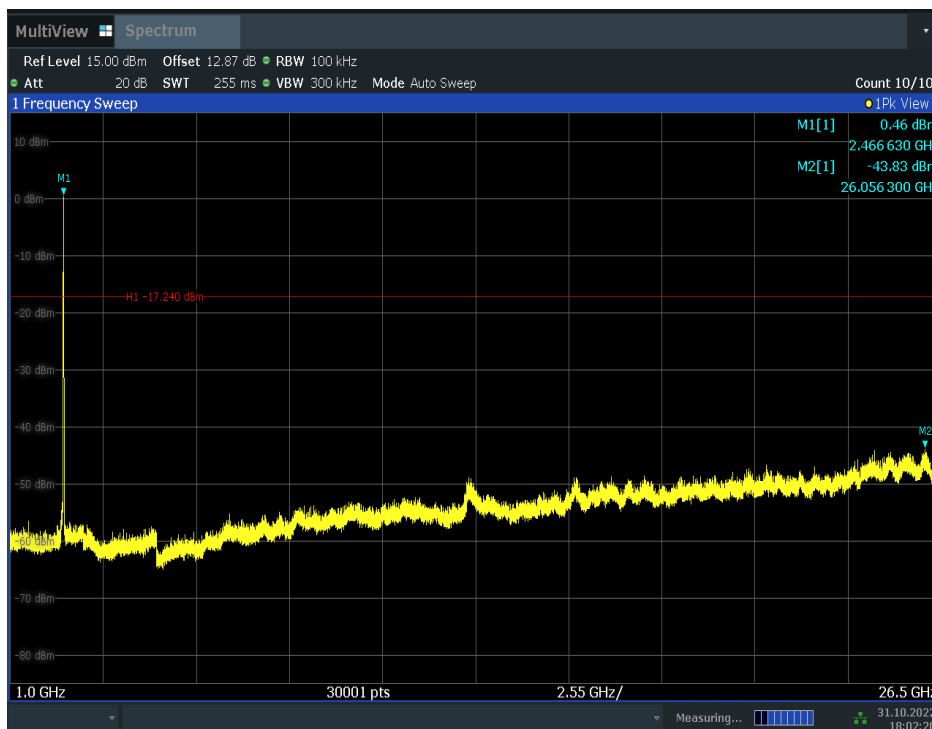
Fig.A.6.1.45 Transmitter Spurious Emission - Conducted (802.11n-HT20, Ch11, 1 GHz-26.5 GHz)
