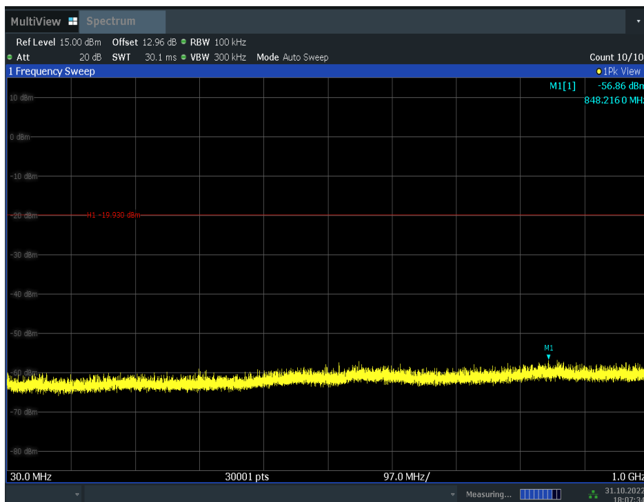
Fig.A.6.1.47 Transmitter Spurious Emission - Conducted (802.11n-HT40, Ch3, 30 MHz-1
