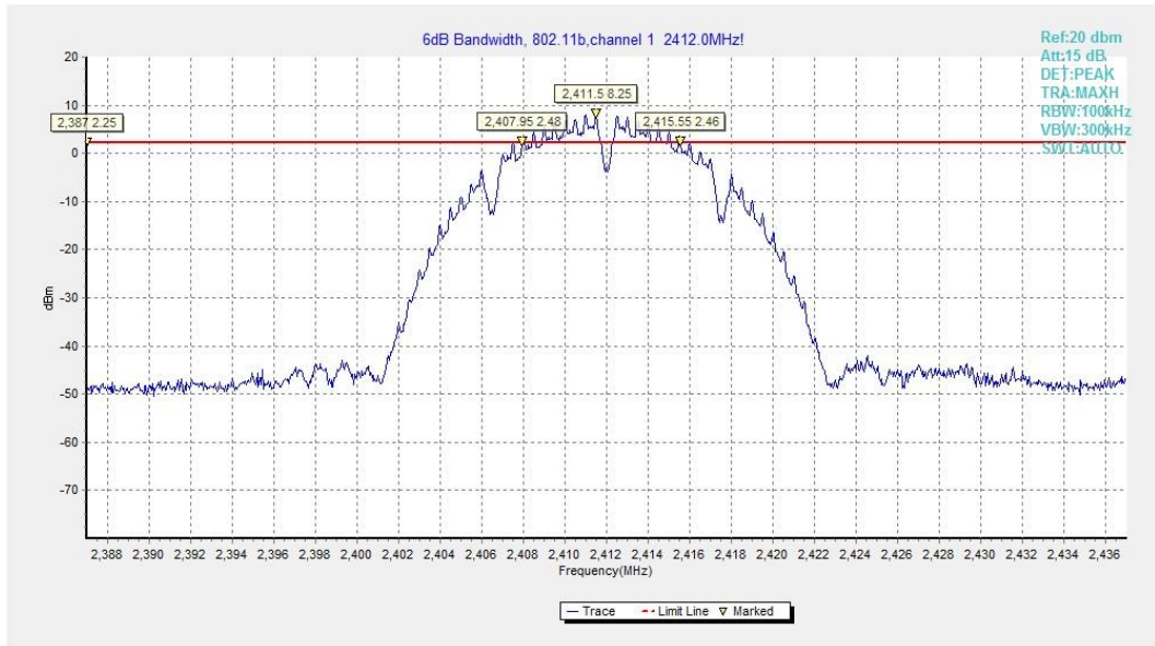
Fig.A.4.1 Occupied 6dB Bandwidth(802.11b,Ch 1)
