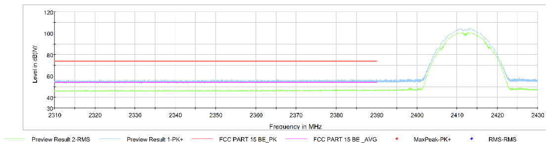
Fig.A.6.2.3 Transmitter Spurious Emission - Radiated (Power): 802.11g, ch1, 2.31 GHz - 2.43GHz
