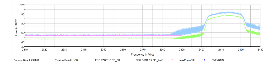
Fig.A.6.2.5 Transmitter Spurious Emission - Radiated (Power): 802.11n-HT20, ch1, 2.31 GHz - 2.43GHz
