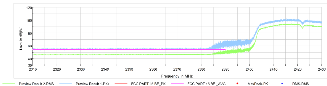
Fig.A.6.2.7 Transmitter Spurious Emission - Radiated (Power): 802.11n-HT40, ch3, 2.31 GHz - 2.43GHz
