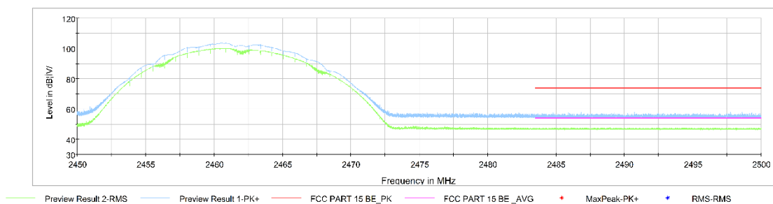
Fig.A.6.2.4 Transmitter Spurious Emission - Radiated (Power): 802.11g, ch11, 2.45 GHz - 2.50GHz
