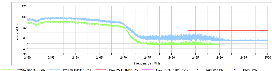
Fig.A.6.2.8 Transmitter Spurious Emission - Radiated (Power): 802.11n-HT40, ch9, 2.45 GHz - 2.50GHz
