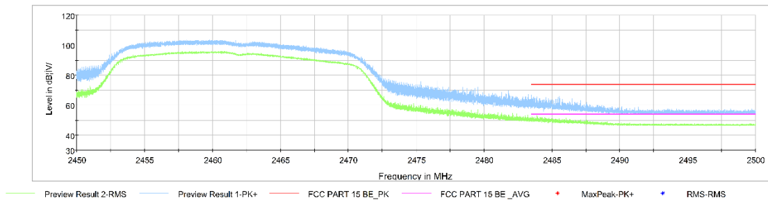
Fig.A.6.2.6 Transmitter Spurious Emission - Radiated (Power): 802.11n-HT20, ch11, 2.45 GHz - 2.50GHz
