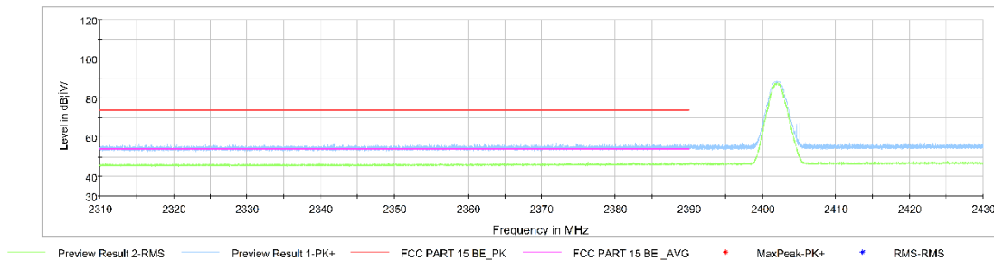
Fig.3. Frequency Band Edges: GFSK, 2402 MHz, Hopping Off, 2.31 GHz – 2.43GHz
