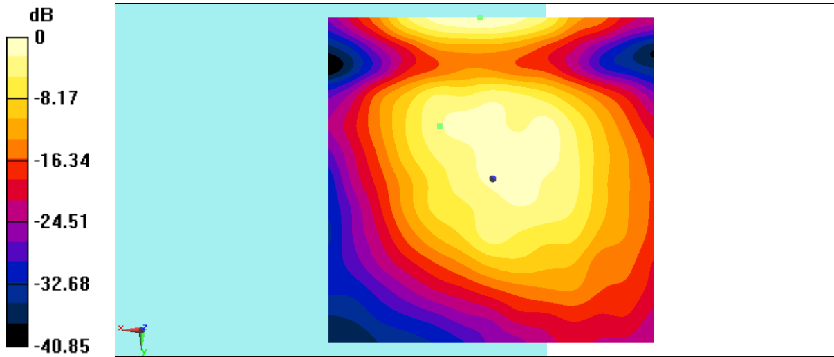
Fig B.1 T-Coil LTEB2
