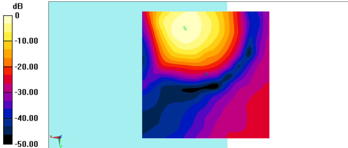
Fig B.2 T-Coil LTEB38
