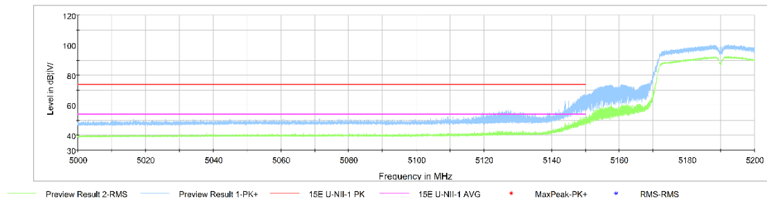
Fig.42 Band Edges (802.11n-HT40 Ch38, 5190MHz)
