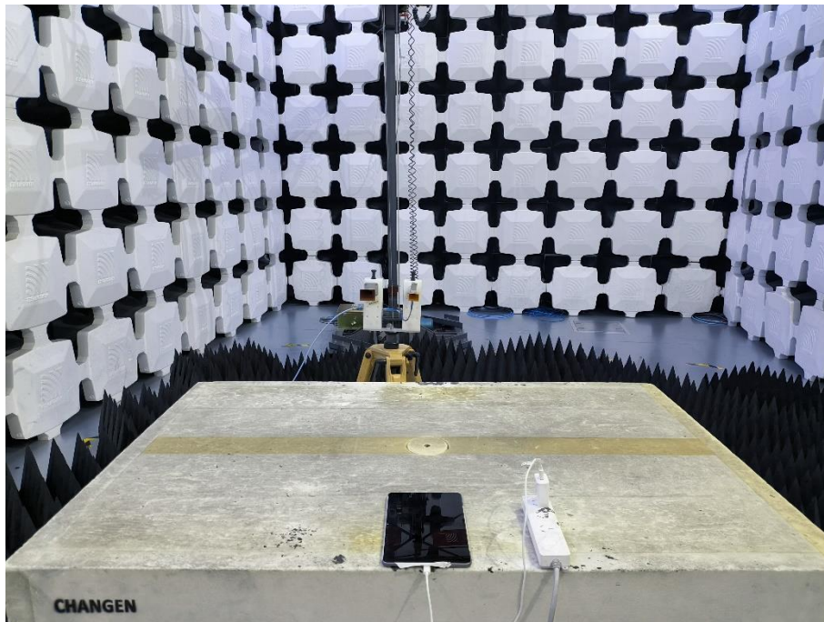
8. Radiated Emissions (Part 15B, Camera/Video Player, 26GHz-40GHz)
