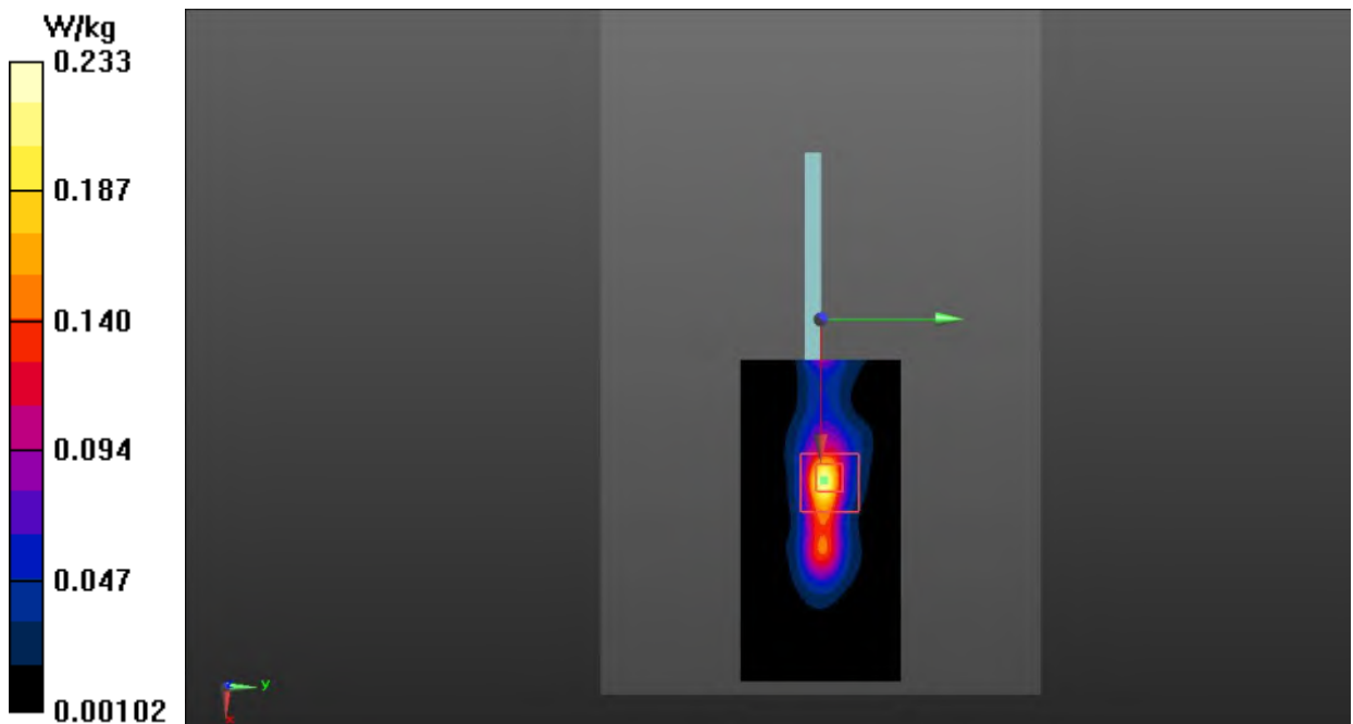
Fig.1 Bluetooth Body
