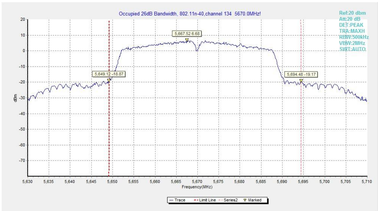
Fig. 12 Occupied 26dB Bandwidth (802.11n-HT40, 5670MHz)
