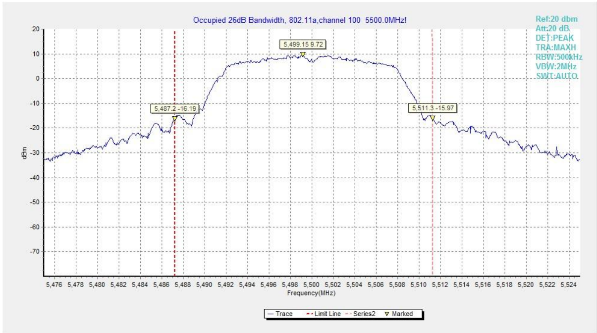
Fig. 5 Occupied 26dB Bandwidth (802.11a, 5500MHz)
