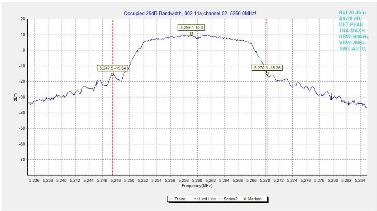
Fig. 3 Occupied 26dB Bandwidth (802.11a, 5260MHz)
