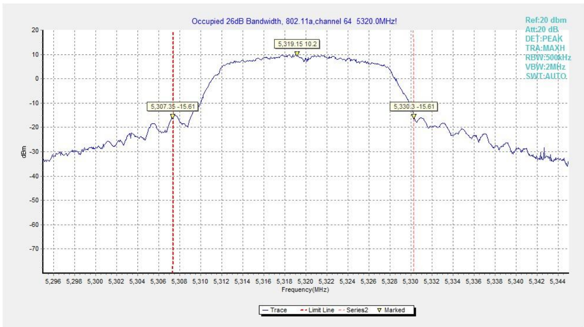
Fig. 4 Occupied 26dB Bandwidth (802.11a, 5320MHz)
