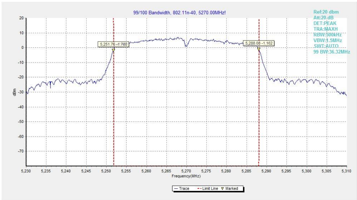
Fig. 31 99% Occupied Bandwidth (802.11n-HT40, 5270MHz)
