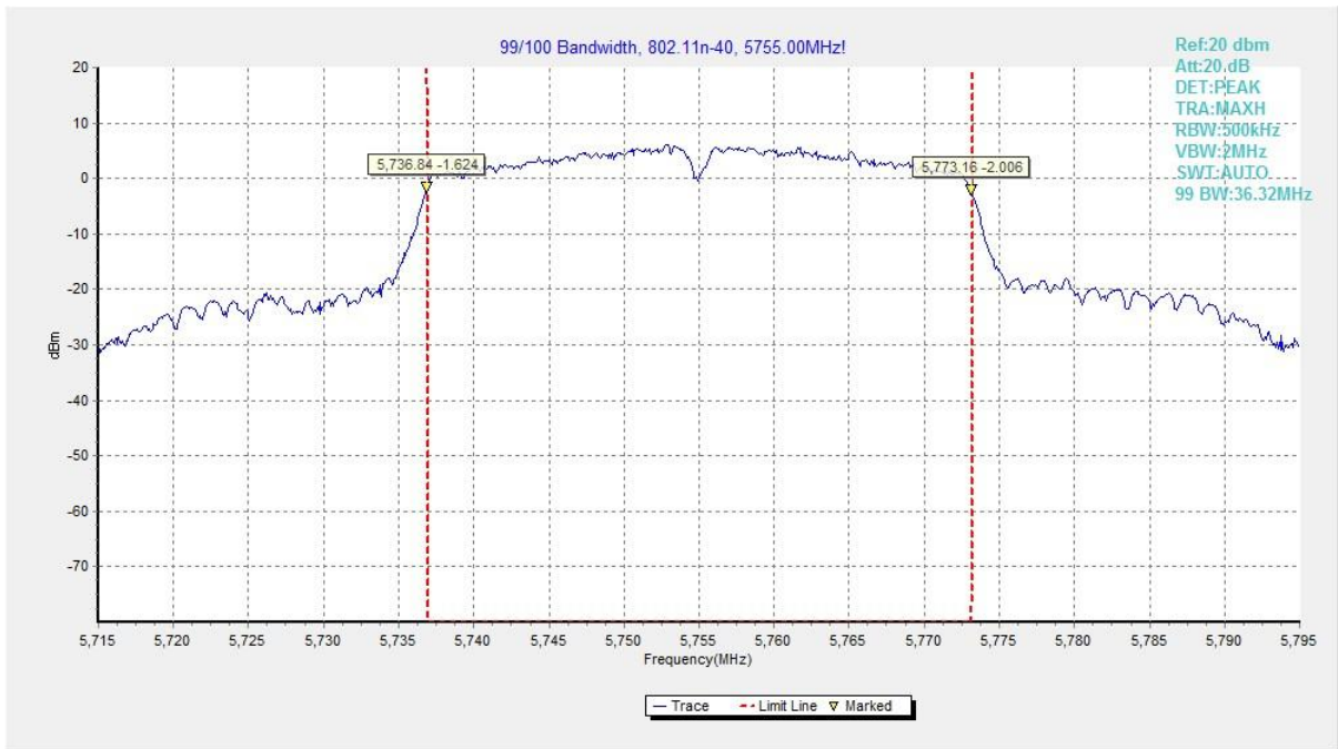
Fig. 35 99% Occupied Bandwidth (802.11n-HT40, 5755MHz)
