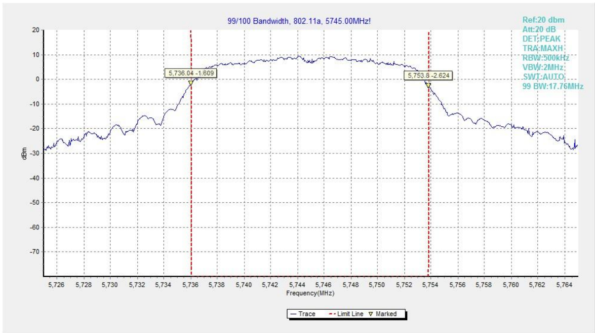
Fig. 27 99% Occupied Bandwidth (802.11a, 5745MHz)
