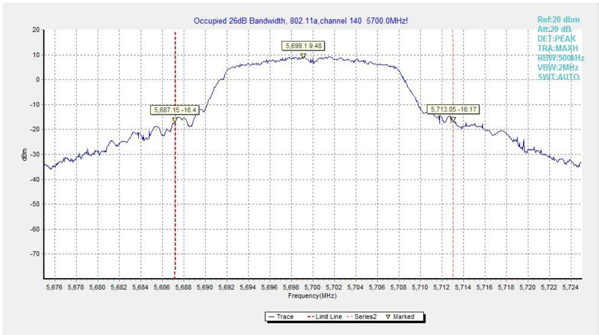
Fig. 6 Occupied 26dB Bandwidth (802.11a, 5700MHz)
