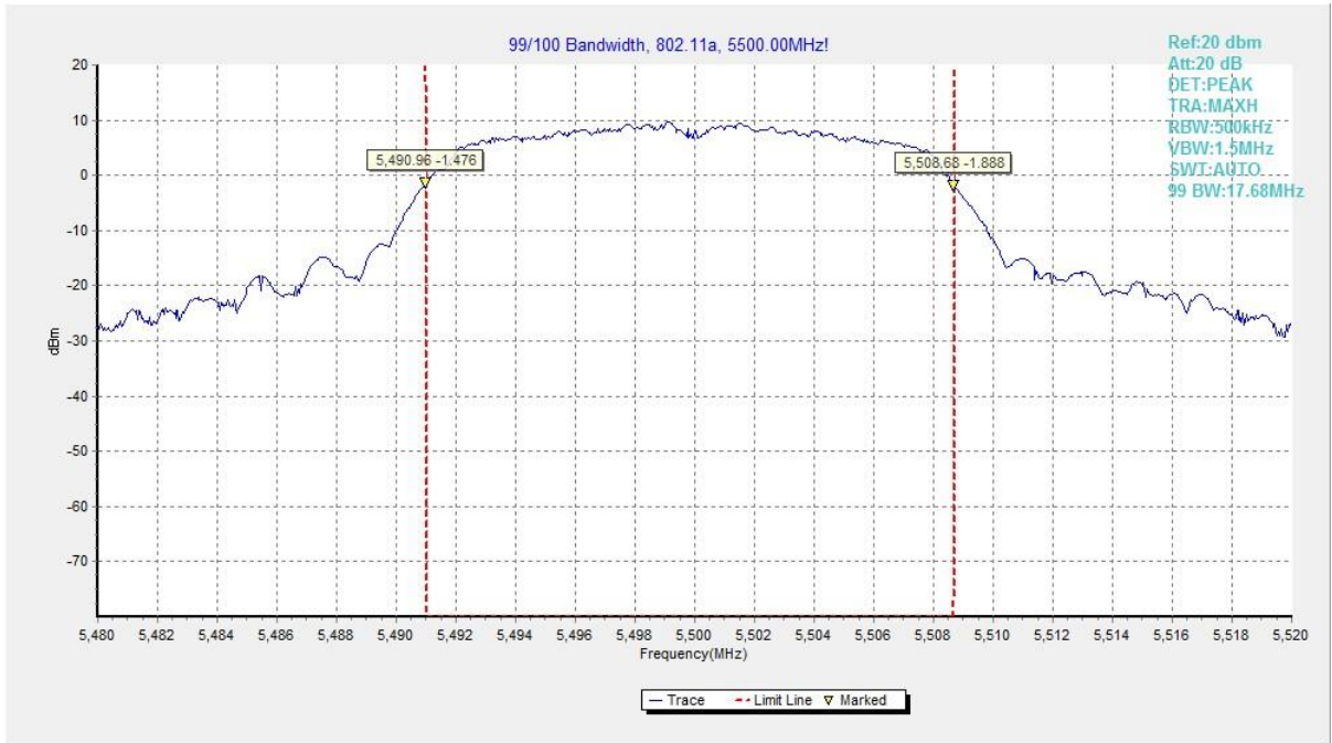
Fig. 25 99% Occupied Bandwidth (802.11a, 5500MHz)
