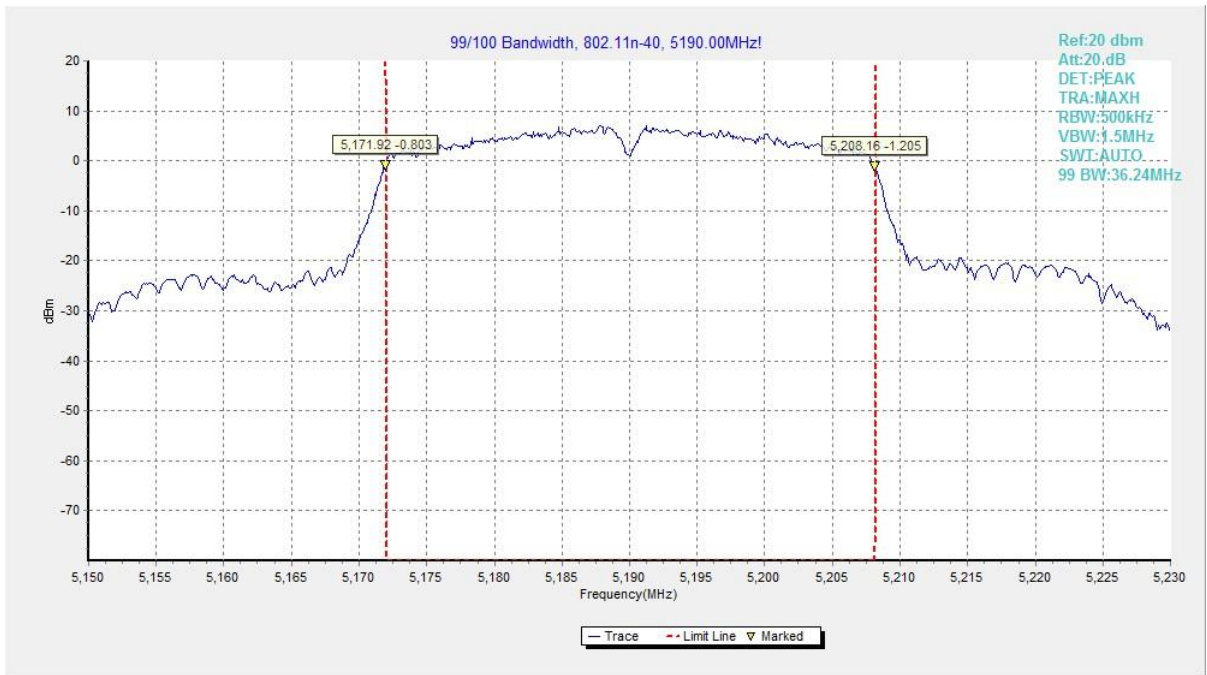
Fig. 29 99% Occupied Bandwidth (802.11n-HT40, 5190MHz)
