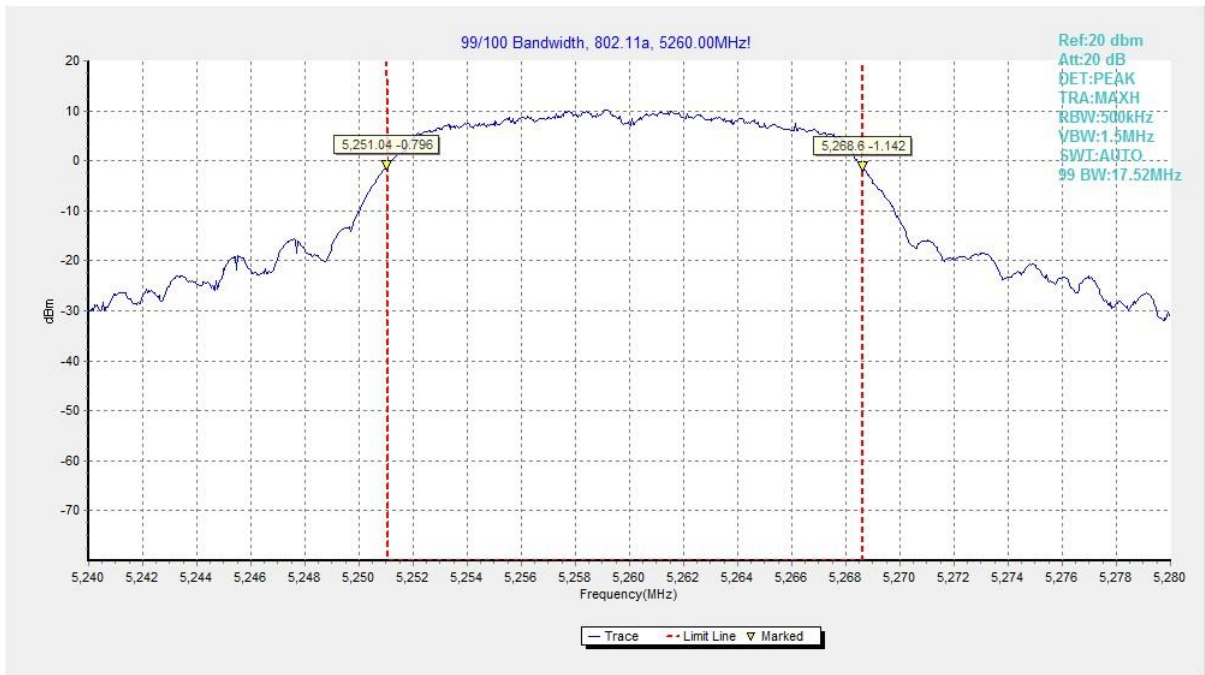
Fig. 23 99% Occupied Bandwidth (802.11a, 5260MHz)
