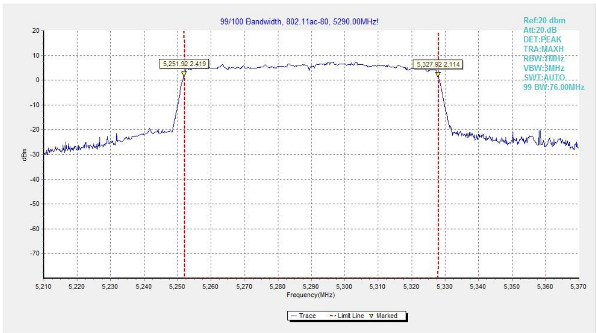
Fig. 38 99% Occupied Bandwidth (802. 11ac-VHT80, 5290MHz)
