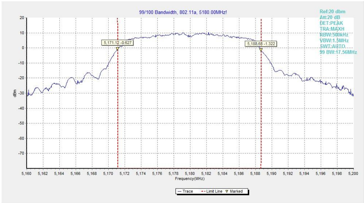
Fig. 21 99% Occupied Bandwidth (802.11a, 5180MHz)
