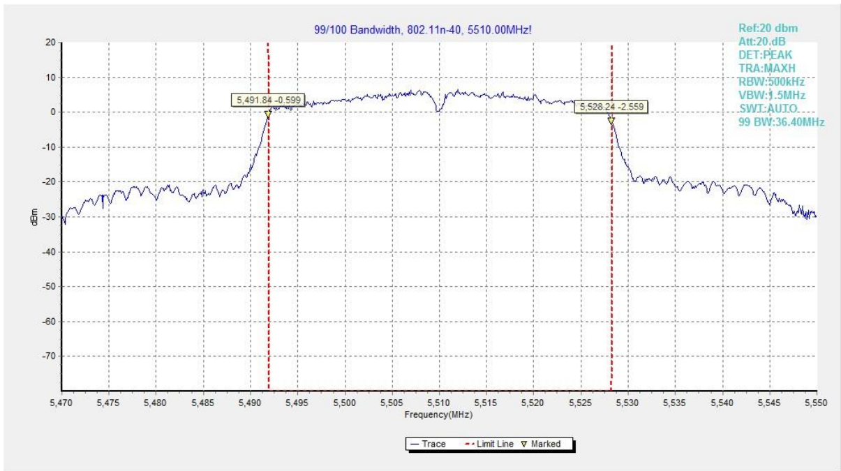
Fig. 33 99% Occupied Bandwidth (802.11n-HT40, 5510MHz)
