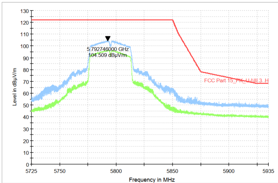
Fig. 52 Band Edges (802.11n-HT40, CH159 5795MHz)
