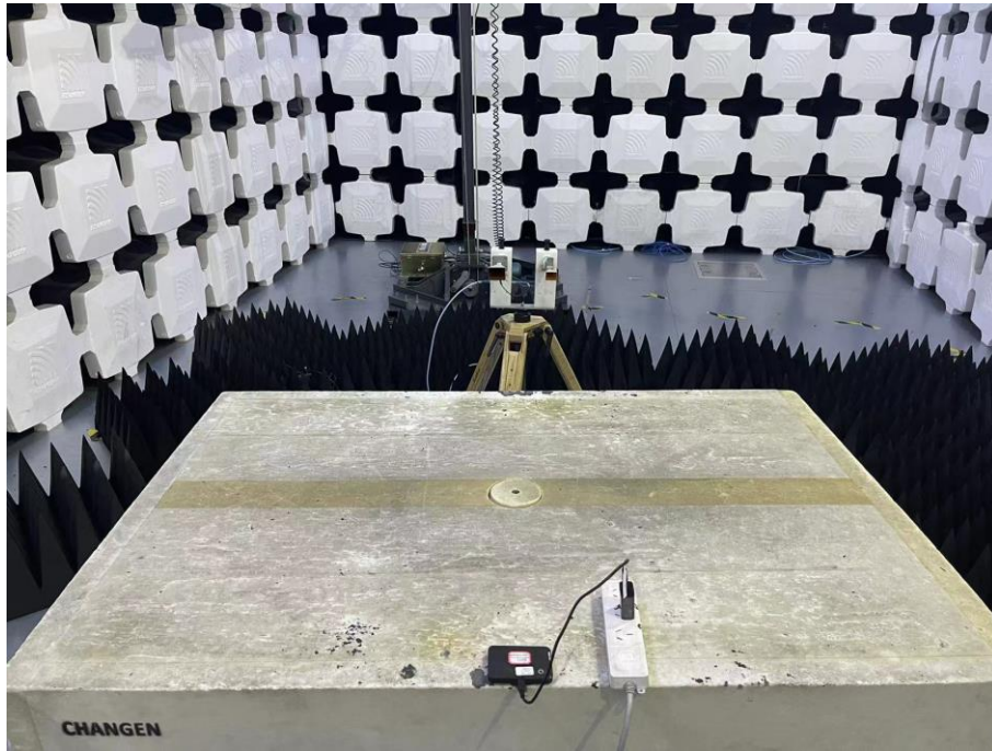
3. Radiated Emissions (Part 15B Charging, 18GHz-26.5GHz)
