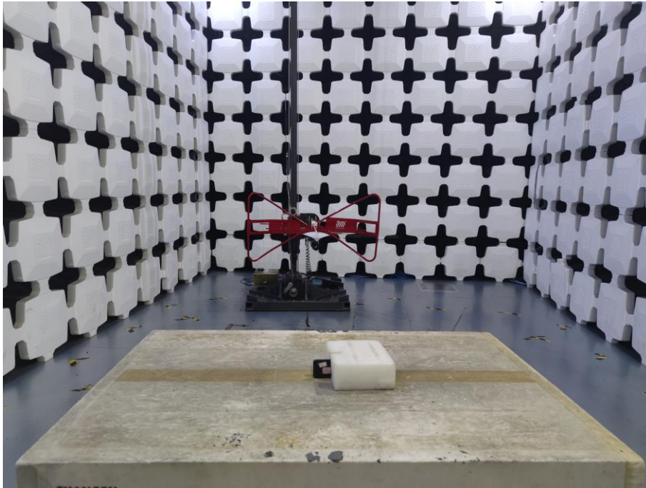
5. Radiated Emissions (Part 15C Wi-Fi, 30MHz-1GHz)
