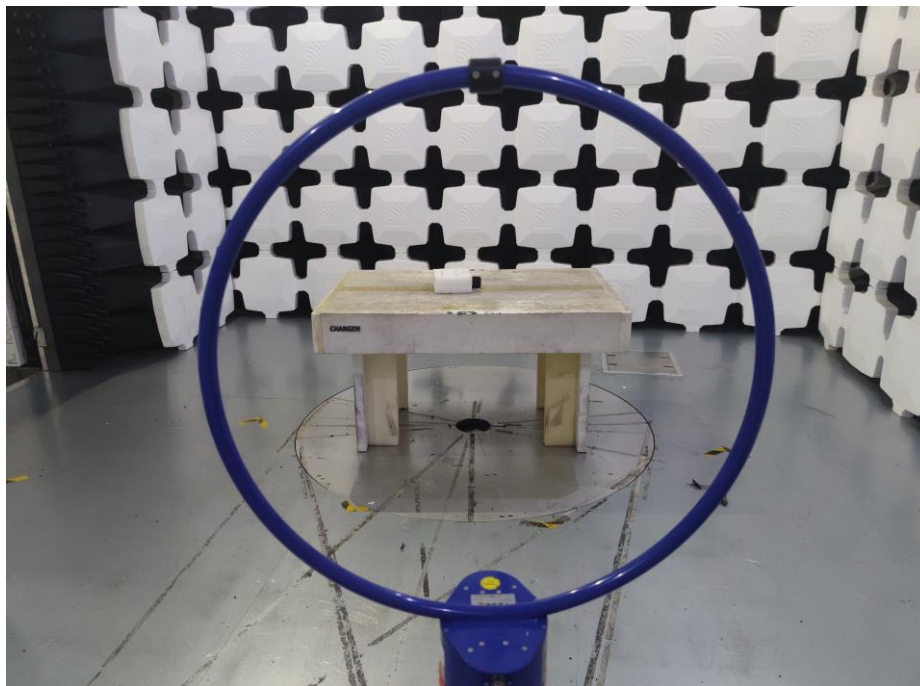
4. Radiated Emissions (Part 15C Wi-Fi, 9kHz-30MHz)
