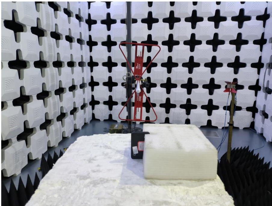
6. Radiated Emissions (Part 15C Wi-Fi, 1GHz -18GHz)
