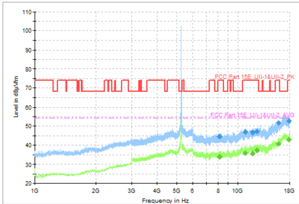
Fig. 68 Transmitter Spurious Emission (802.11a, CH52 5260MHz)
