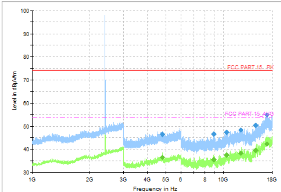
Fig. 43 Radiated Spurious Emission (8DPSK, Ch0, 1GHz ~ 18GHz)
