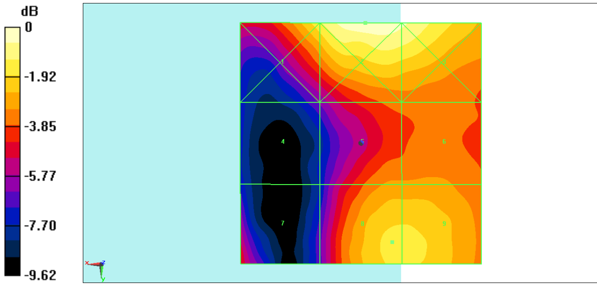
Fig B.3 HAC RF E-Field LTE Band38
