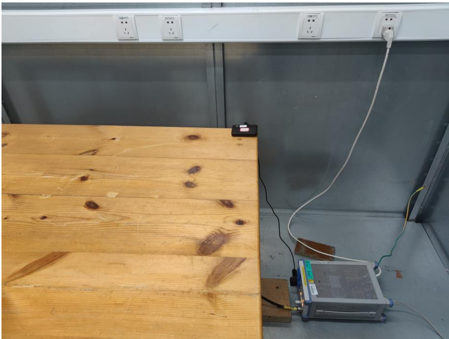
12. Conducted Emission (Part 15B, Charging)
