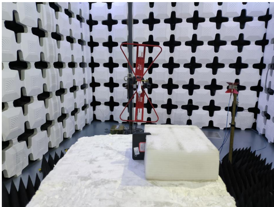
10. Radiated Emissions (Part 27,1GHz-18GHz)
