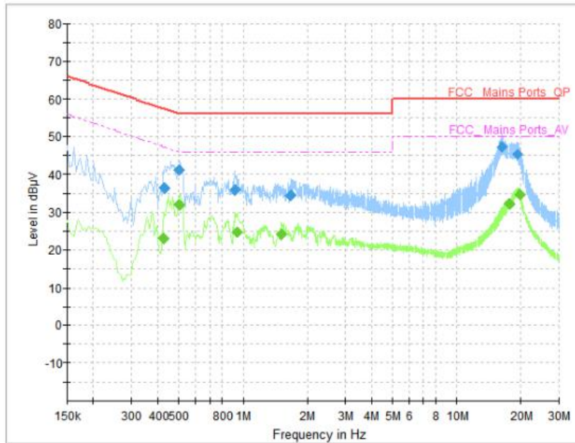
Fig. 73 AC Power line Conducted Emission (Idle)
