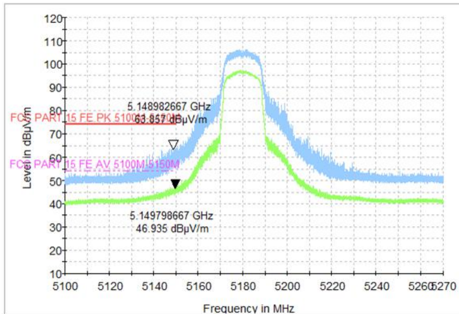
Fig. 37 Band Edges (802.11a, CH36 5180MHz)
