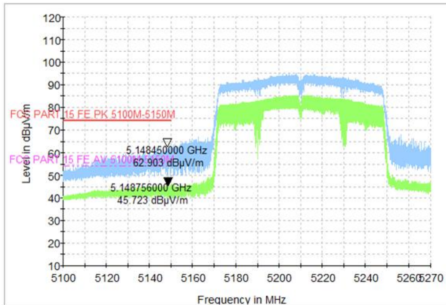
Fig. 45 Band Edges (802.11ac-VHT80, CH42 5210MHz)
