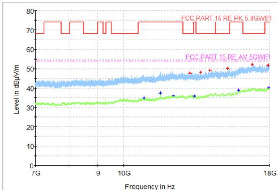
Fig. 62 Transmitter Spurious Emission (802.11ac-VHT40, CH159 5795MHz)
