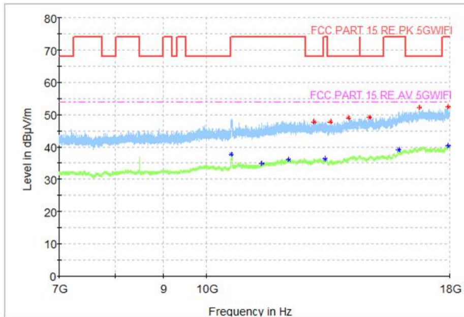
Fig. 60 Transmitter Spurious Emission (802. 11ac-VHT40, CH62 5310MHz)
