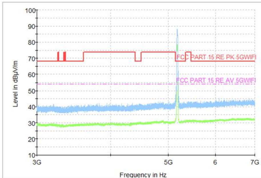
Fig. 68 Transmitter Spurious Emission (All channel, 3GHz~7GHz)
