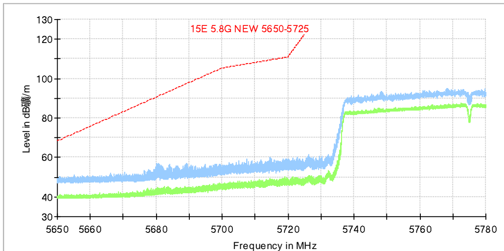
Fig. 20 Band Edges (802.11ac-HT80 Ch155, 5775MHz)
