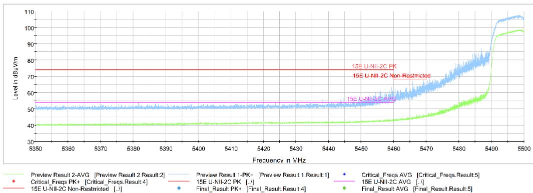
Fig.48 Band Edges (802.11ac-HT20 Ch100, 5500MHz)
