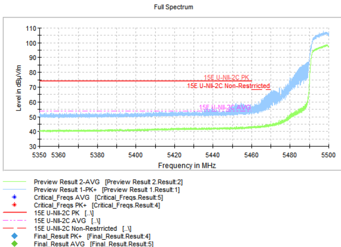
Fig.40 Band Edges (802.11n-HT20 Ch100, 5500MHz)
