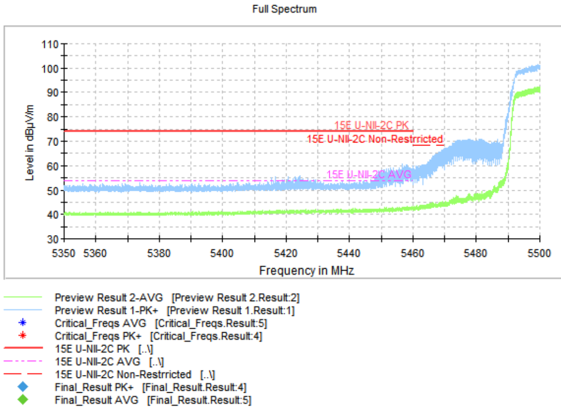
Fig.44 Band Edges (802.11n-HT40 Ch102, 5510MHz)
