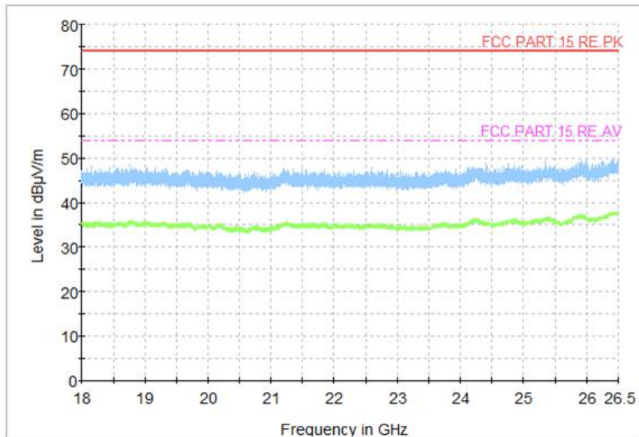
Fig.25 Radiated Spurious Emission (Ch19, 18 GHz - 26.5 GHz), 1M
