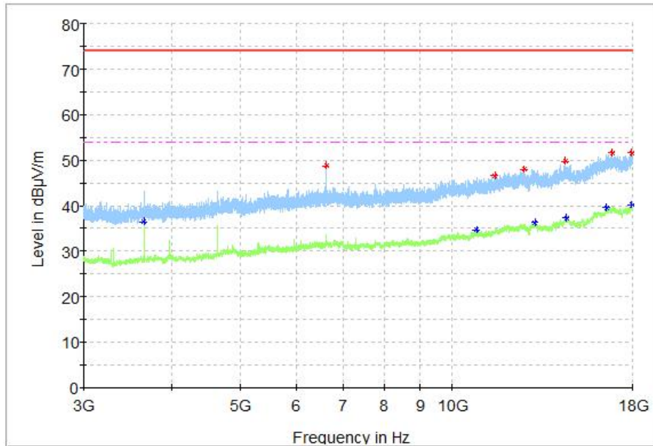
Fig.24 Radiated Spurious Emission (Ch19, 3 GHz - 18 GHz), 1M
