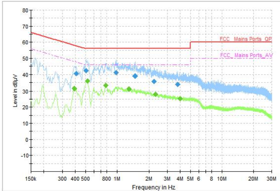
Fig.29 AC Power line Conducted Emission (Traffic, AE2, 120V), 1M
