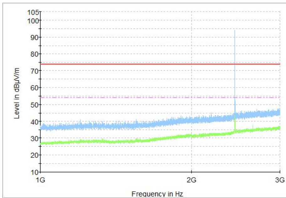
Fig.23 Radiated Spurious Emission (Ch19, 1 GHz - 3 GHz), 1M
