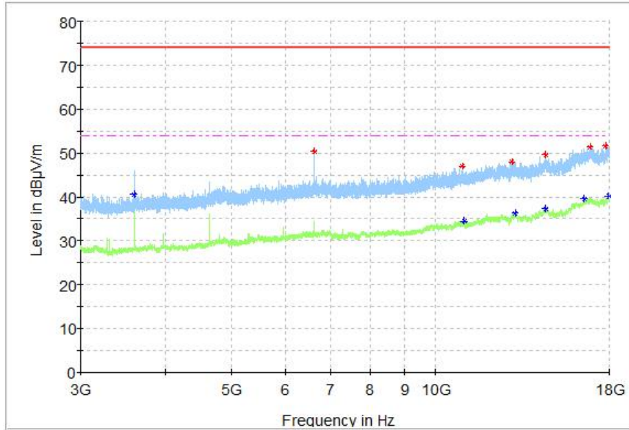
Fig.20 Radiated Spurious Emission (Ch0, 3 GHz - 18 GHz), 1M
