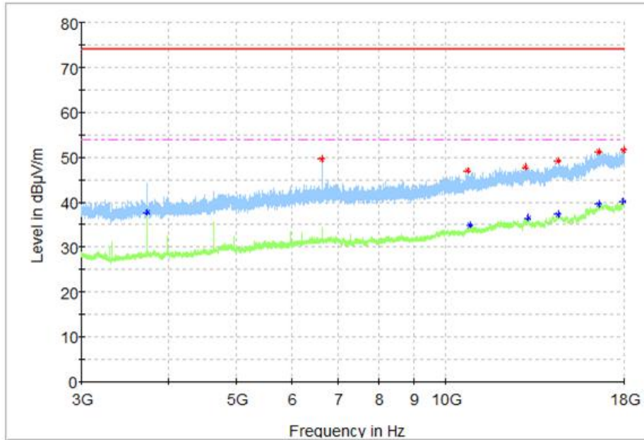
Fig.26 Radiated Spurious Emission (Ch39, 3 GHz - 18 GHz), 1M
