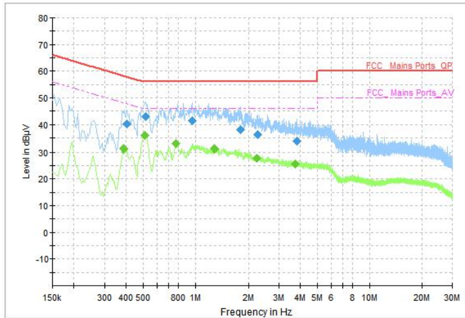
Fig.30 AC Power line Conducted Emission (Idle, AE2, 120V), 1M
