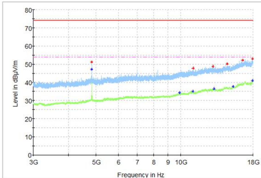
Fig.50 Radiated Spurious Emission (802.11g, CH1, 3GHz-18GHz)
