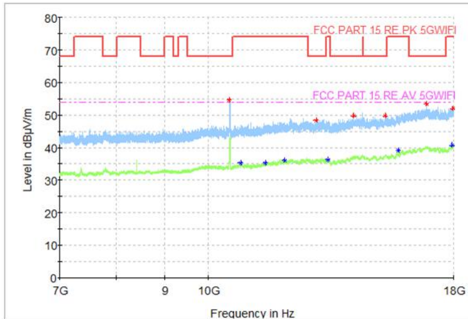
Fig. 51 Transmitter Spurious Emission (802.11a, CH52 5260MHz)
