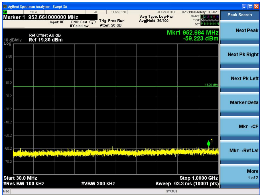
Channel 9400, 30MHz~1GHz
