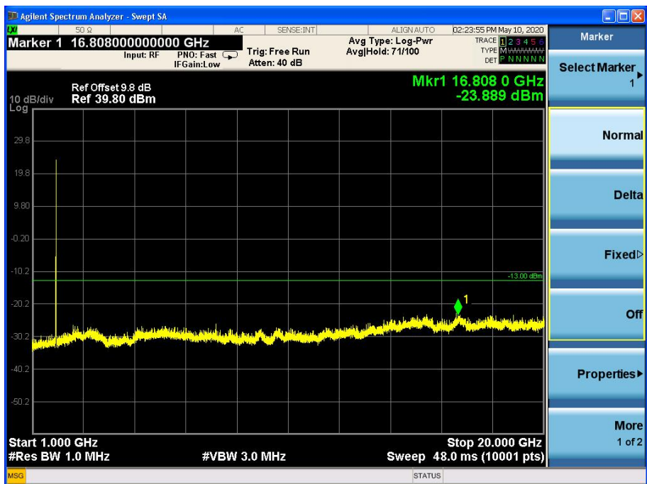
Channel 9400, 1GHz~20GHz
