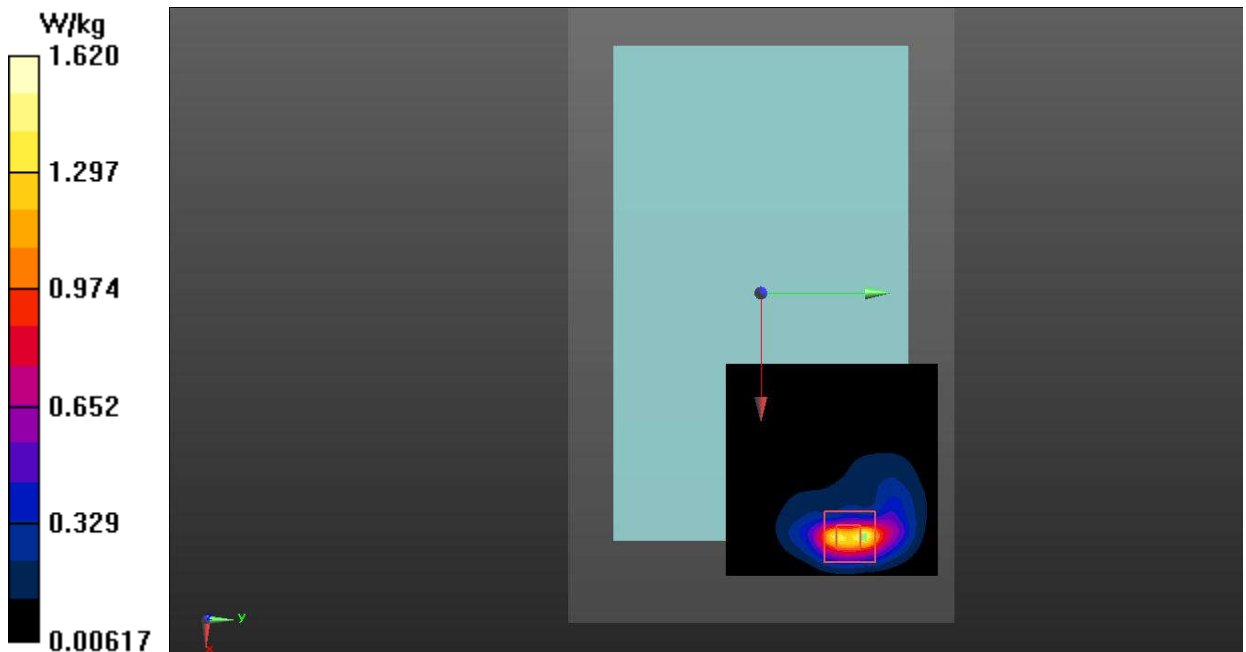
Fig.2 GSM 1900 Body
