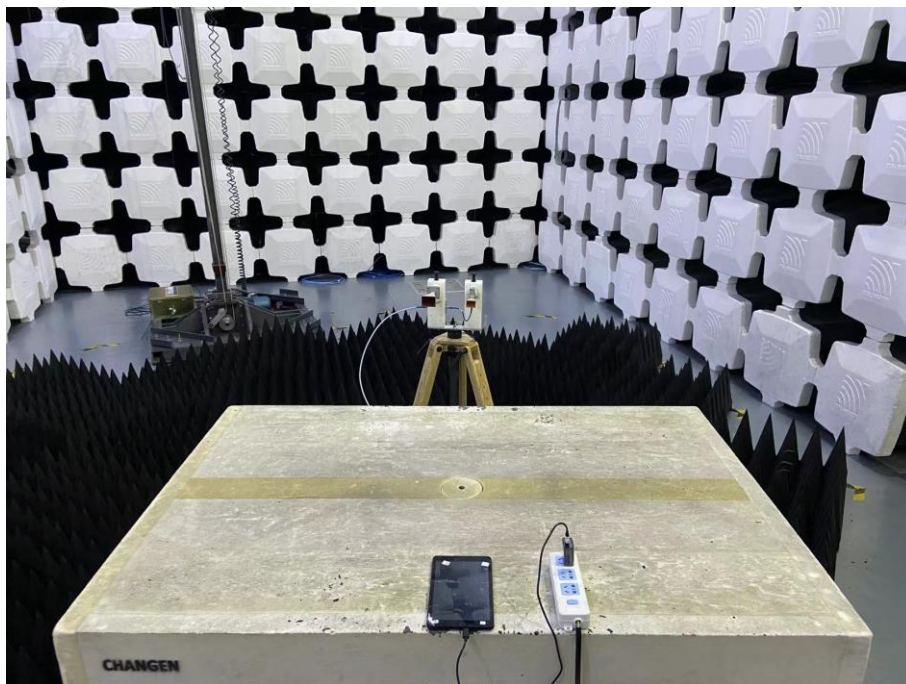
8. Radiated Emissions (Part 15B, Camera/Video Player /GSM receiver/WCDMA receiver /LTE receiver, 26GHz-40GHz)
