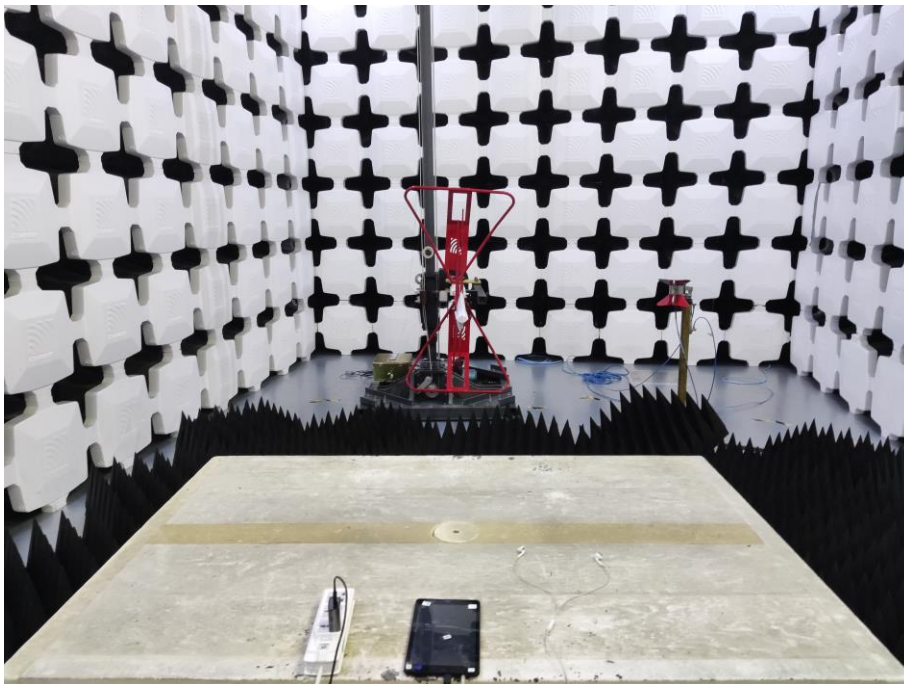
10. Radiated Emissions (Part 15B, FM receive, 1GHz-18GHz)
