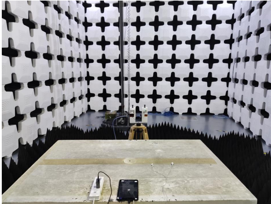
11. Radiated Emissions (Part 15B, FM receive, 18GHz-26.5GHz)
