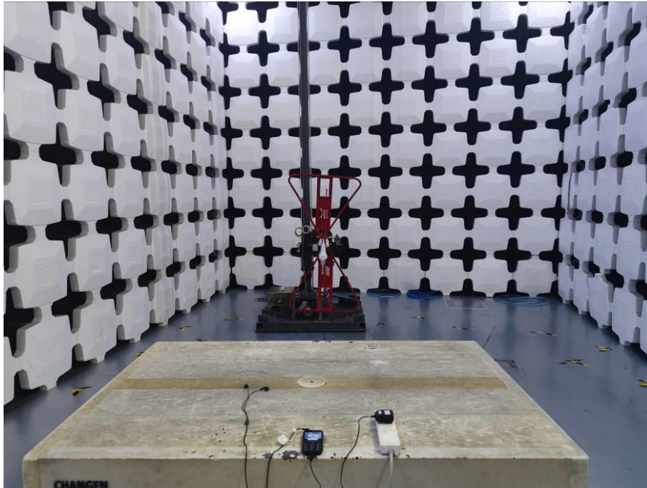
3. Radiated Emissions (Part 15B, Camera/GSM receiver/FM receiver,30MHz-1GHz)
