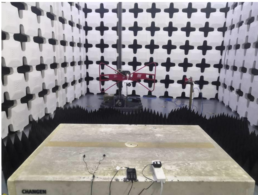
4. Radiated Emissions (Part 15B, Camera/GSM receiver/FM receiver,1GHz-18GHz)
